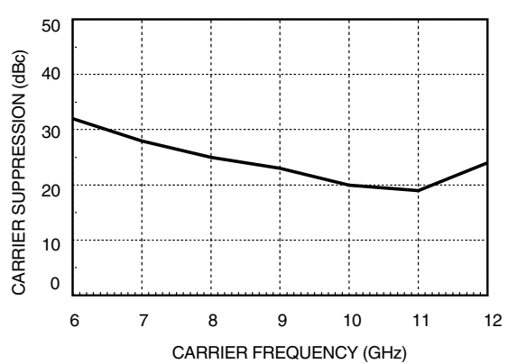
Carrier Suppression *
