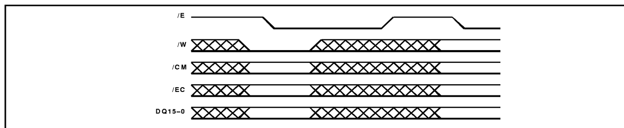
Figure 4: Write Cycle
