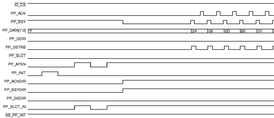
Figure 12. Parallel Port—IBM DMA Read
