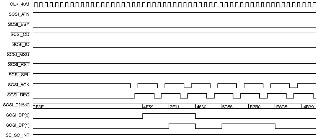
Figure 7. SCSI Synchronous Read
