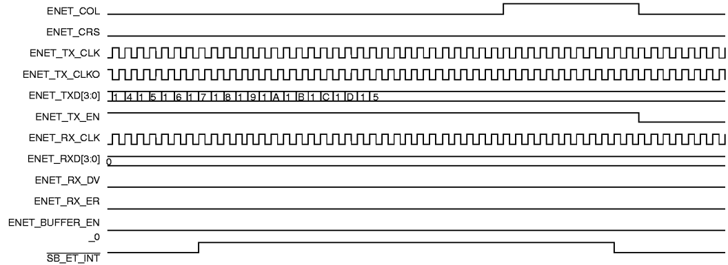
Figure 10. Ethernet-Collision Detected
