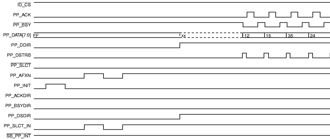
Figure 13. Parallel Port-IBM DMA Write
