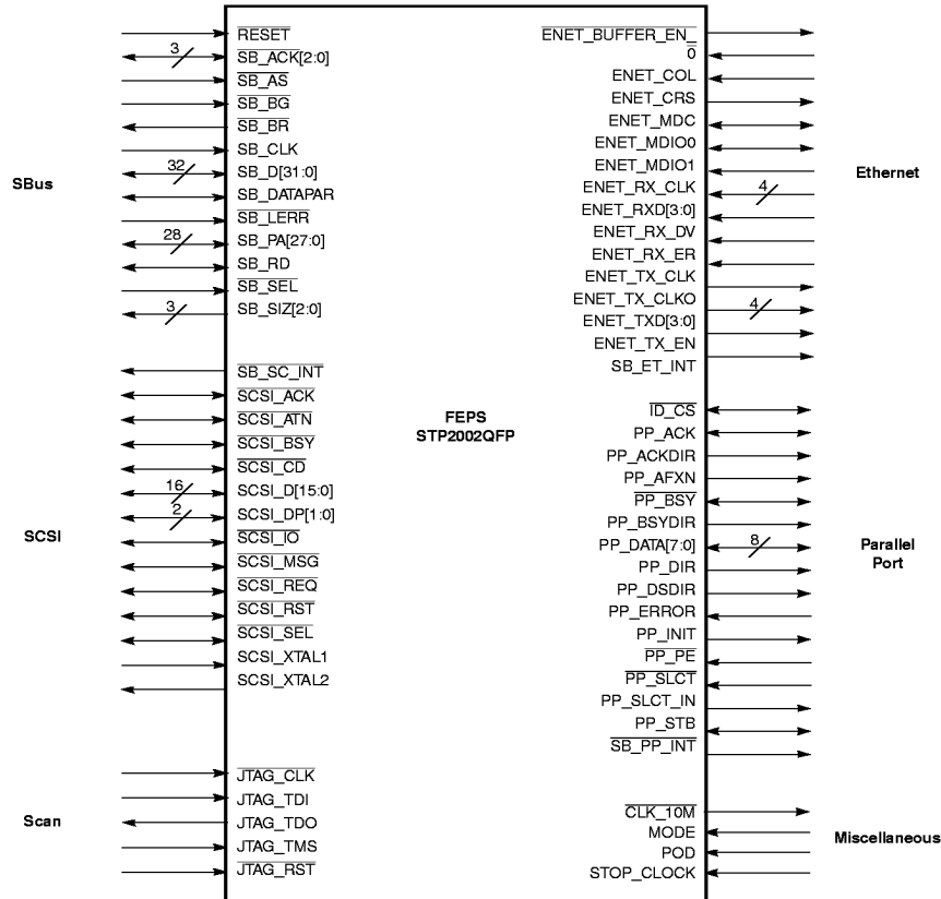
Figure 1. External Interfaces
