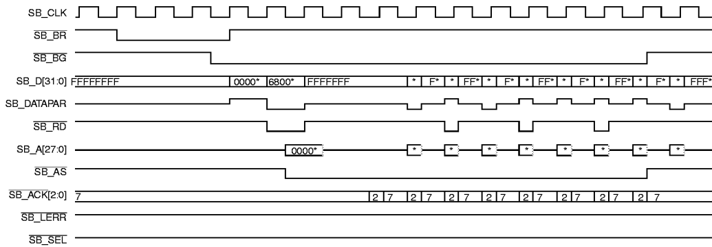
Figure 4. SBus Write
