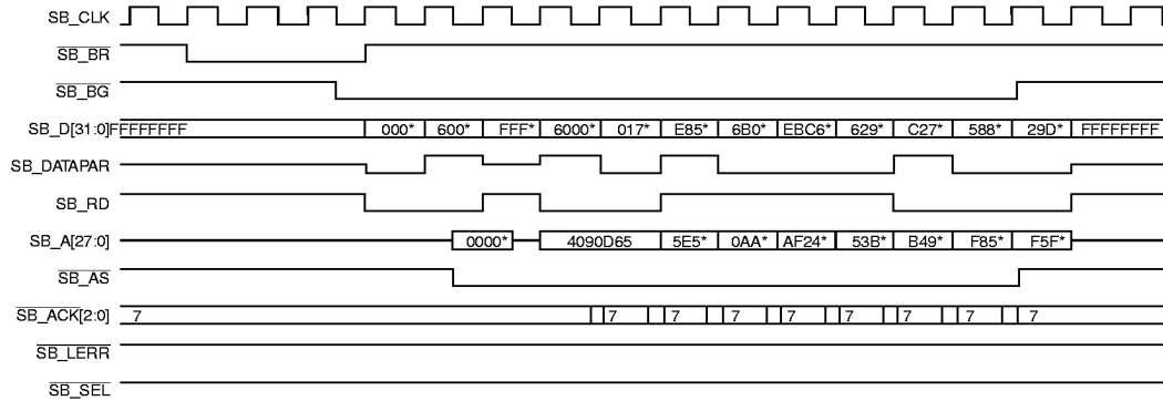
Figure 3. SBus Read
