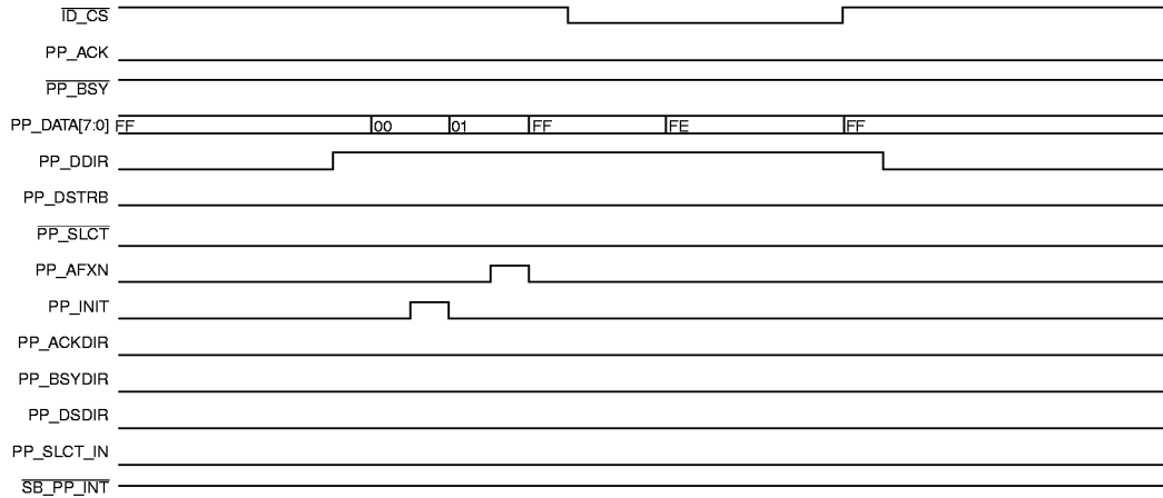
Figure 11. Parallel Port—EPROM Read
