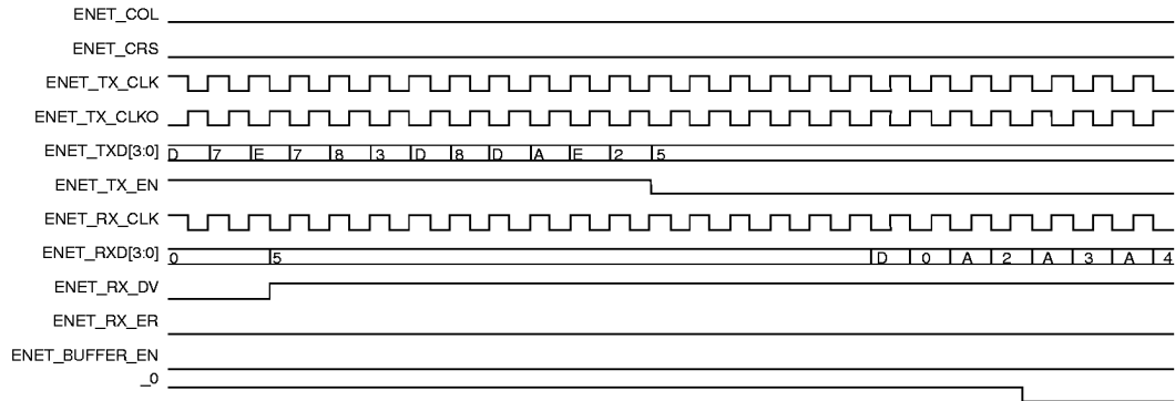
Figure 9. Ethernet Tx and Rx
