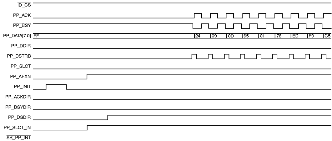
Figure 14. Parallel Port-Xerox DMA Read
