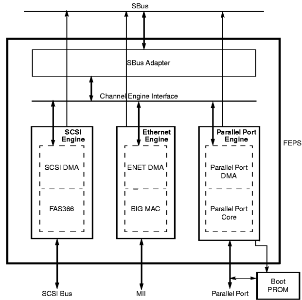
Figure 2. FEPS Functional Block Diagram
