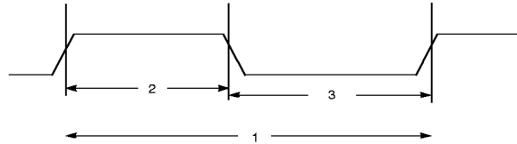
Figure 15. SCSI Clock
