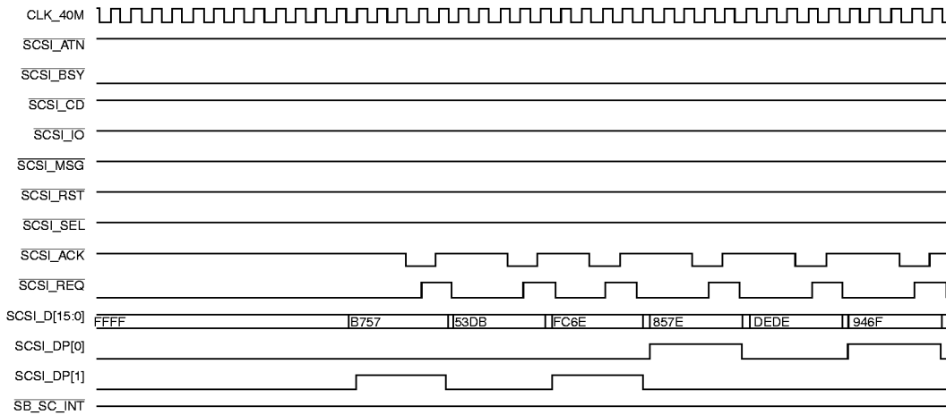
Figure 6. SCSI Asynchronous Write
