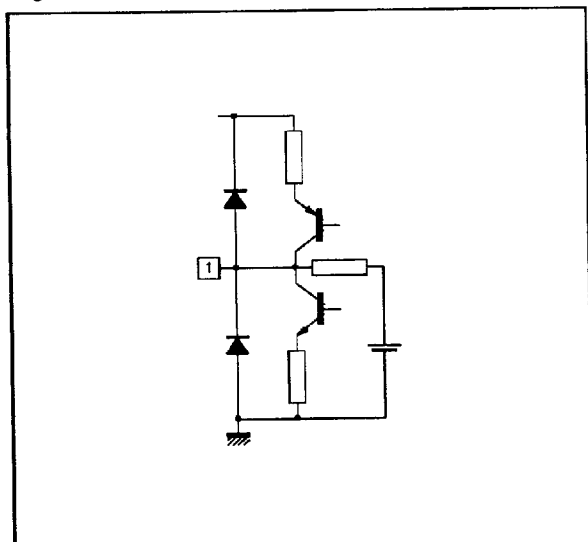
Figure 3 : CVBS Output
