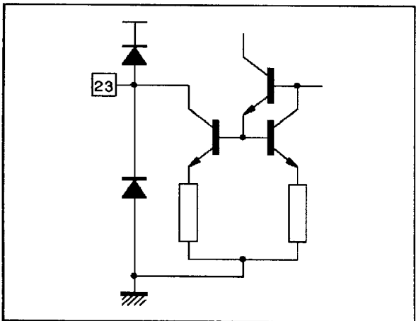
Figure 19 : Tuner AGC Output
