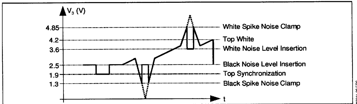
Figure 25 : Black and White Noise Inverter
