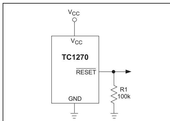
FIGURE 4-2: Ensuring \overline{\text{RESET}} Valid to V_{CC} = 0\text{V} .
