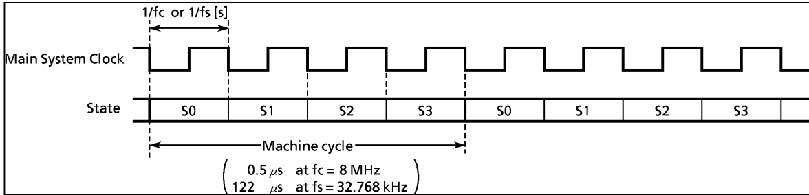
Figure 1-13. Machine Cycle
