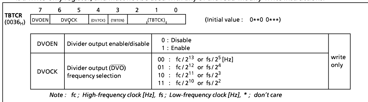
Figure 2-14. Divider Output Control Register
