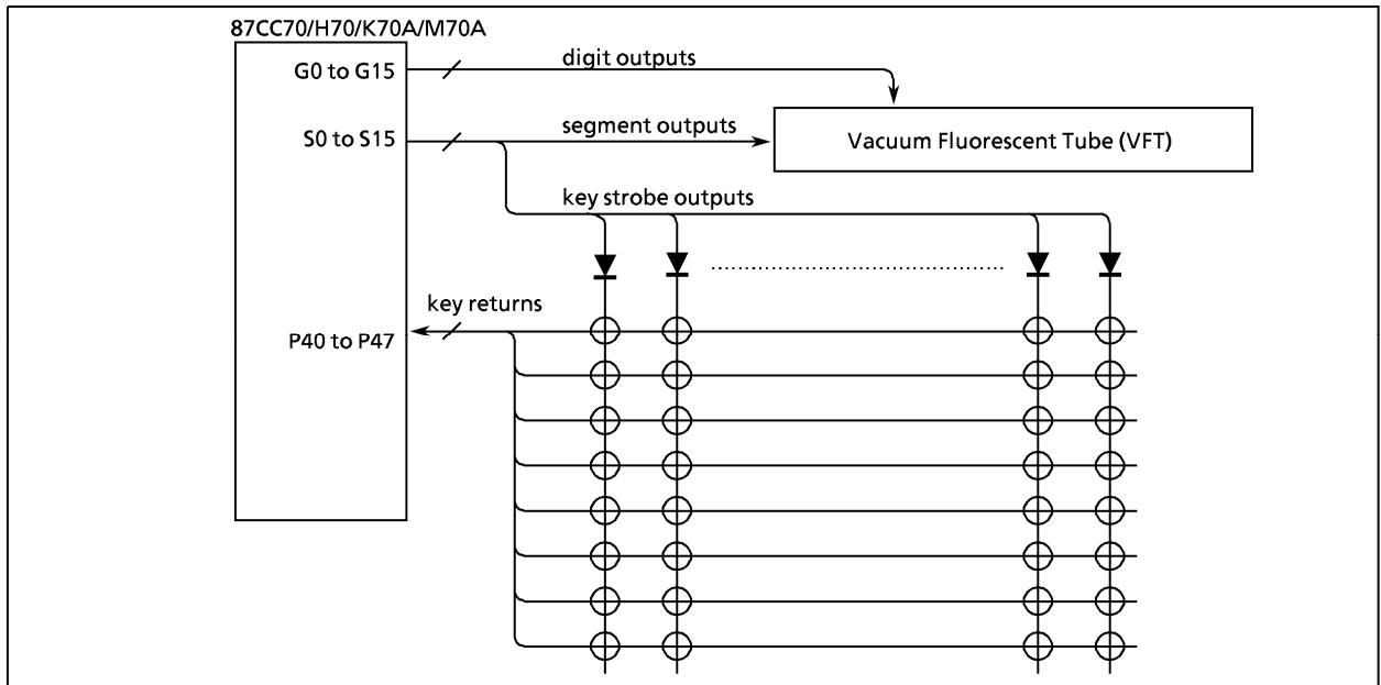
Figure 2-48. Key Matrix Example
