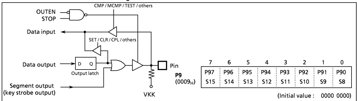
Figure 2-11. Port P9
