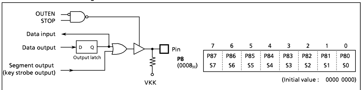
Figure 2-10. Port P8
