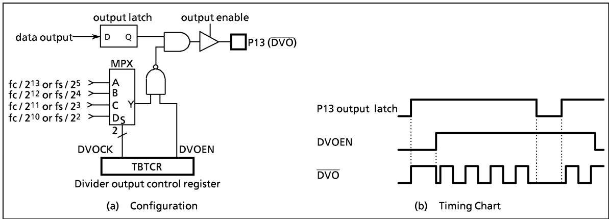
Figure 2-15. Divider Output
