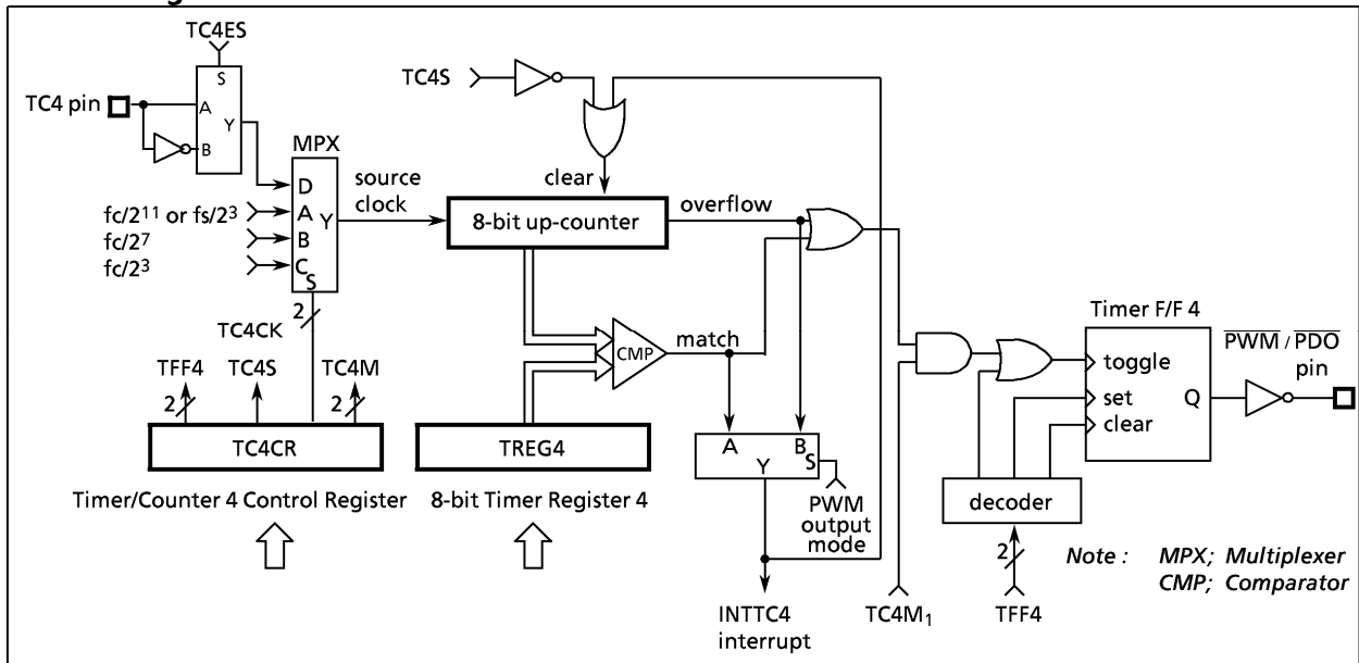
Figure 2-25. Timer/Counter 4
