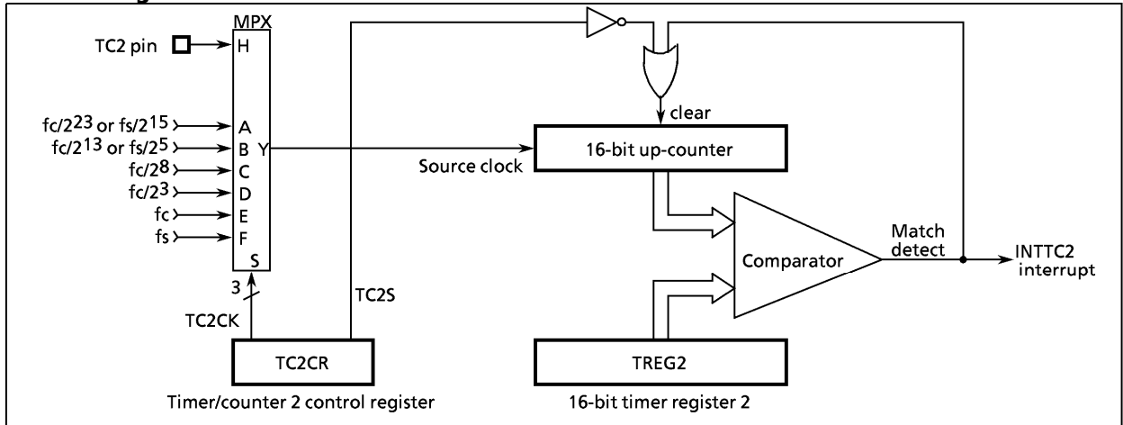
Figure 2-20. Timer/Counter 2
