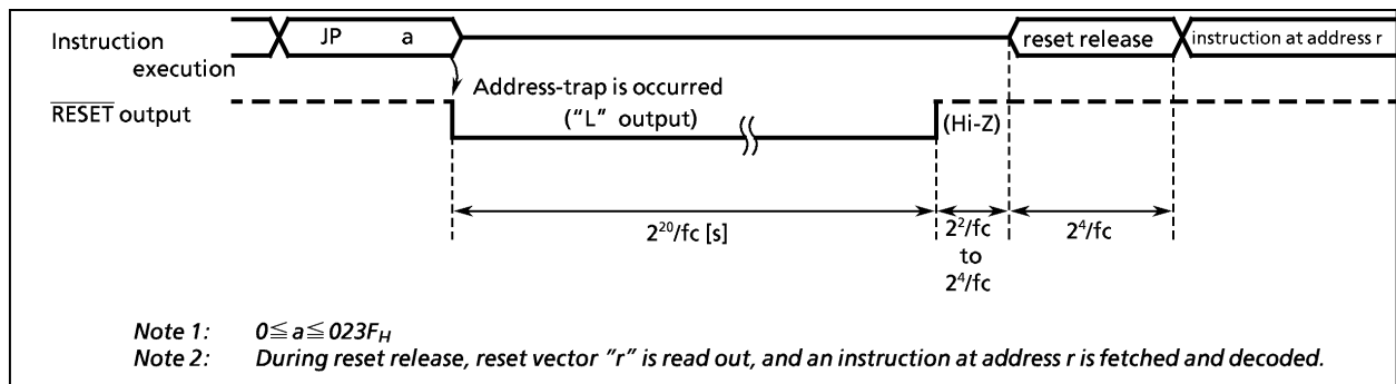
Figure 1-31. Address-Trap-Reset
