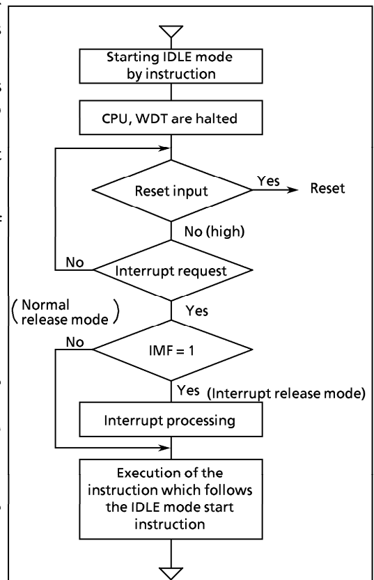
Figure 1-19. IDLE Mode
