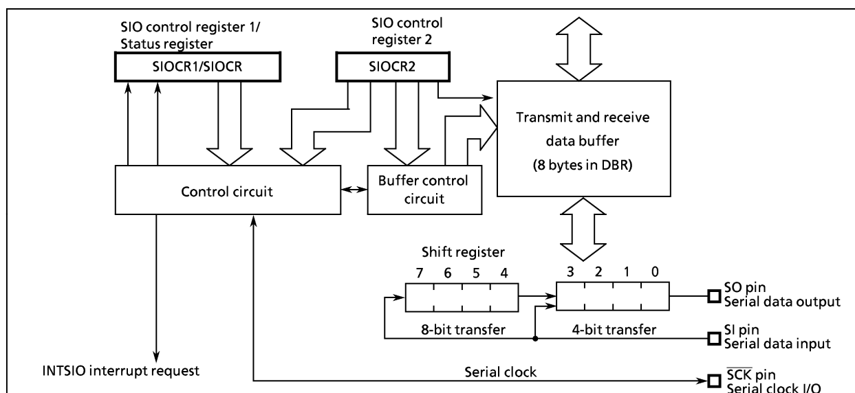
Figure 2-29. Serial Interface
