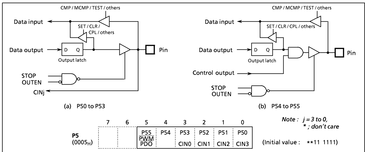
Figure 2-8. P5 Port
