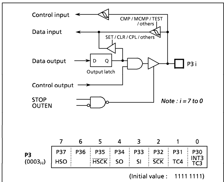
Figure 2-6. Port P3
