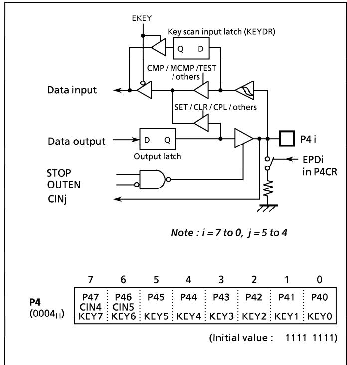
Figure 2-7. Port P4
