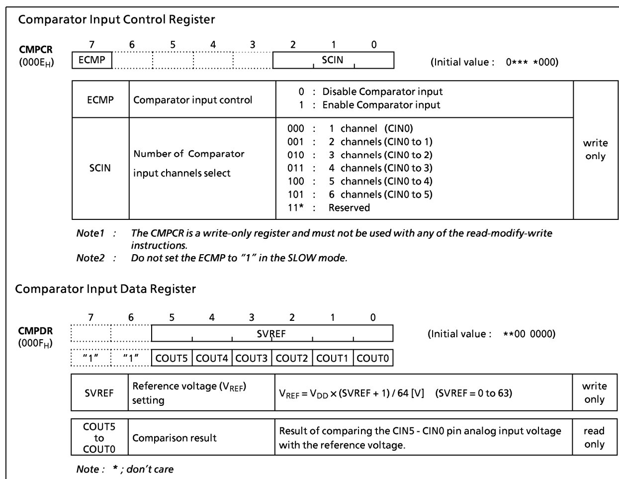
Figure 2-42. Comparator Input Control Register and Data Register
