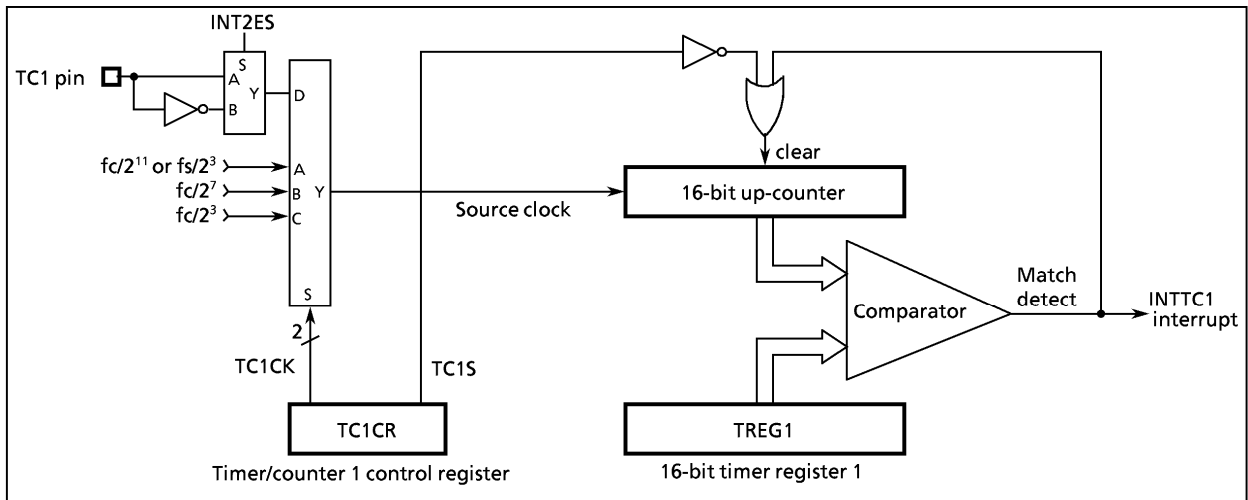
Figure 2-16. Timer/Counter 1
