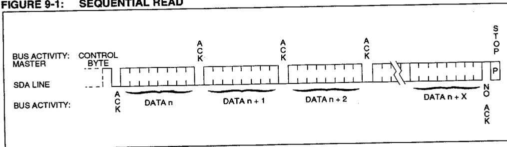
FIGURE 9-1: SEQUENTIAL READ
