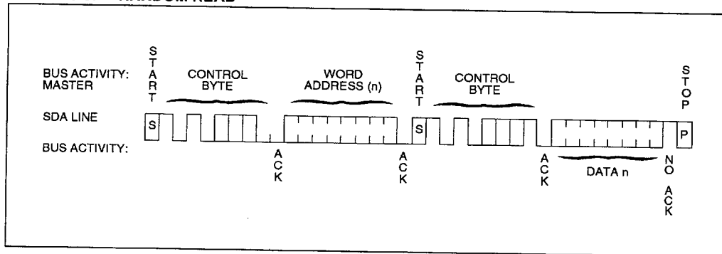
FIGURE 8-3: RANDOM READ
