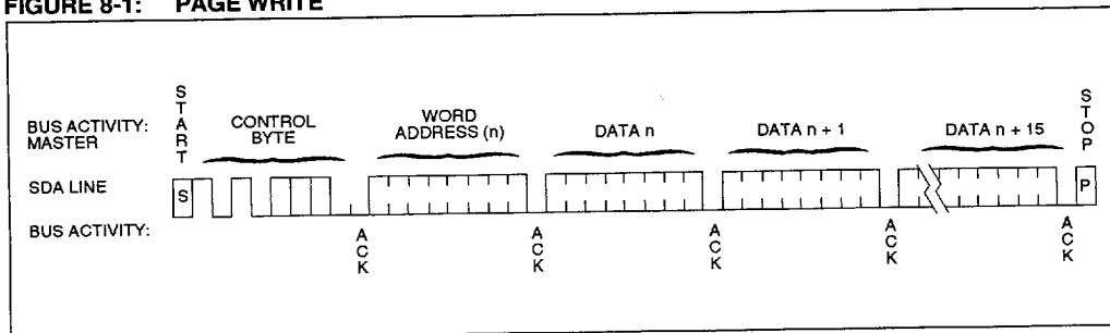
FIGURE 8-1: PAGE WRITE
