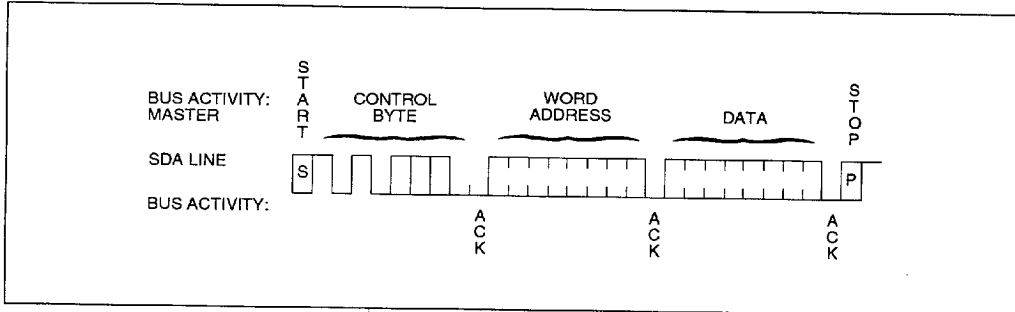
FIGURE 5-1: BYTE WRITE
