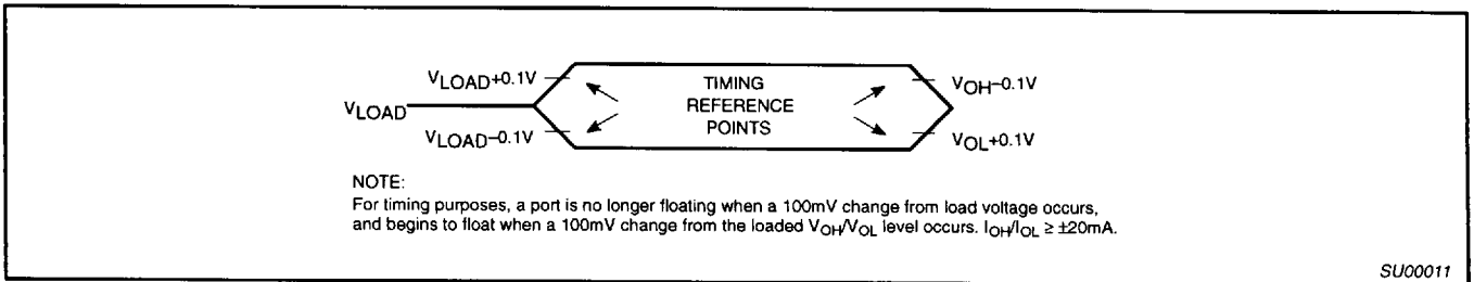
Figure 11. Float Waveform
