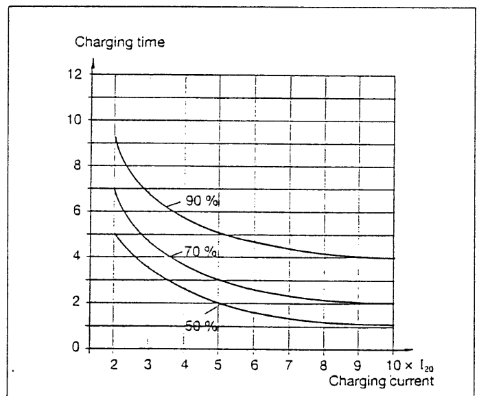
Fig. 5 shows the recharge time subject to the initial charging current to 50%, 70% and 90% of capacity. The graph is based on 2.4 Volt/cell charging voltage.
