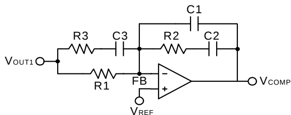
Figure 9. Compensation Network
