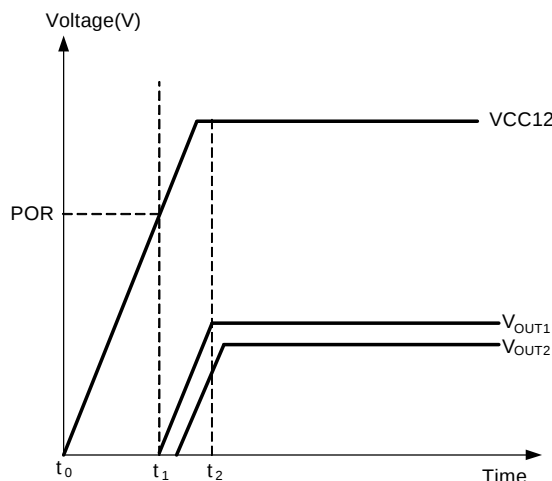
Figure 1. Soft-Start Interval
