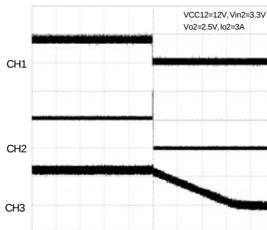
UVP_Linear Regulator ( FBL < 50\% V_{REF} )
