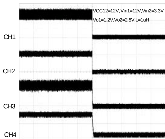
Shutdown(FS_DIS=GND)
