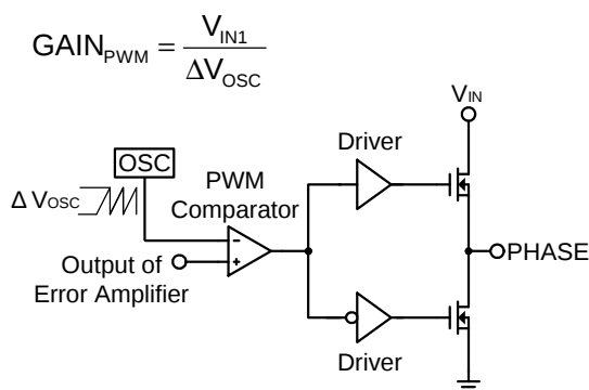
Figure 8. The PWM Modulator
