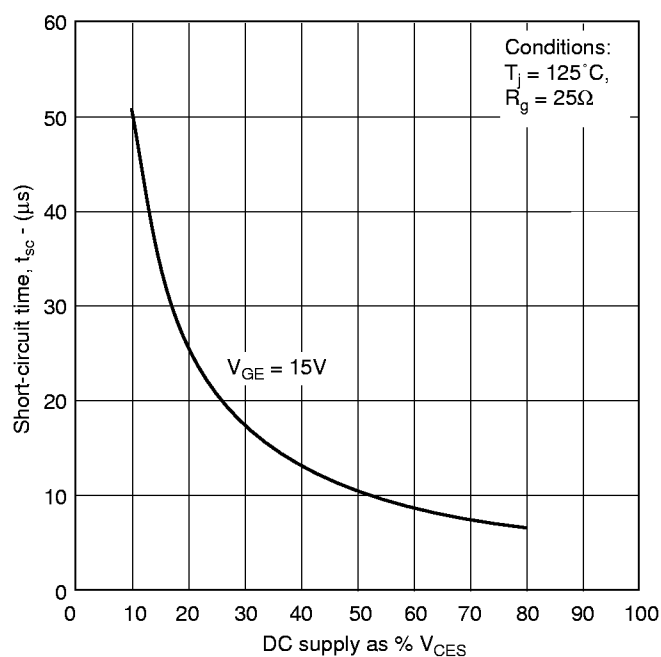
Fig.18 Short circuit withstand
