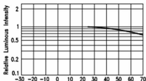
Fig.5 Luminous Intensity vs. Ambient Temperature
