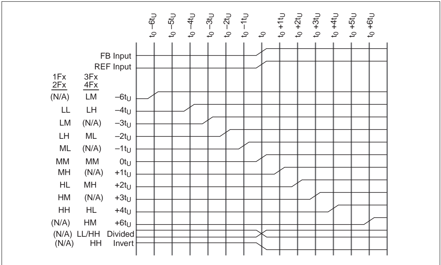
Figure 1. Typical Outputs with FB Connected to a Zero-Skew Output (4)
