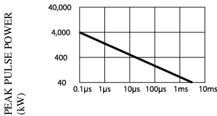
PULSE WIDTH
