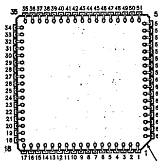
Figure 2. 80C186 Pinout Diagrams
