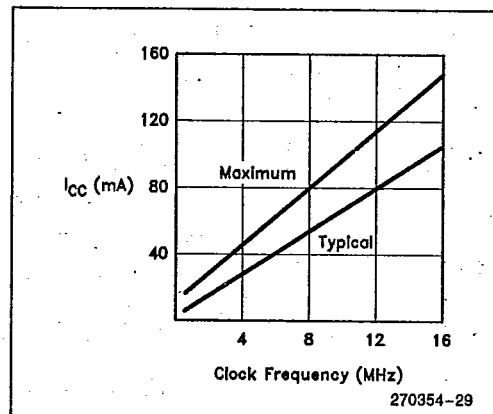
Figure 46. I_{CC} vs Frequency
