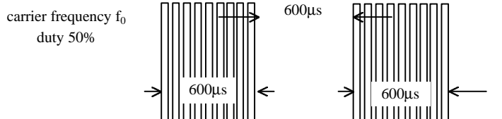
Fig 1. Burst Wave
