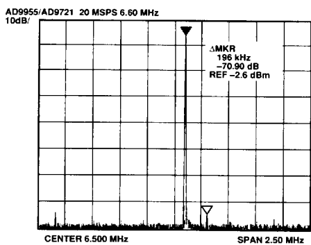
Figure 12. AD9955/AD9721 Output Spectrum
