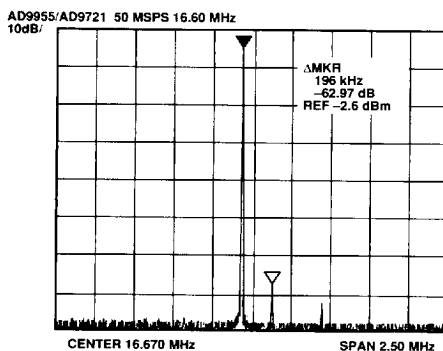
Figure 15. AD9955/AD9721 Output Spectrum
