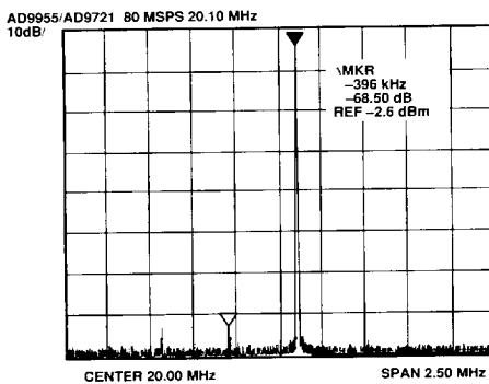
Figure 17. AD9955/AD9721 Output Spectrum
