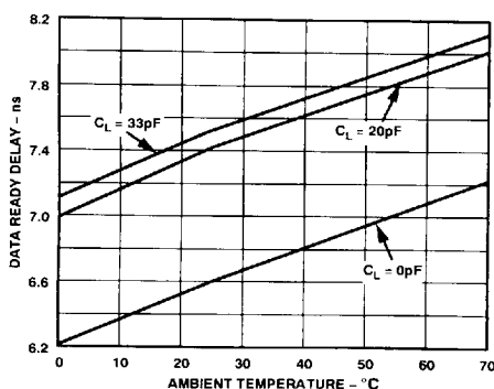
Figure 5. Data Ready Delay vs. Ambient Temperature
