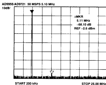
Figure 13. AD9955/AD9721 Output Spectrum
