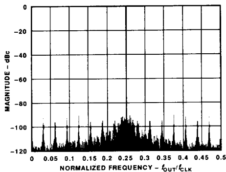
Figure 8. AD9955 Output Spectrum
