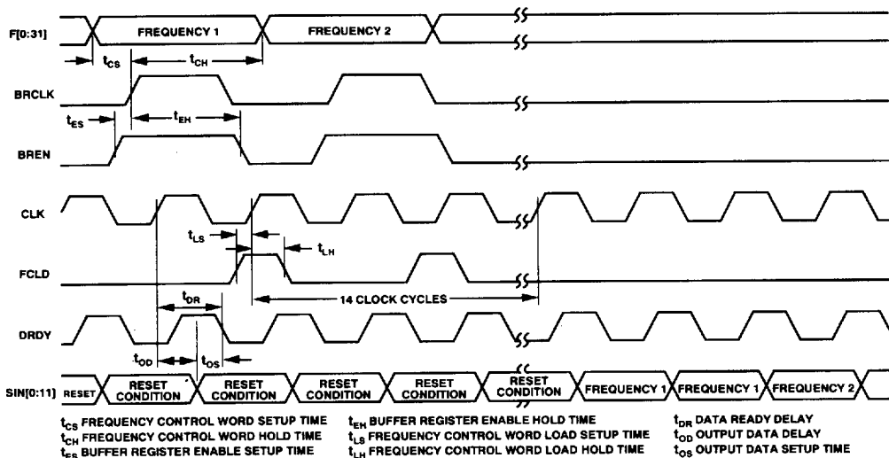
Figure 4. Parallel Mode Timing
