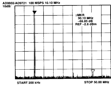
Figure 19. AD9955/AD9721 Output Spectrum
