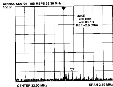
Figure 21. AD9955/AD9721 Output Spectrum
