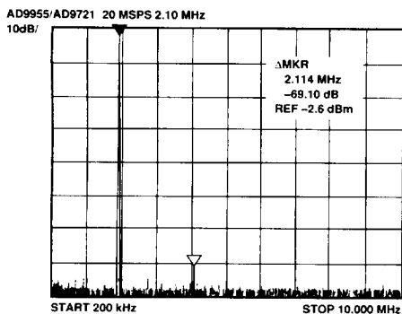
Figure 10. AD9955/AD9721 Output Spectrum
