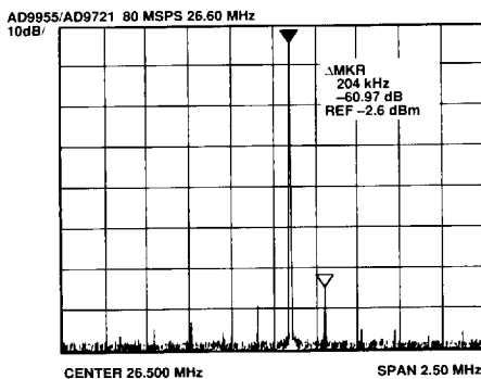
Figure 18. AD9955/AD9721 Output Spectrum
