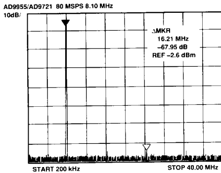
Figure 16. AD9955/AD9721 Output Spectrum
