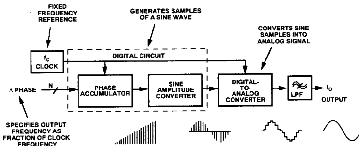
Figure 1. Block Diagram of DDS Generator
