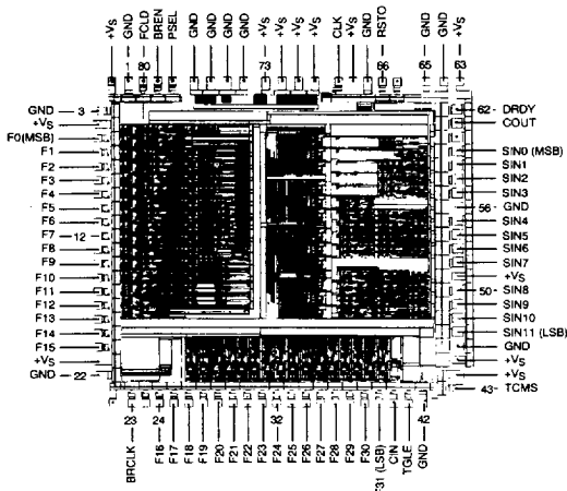
AD9955 Chip Layout
