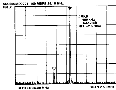
Figure 20. AD9955/AD9721 Output Spectrum
