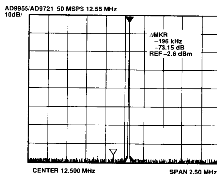
Figure 14. AD9955/AD9721 Output Spectrum
