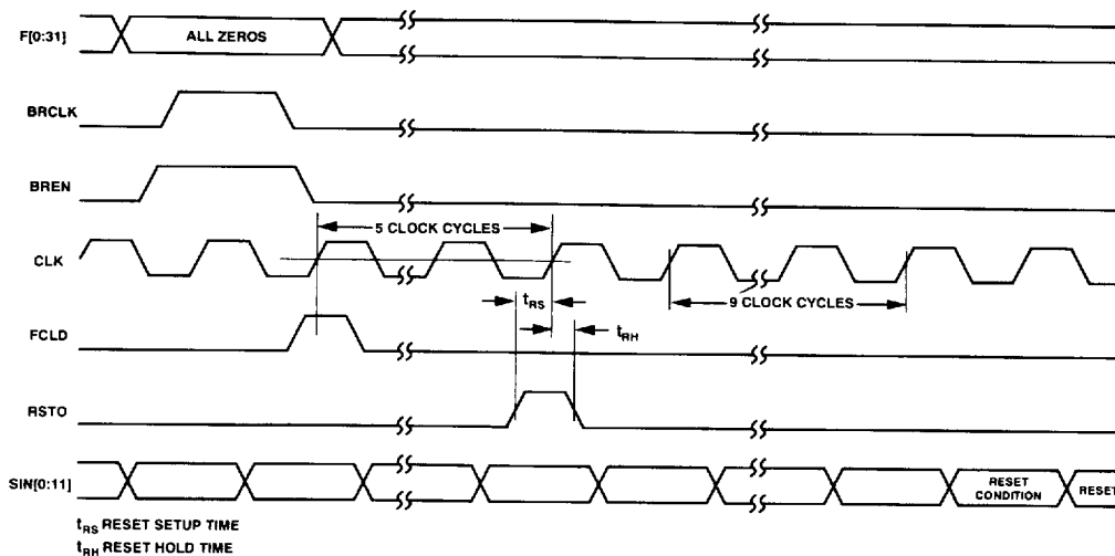
Figure 2. Reset Timing
