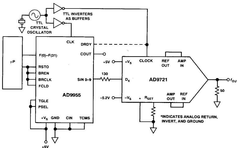
Figure 7. AD9955/AD9721 DDS Synthesizer
