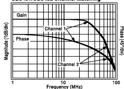
CLC431/CLC432 Channel Matching
