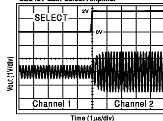
CLC431 Gain-Select Amplifier
