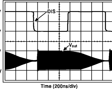
Off-Isolation During Disable (CLC431)
