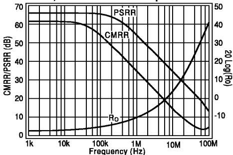
CMRR, PSRR and Closed-loop Ro
