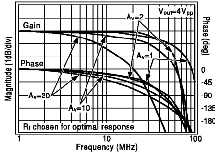
Non-Inverting Frequency Response
