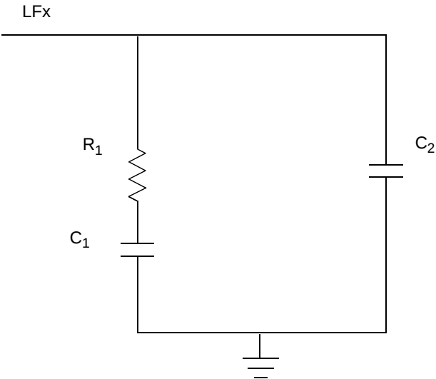
Figure 30. Loop-Filter Component
