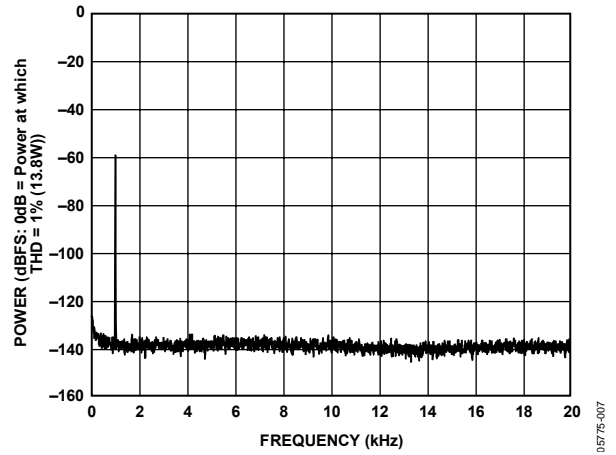
Figure 7. -60 dBFS Output Power into 4 Ω Load
