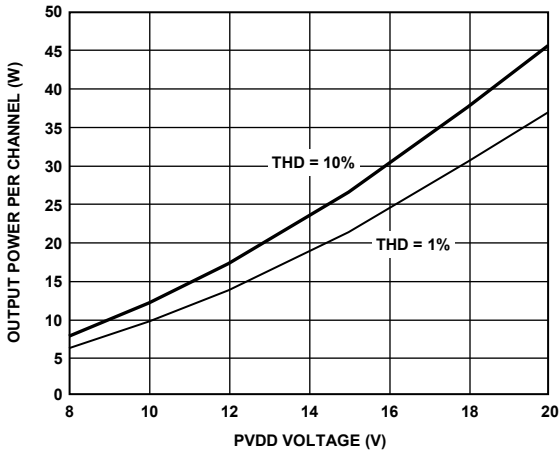
Figure 28. Maximum Power vs. PVDD, Stereo Mode, 4Ω Load
