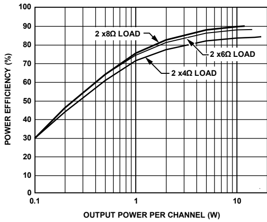
Figure 34. Power Efficiency vs. Output Power, Stereo Mode, PVDD = 12 V
