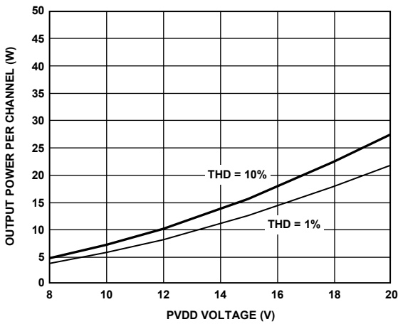
Figure 30. Maximum Power vs. PVDD, Stereo Mode, 8Ω Load
