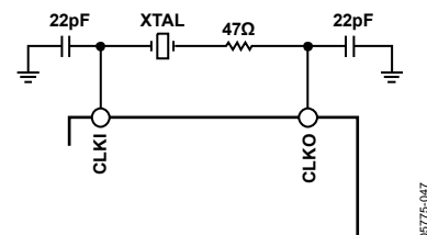
Figure 47. Crystal Connection
