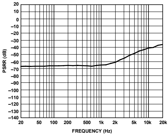
Figure 36. Power Supply Rejection Ratio (PSRR) vs. Frequency
