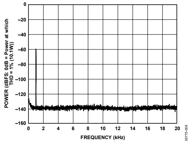
Figure 8. -60 dBFS Output Power into 6 Ω Load
