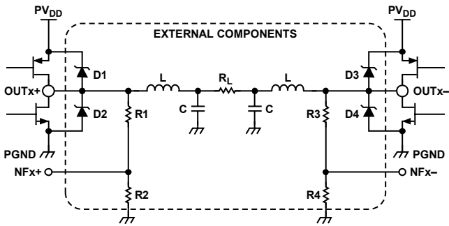
Figure 45. H-Bridge Configuration
