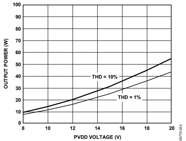
Figure 33. Maximum Power vs. PVDD, Mono Mode, 4Ω Load
