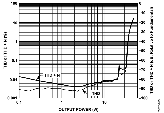
Figure 25. THD and THD + N vs. Output Power, 1 kHz Sine, 4 Ω Load, PVDD = 20 V
