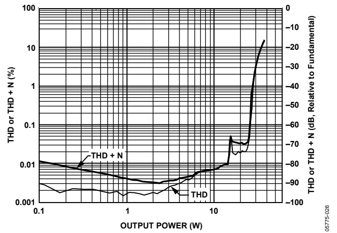
Figure 26. THD and THD + N vs. Output Power, 1 kHz Sine, 6 Ω Load, PVDD = 20 V
