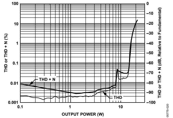
Figure 20. THD and THD + N vs. Output Power, 1 kHz Sine, 6Ω Load, PVDD = 15 V
