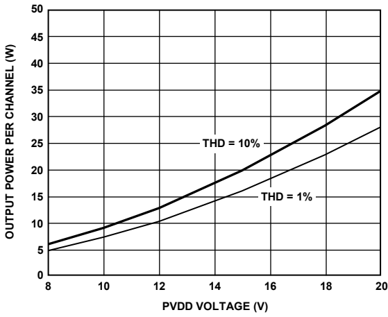
Figure 29. Maximum Power vs. PVDD, Stereo Mode, 6Ω Load
