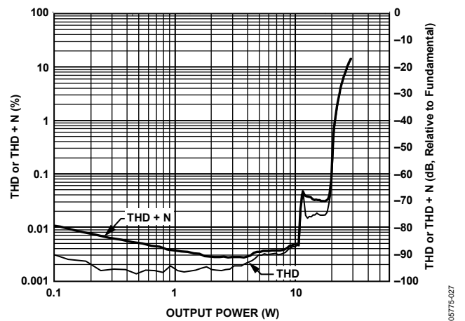
Figure 27. THD and THD + N vs. Output Power, 1 kHz Sine, 8 Ω Load, PVDD = 20 V
