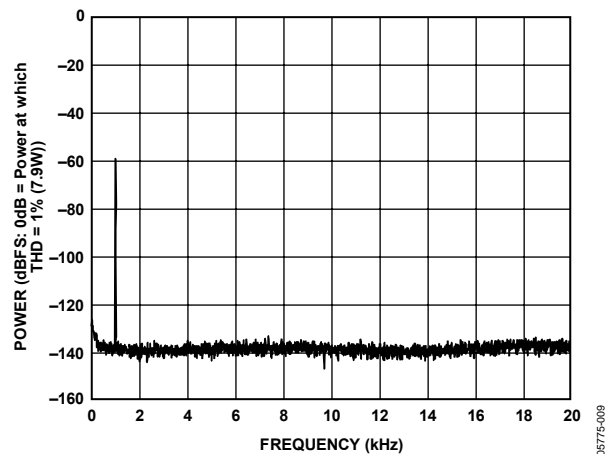
Figure 9. -60 dBFS Output Power into 8 Ω Load
