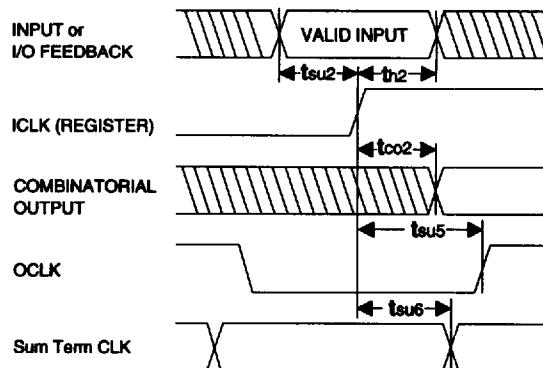
Registered Input
