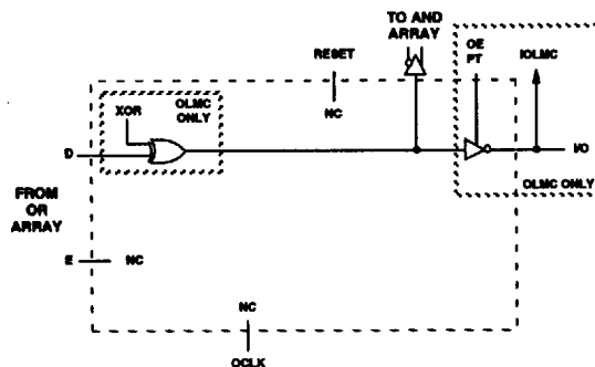
Combinatorial
