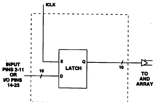
Latched Input
