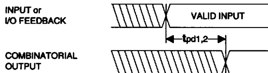
Combinatorial Output
