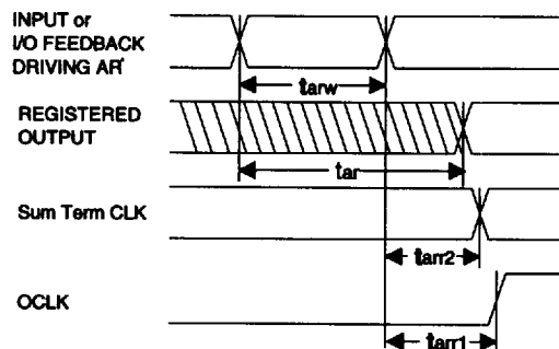
Asynchronous Reset
