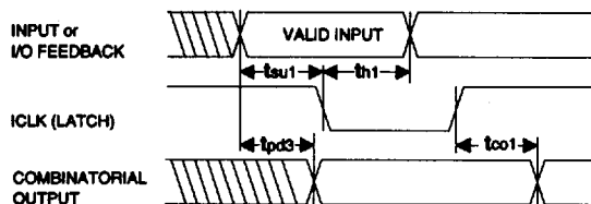
Latched Input
