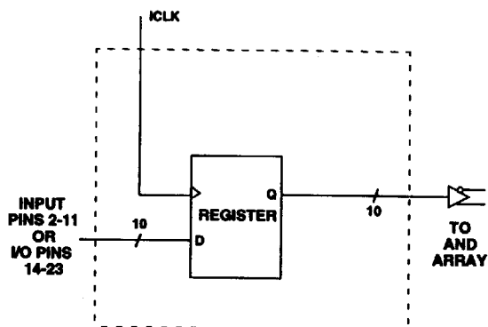
Registered Input
