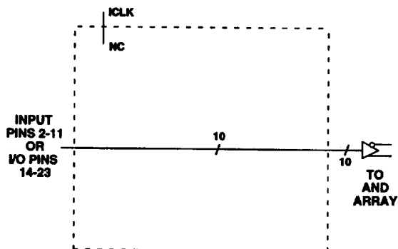
Asynchronous Input
