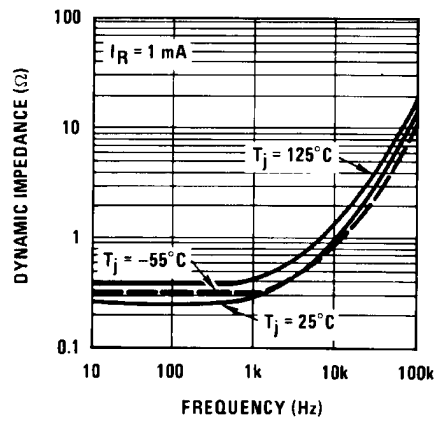
Dynamic Impedance
