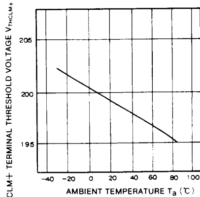
CLM+ TERMINAL THRESHOLD VOLTAGE VS. AMBIENT TEMPERATURE
