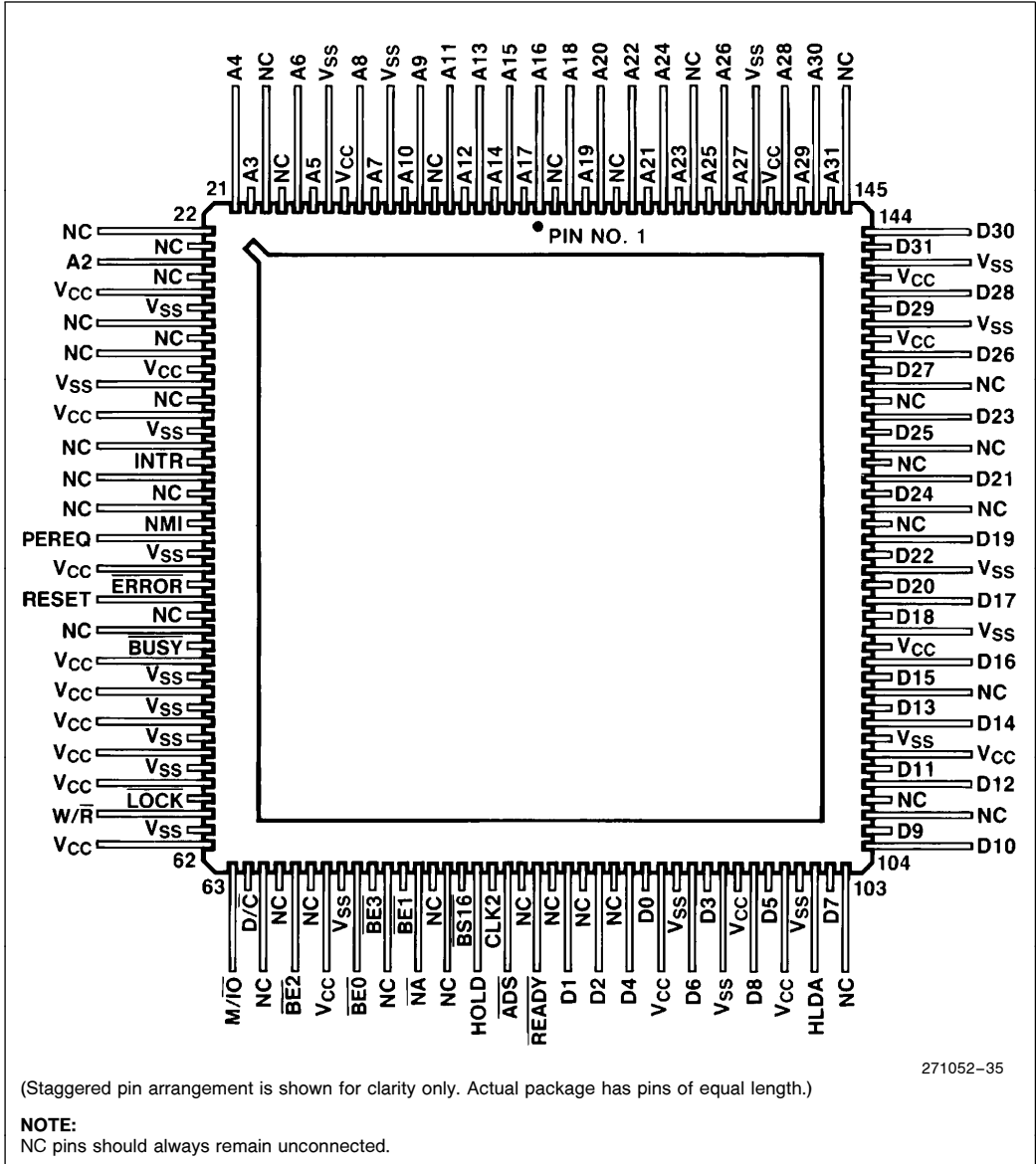
Figure 6-3. Military Intel386™ Processor CQFP Pinout—View from Top Side
