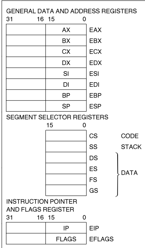
Figure 2-1. Military Intel386 Microprocessor Base Architecture Registers
