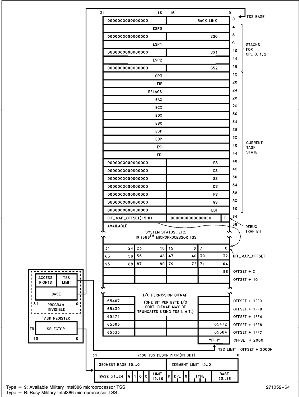
Figure 4-15a. Military Intel386™ Microprocessor TSS and TSS Registers
