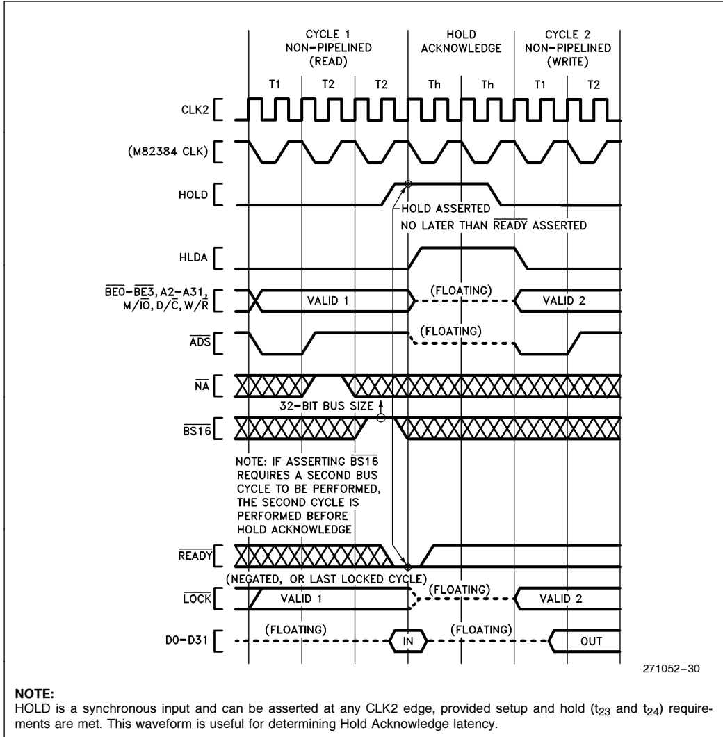
Figure 5-26. Requesting Hold from Active Bus ( \overline{N\bar{A}} negated)
