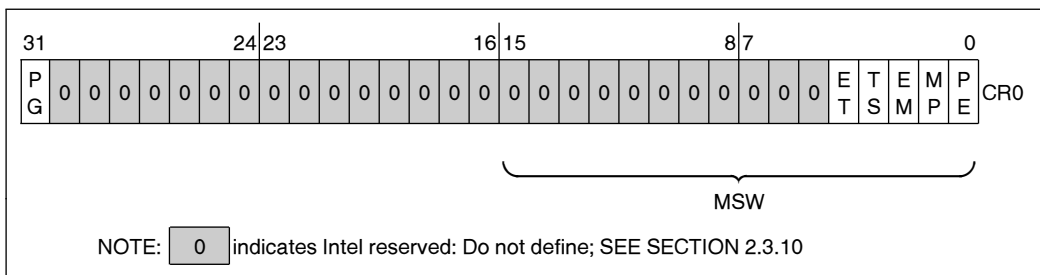
Figure 2-5. Control Register 0
