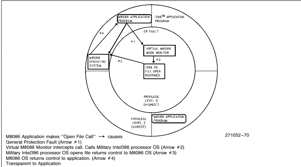
Figure 4-25. Virtual M8086 Environment Interrupt and Call Handling
