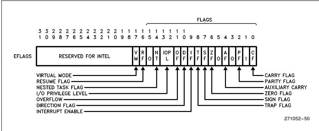
Figure 2-3. Flags Register
