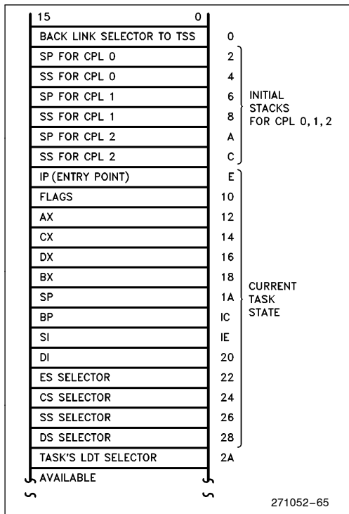
Figure 4-16. 286 TSS
