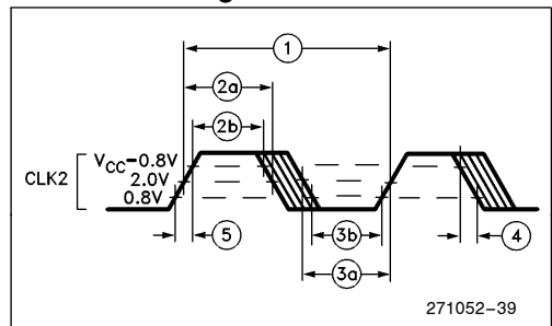
Figure 7-3. CLK2 Timing
