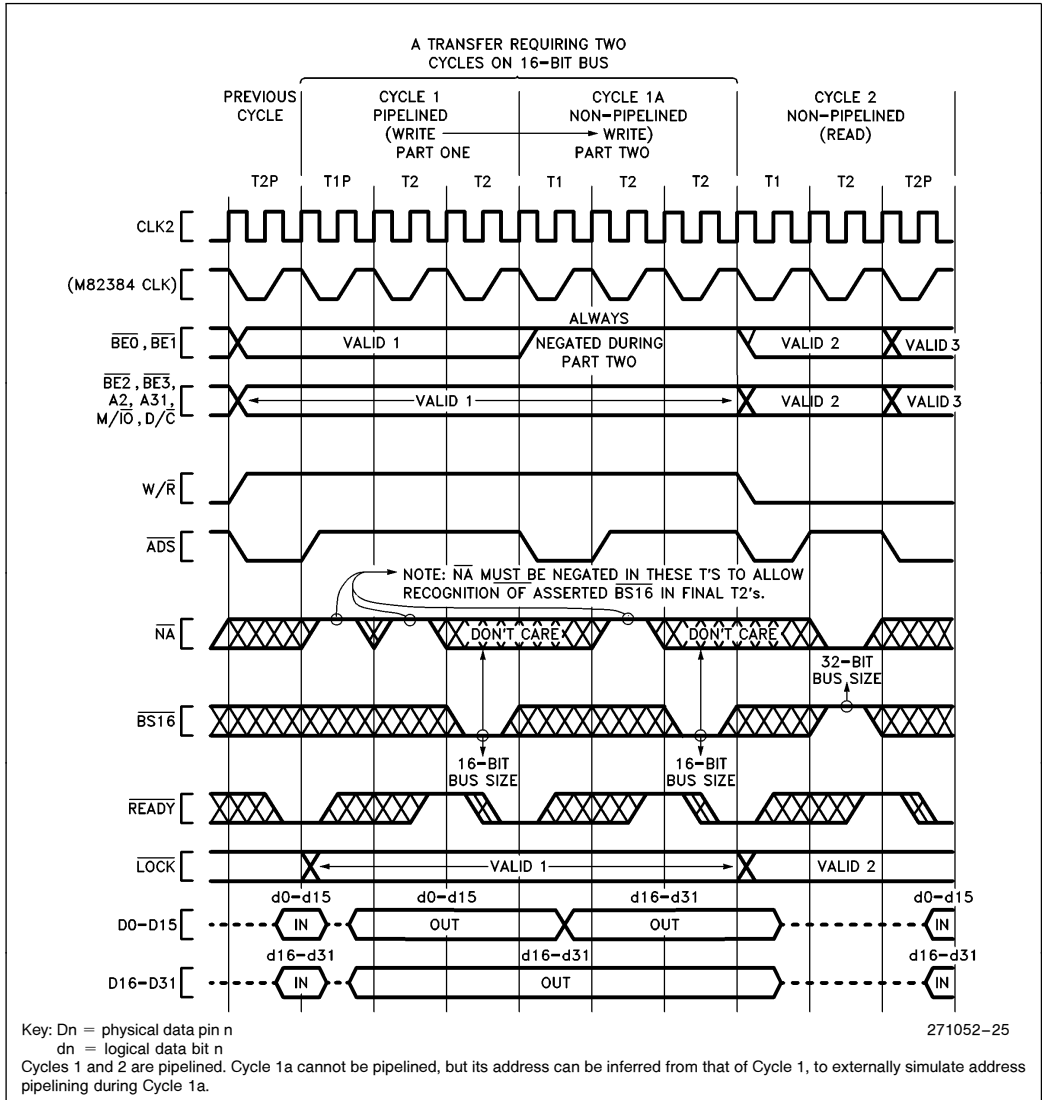
Figure 5-21. Using \overline{NA} and \overline{BS16}
