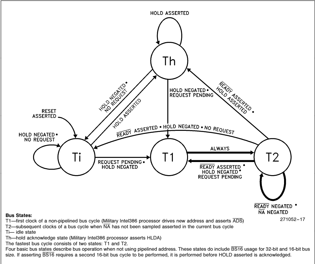
Figure 5-13. Military Intel386™ Processor Bus States (not using pipelined address)
