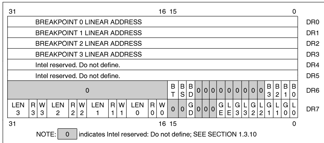
Figure 2-13. Debug Registers
