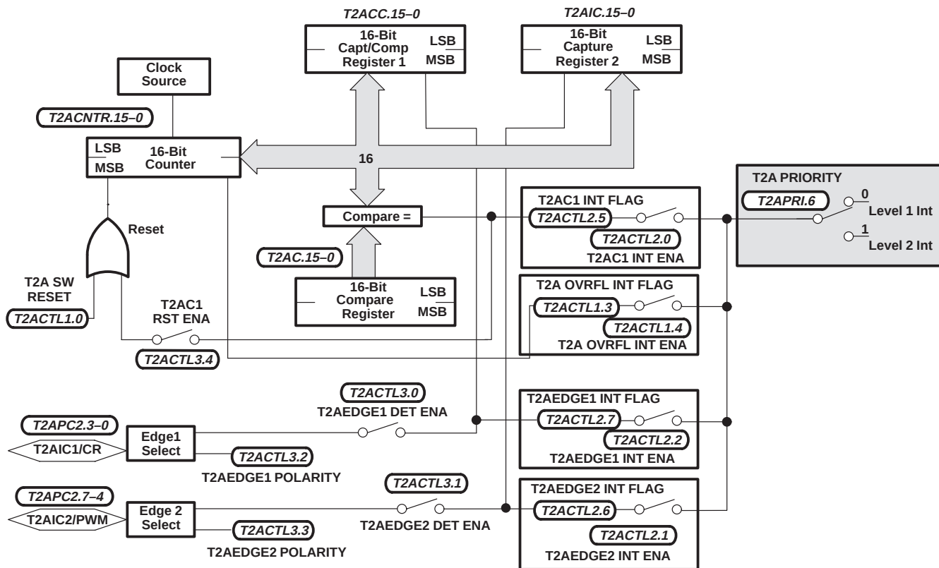
Figure 13. Dual-Capture Mode
