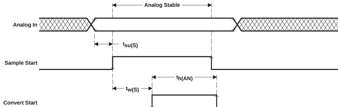
Figure 26. Analog Timing
