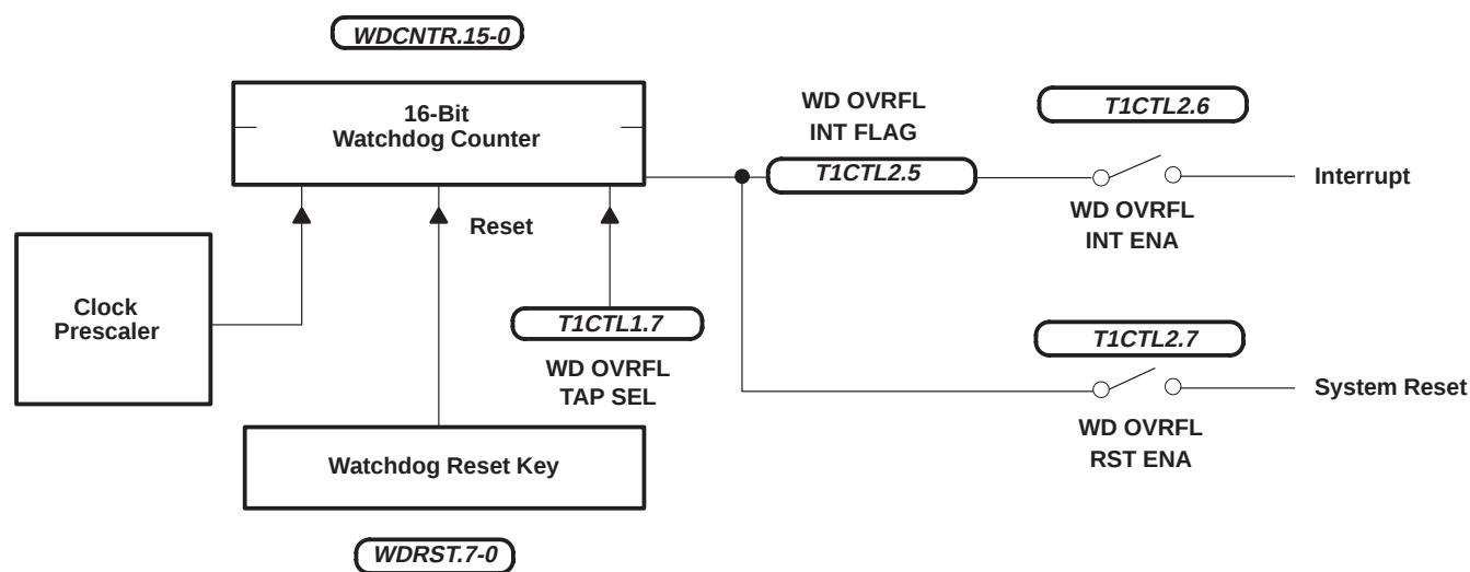
Figure 8. Standard Watchdog
