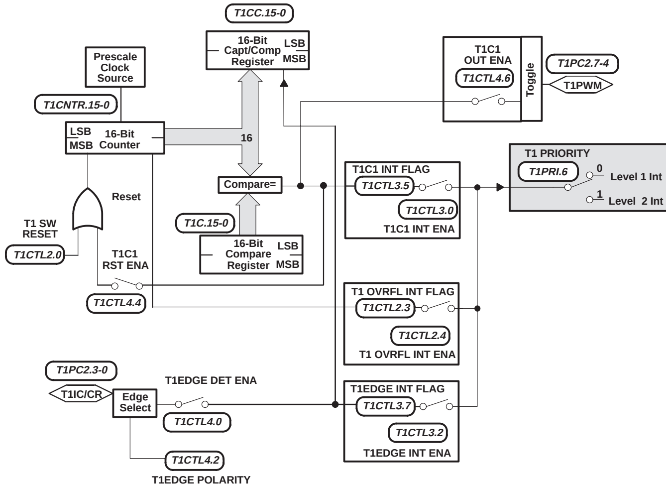
Figure 6. Capture/Compare Mode
