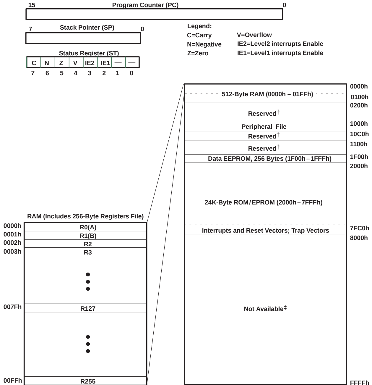
Figure 1. Programmer's Model
