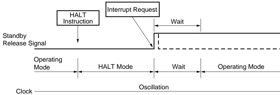
Figure 24-2. HALT Mode Released by Interrupt Request Generation
