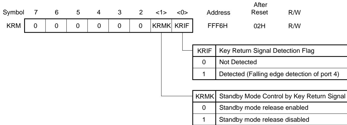
Figure 6-27. Key Return Mode Register Format
