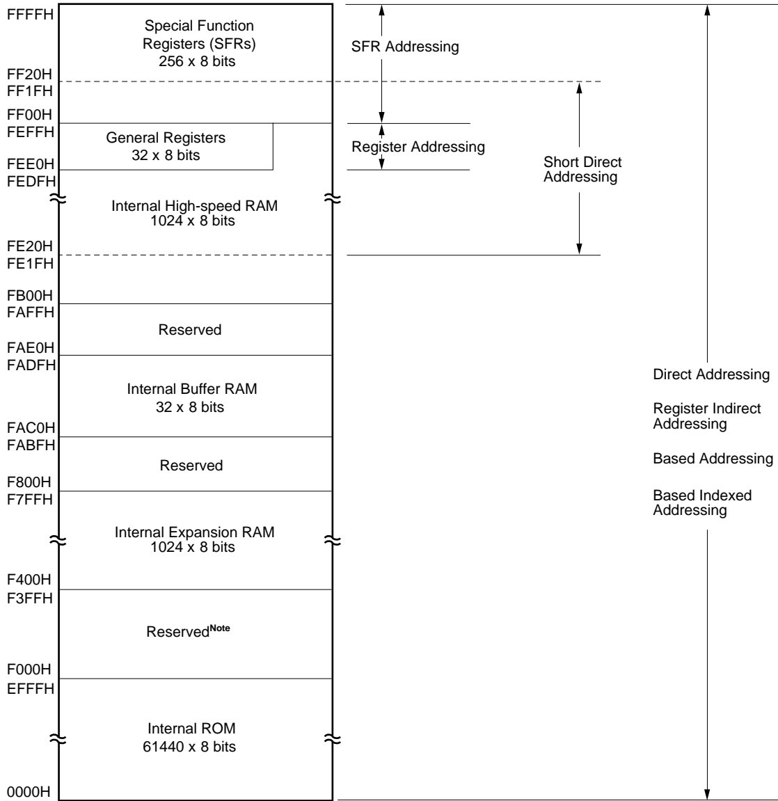
Figure 5-6. Data Memory Addressing ( \mu PD78P078, 78P078Y)
