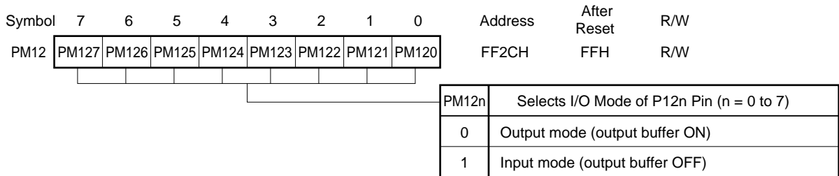
Figure 21-3. Port Mode Register 12 Format
