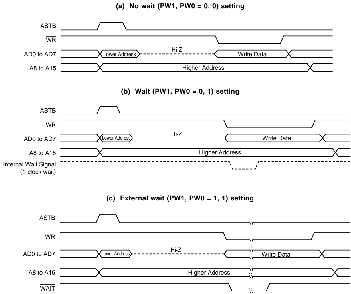
Figure 23-7. External Memory Write Timing in Multiplexed Bus Mode
