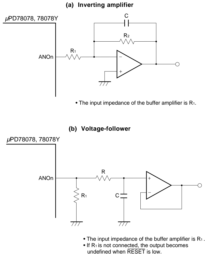
Figure 16-3. Use Example of Buffer Amplifier
