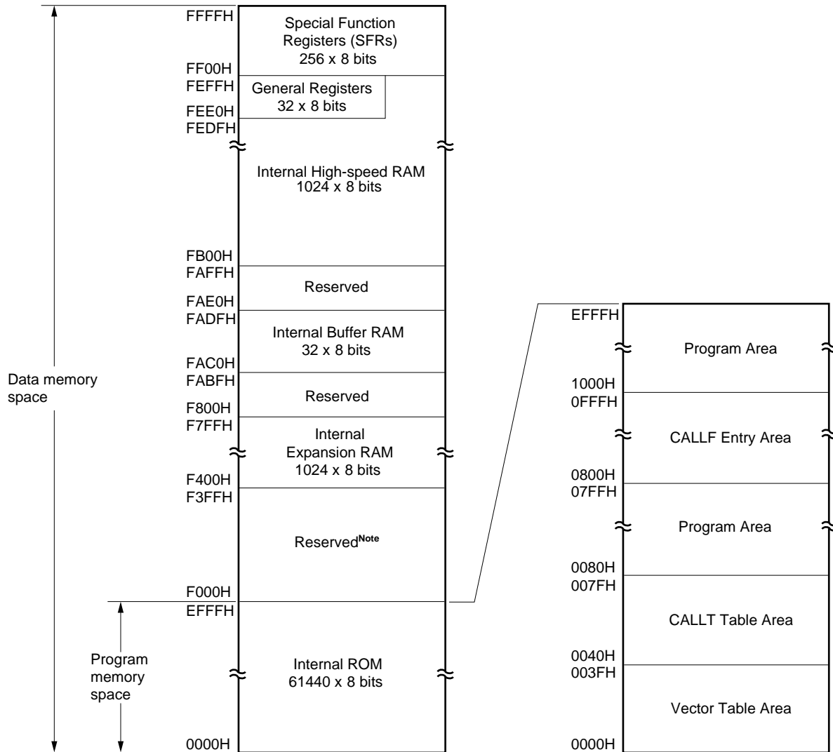
Figure 5-2. Memory Map ( \mu PD78078, 78078Y)
