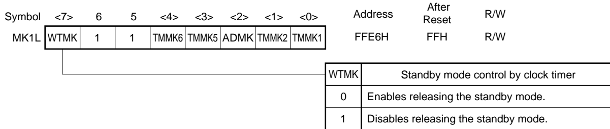
Figure 22-20. Format of Interrupt Mask Flag Register 1L
