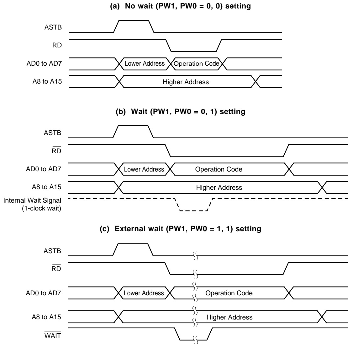
Figure 23-5. Instruction Fetch from External Memory in Multiplexed Bus Mode
