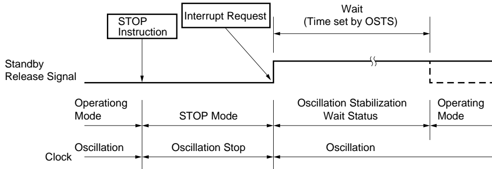
Figure 24-4. STOP Mode Released by Interrupt Request Generation
