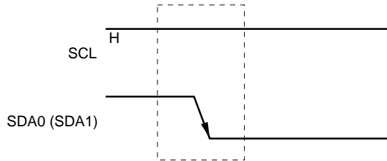
Figure 18-15. Start Condition
