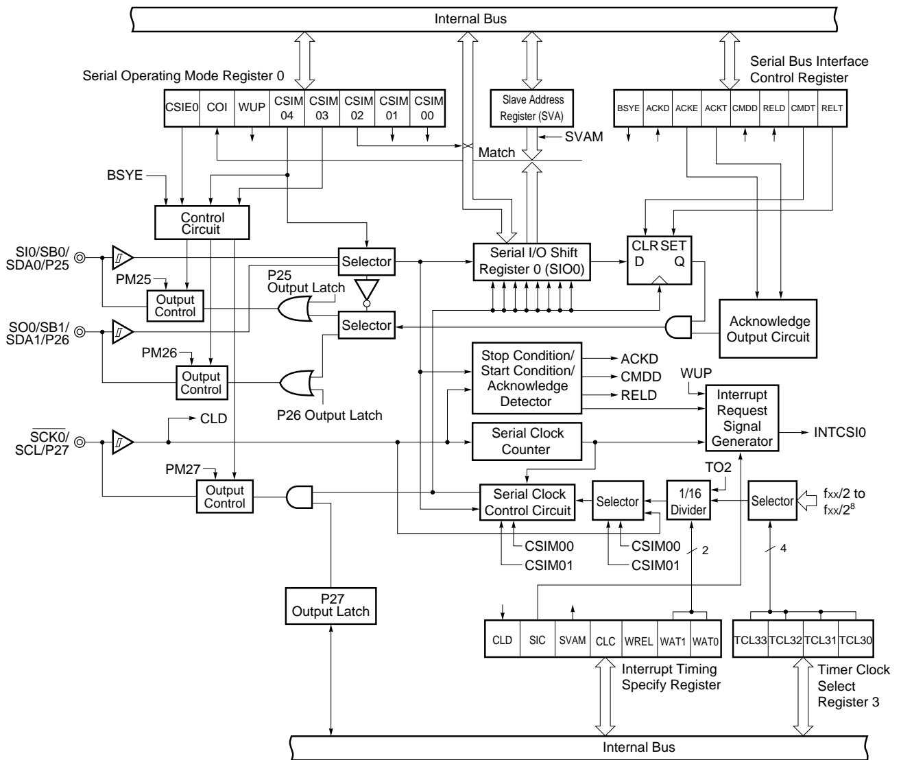
Figure 18-2. Serial Interface Channel 0 Block Diagram
