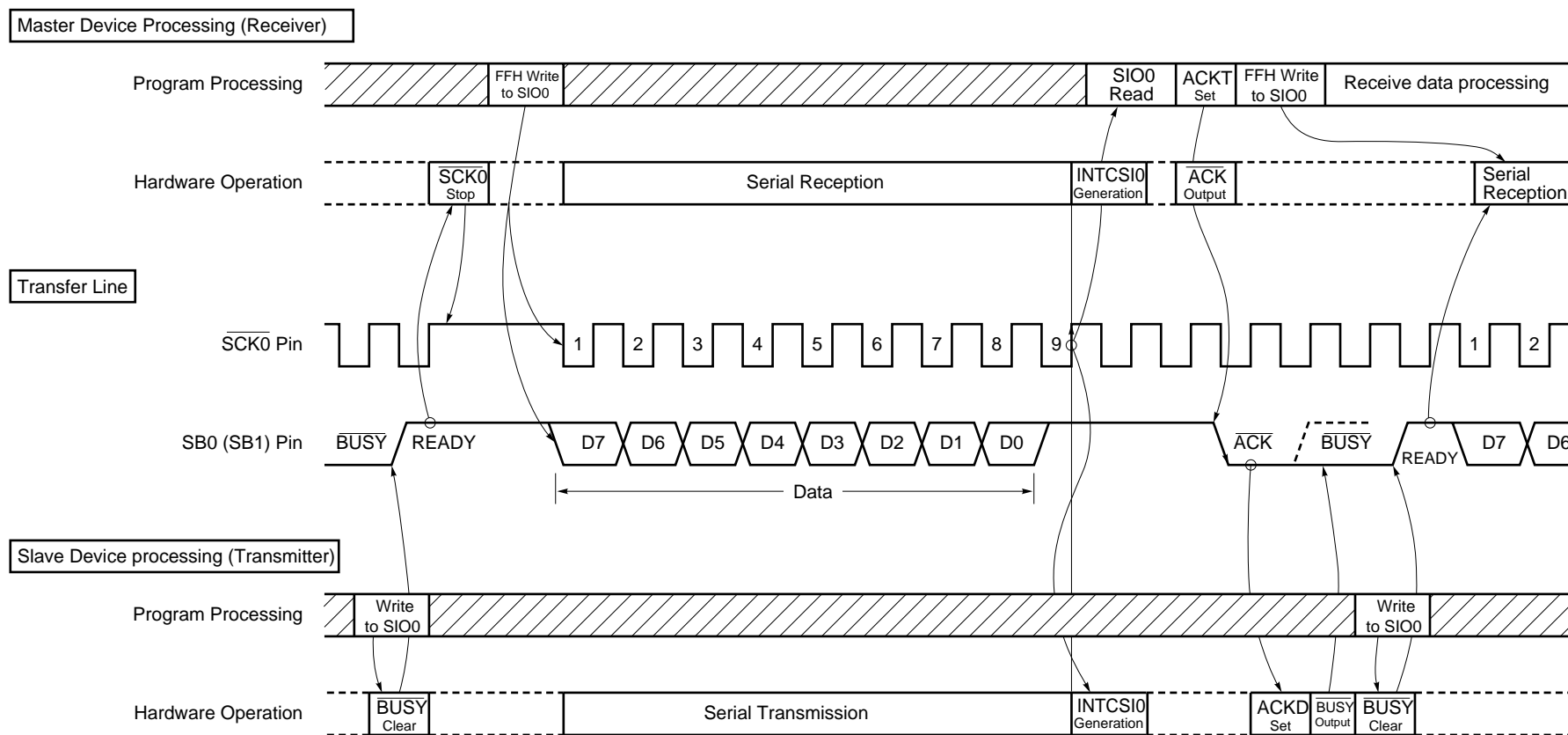
Figure 17-30. Data Transmission from Slave Device to Master Device
