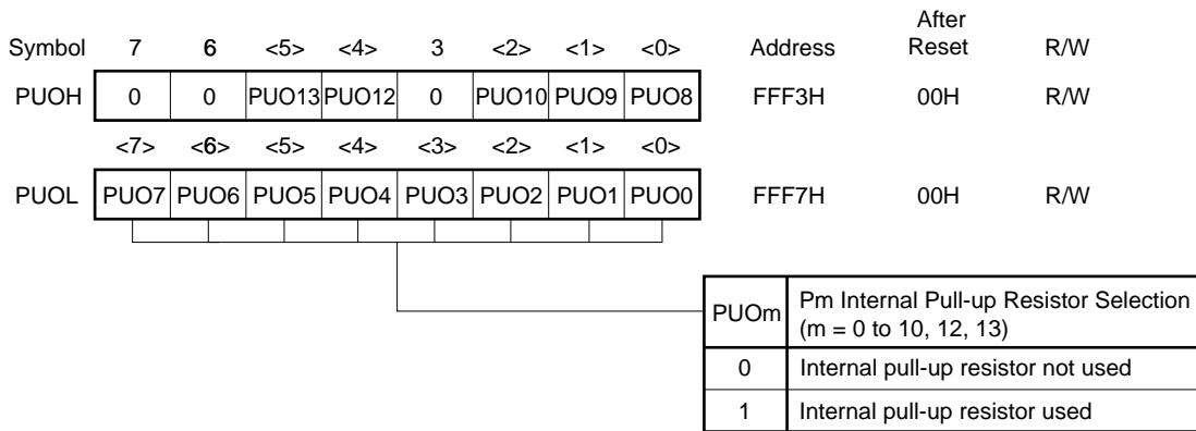
Figure 6-25. Pull-Up Resistor Option Register Format
