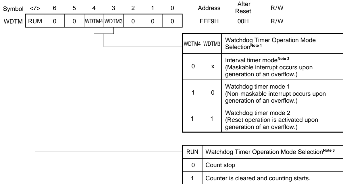
Figure 12-3. Watchdog Timer Mode Register Format
