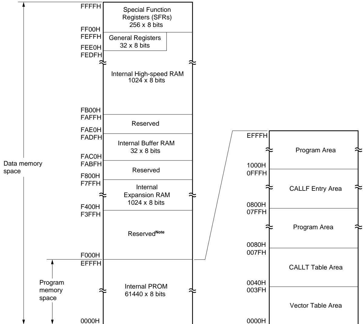
Figure 5-3. Memory Map ( \mu PD78P078, \mu PD78P078Y)
