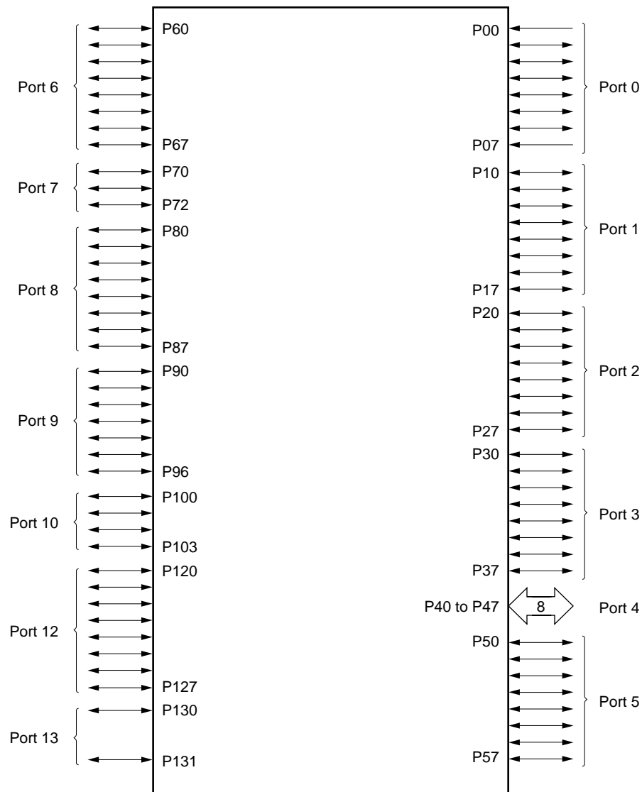
Figure 6-1. Port Types
