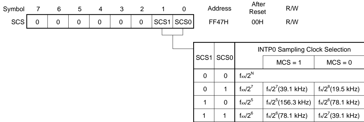
Figure 22-7. Sampling Clock Select Register Format
