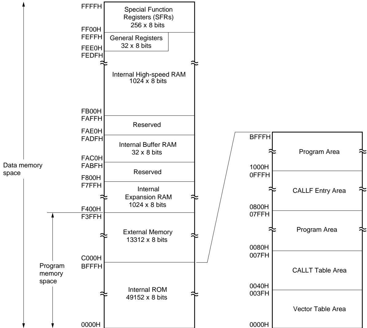
Figure 5-1. Memory Map ( \mu PD78076, 78076Y)
