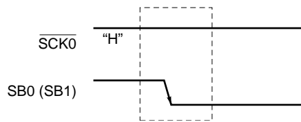
Figure 17-13. Command Signal
