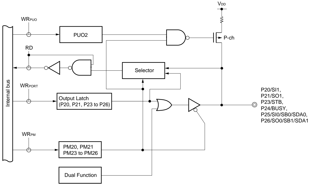
Figure 6-6. Block Diagram of P22 and P27
