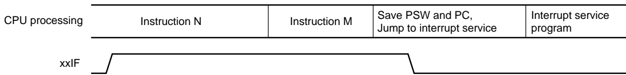
Figure 22-17. Interrupt Request Hold
