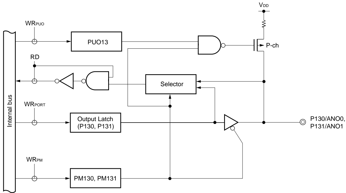
Figure 6-23. Block Diagram of P130 and P131
