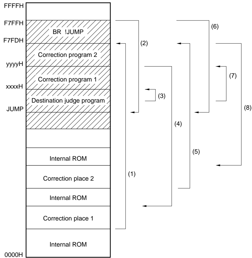
Figure 26-10. Program Transition Diagram (when Two Places are Corrected)
