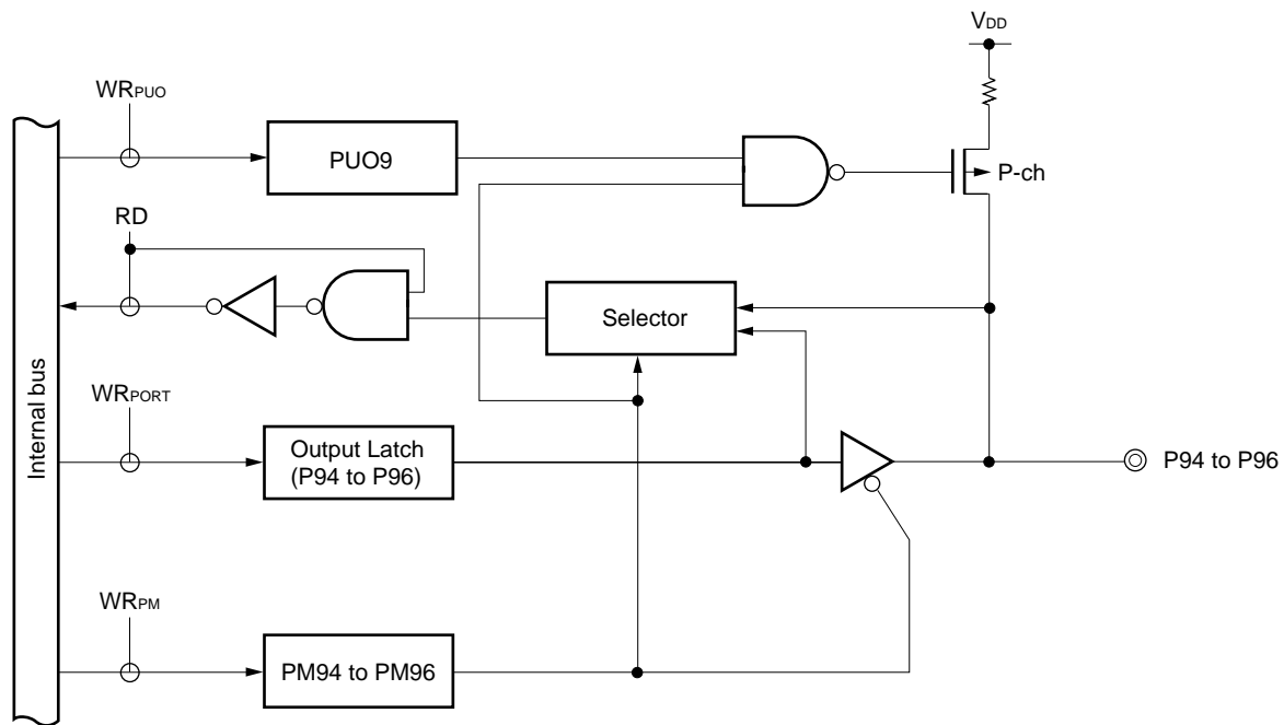
Figure 6-19. Block Diagram of P94 to P96
