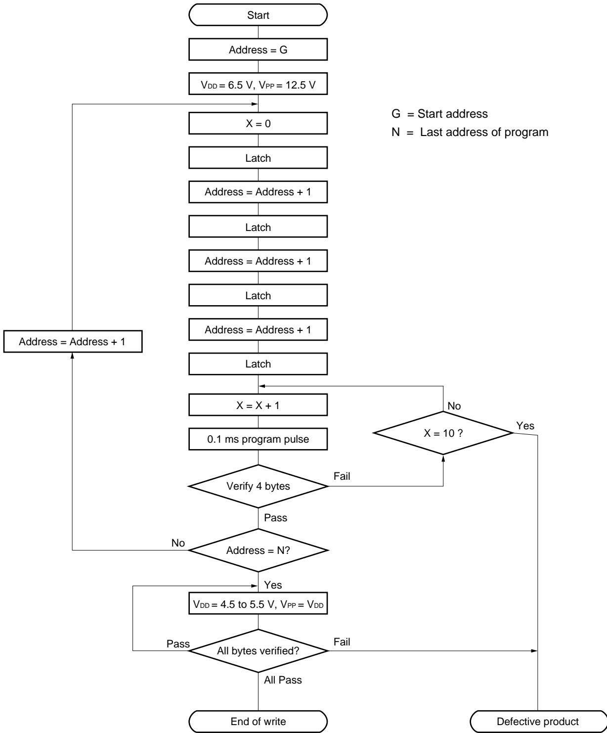
Figure 27-3. Page Program Mode Flowchart
