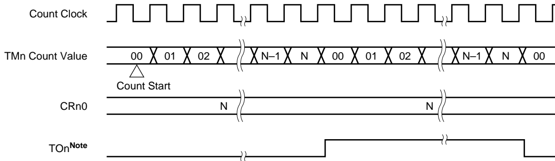
Figure 10-13. Timing of Square Wave Output Operation
