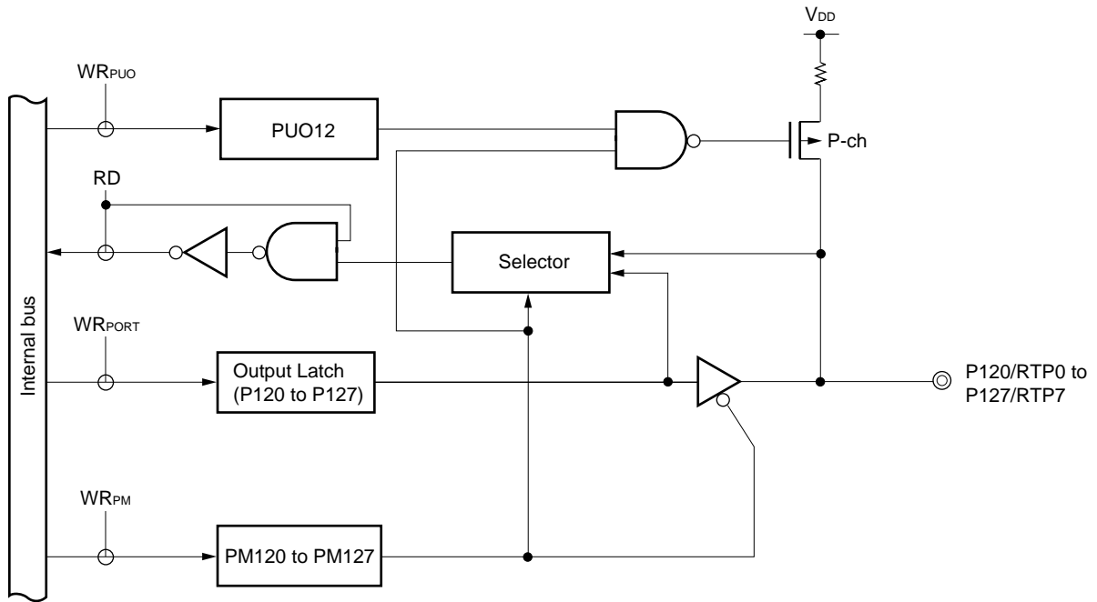
Figure 6-22. Block Diagram of P120 to P127
