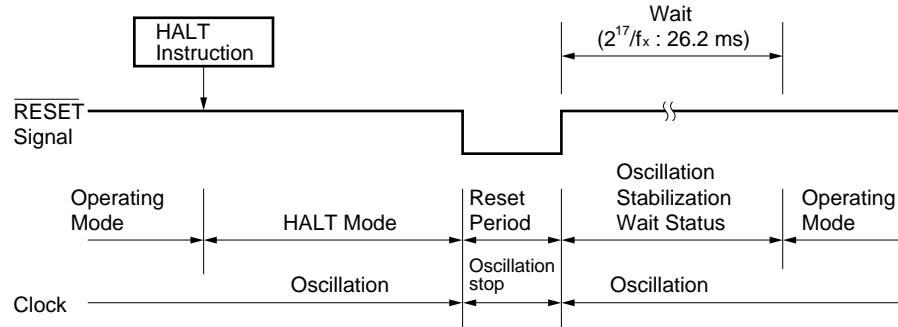
Figure 24-3. HALT Mode Released by \overline{\text{RESET}} Input
