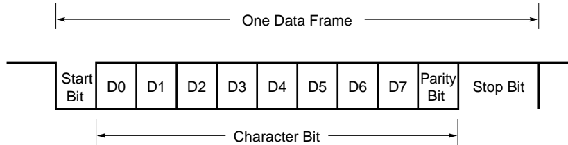
Figure 20-7. Asynchronous Serial Interface Transmit/Receive Data Format
