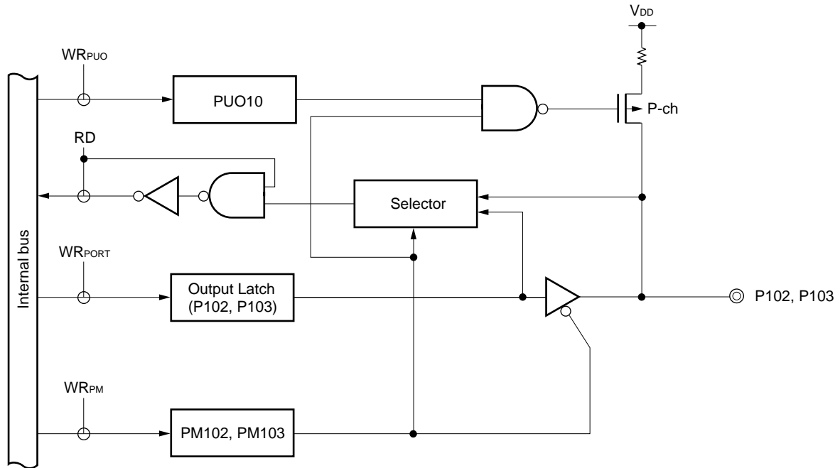
Figure 6-21. Block Diagram of P102 and P103
