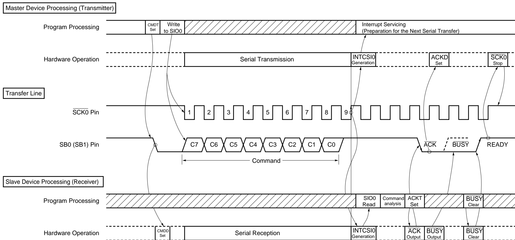
Figure 17-28. Command Transmission from Master Device to Slave Device
