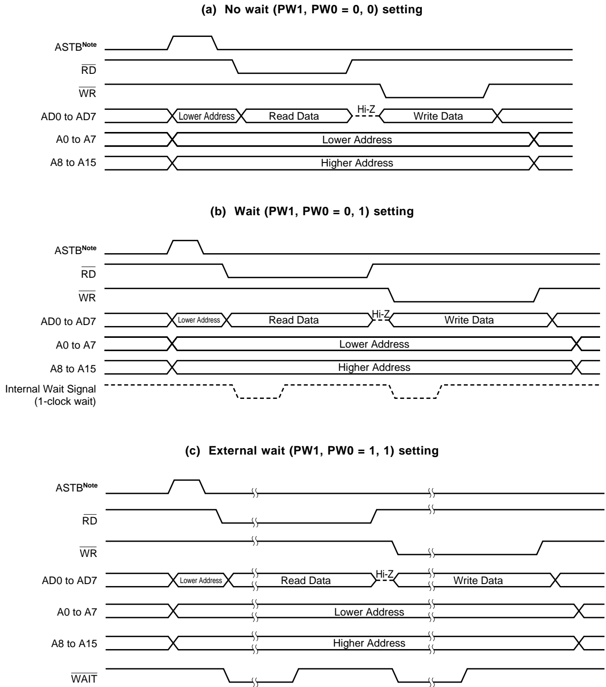
Figure 23-12. External Memory Read Modify Write Timing in Separate Bus Mode
