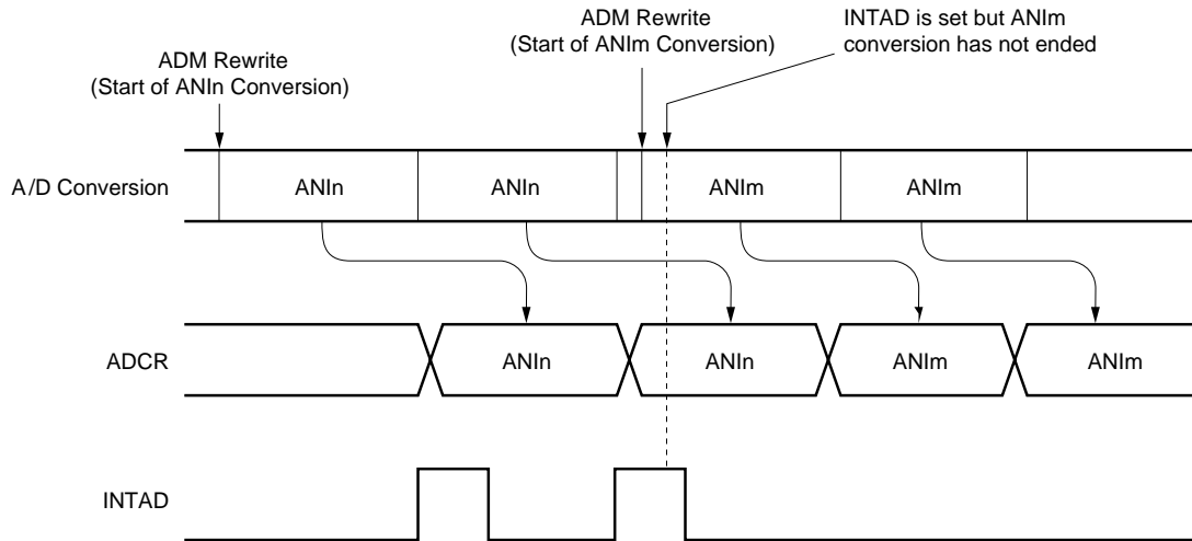
Figure 15-11. A/D Conversion End Interrupt Request Generation Timing
