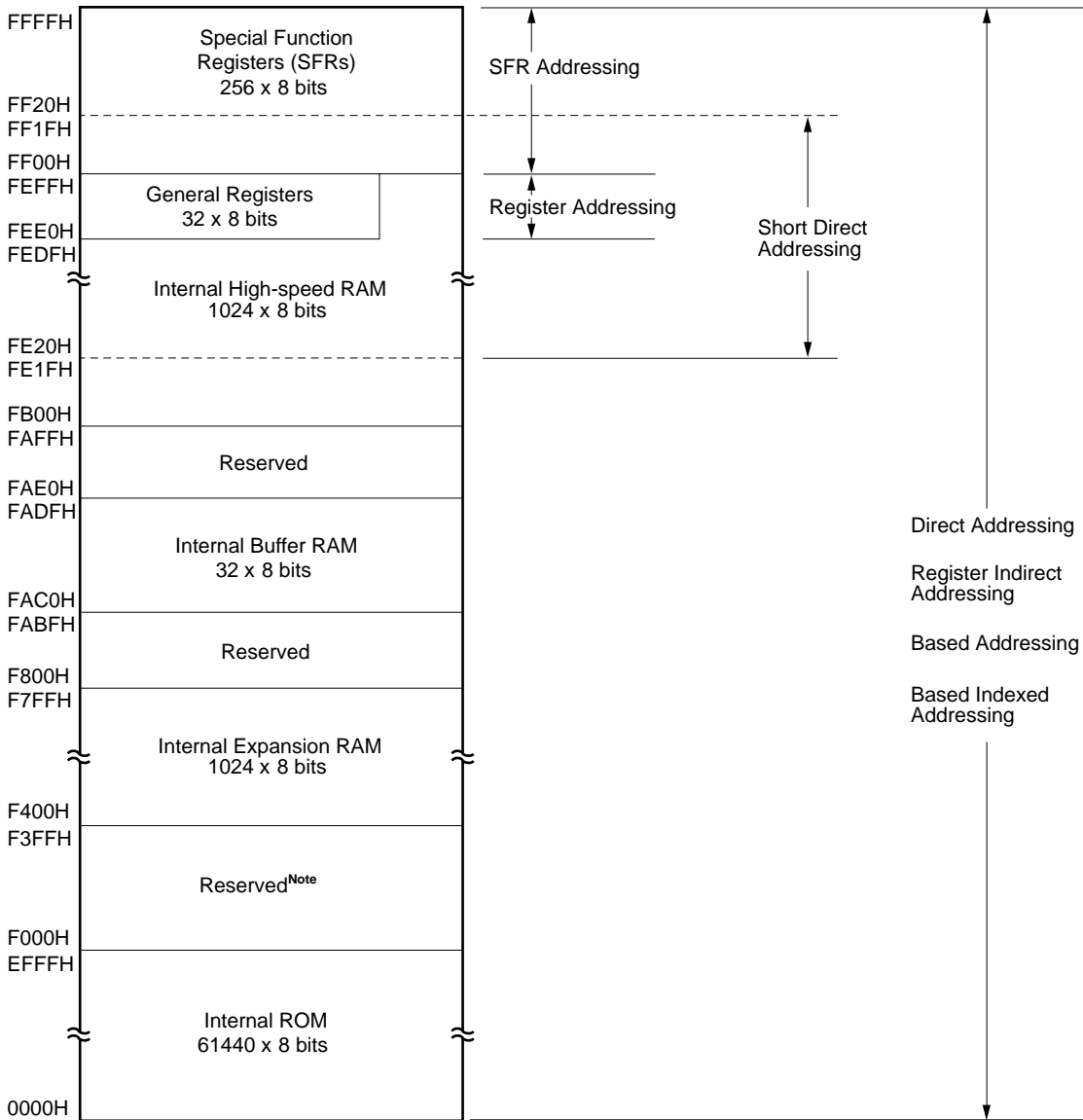
Figure 5-5. Data Memory Addressing ( \mu PD78078, 78078Y)
