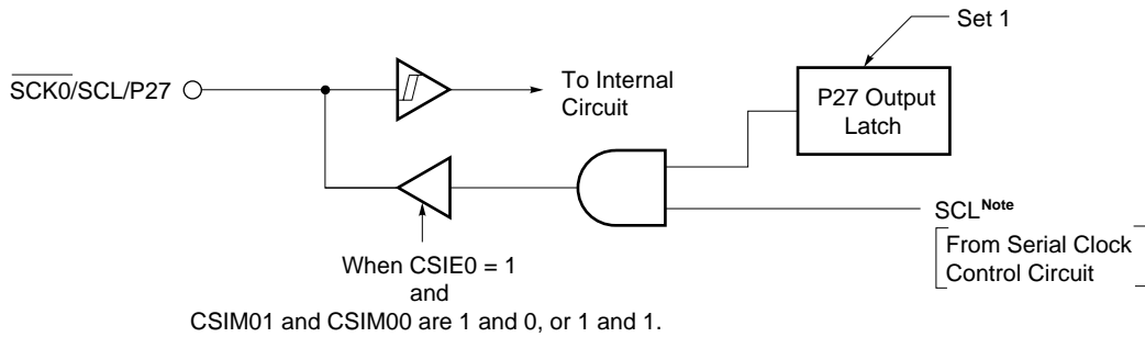
Figure 18-28. \overline{\text{SCK0/SCL/P27}} Pin Configuration
