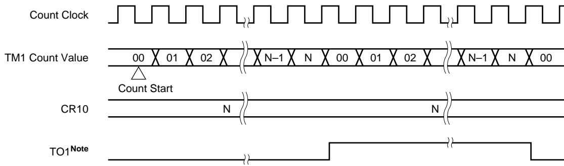
Figure 9-10. Timing of Square Wave Output Operation
