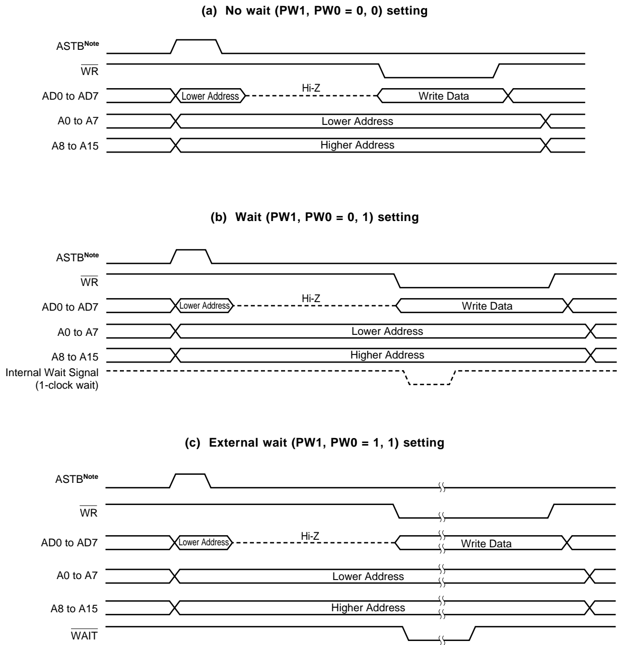
Figure 23-11. External Memory Write Timing in Separate Bus Mode
