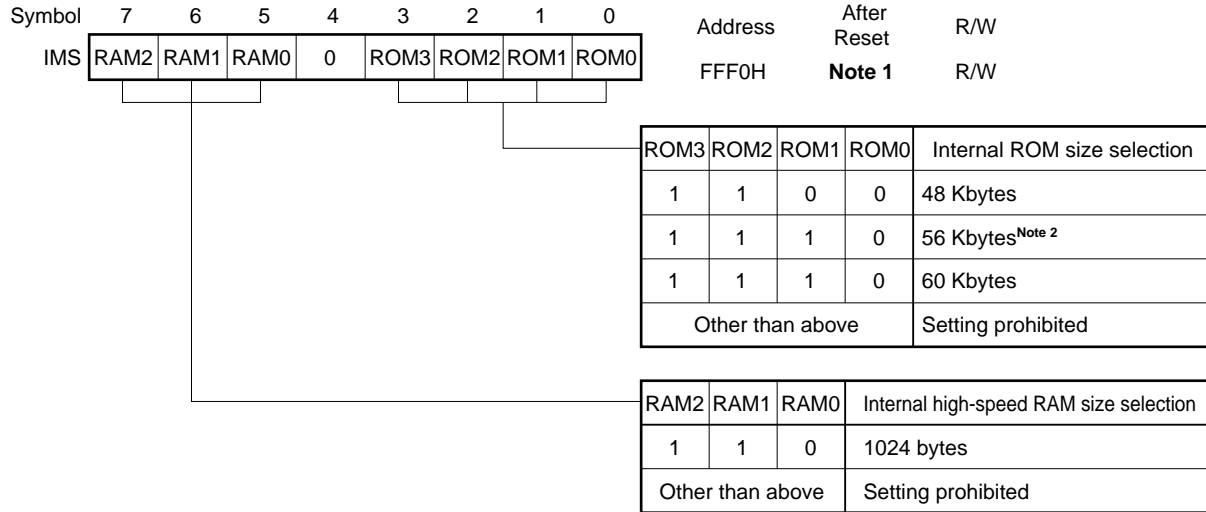
Figure 23-3. Internal Memory Size Switching Register Format
