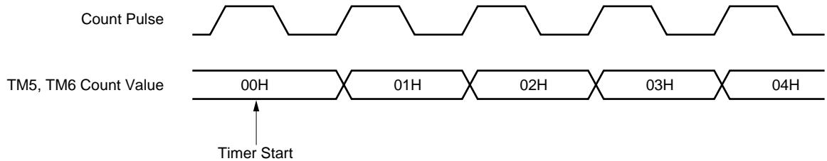
Figure 10-19. 8-bit Timer Registers 5 and 6 Start Timings
