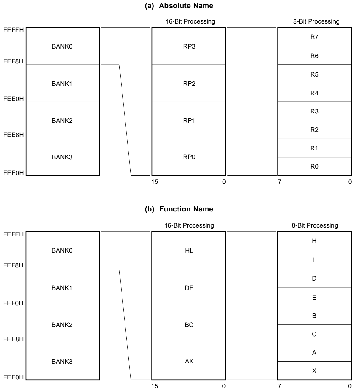
Figure 5-12. General Register Configuration
