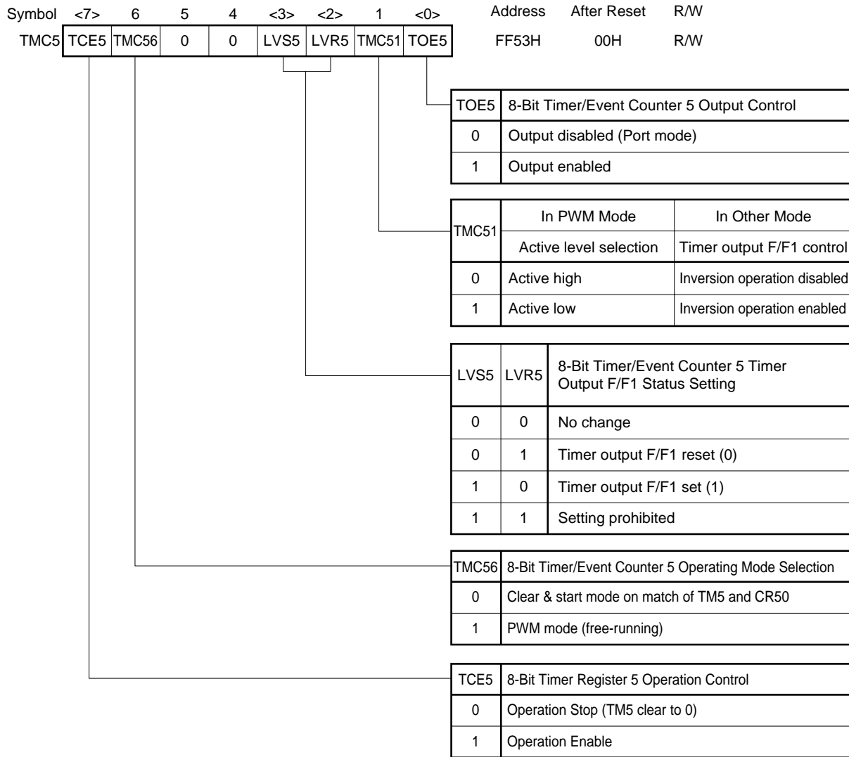
Figure 10-5. 8-Bit Timer Output Control Register Format
