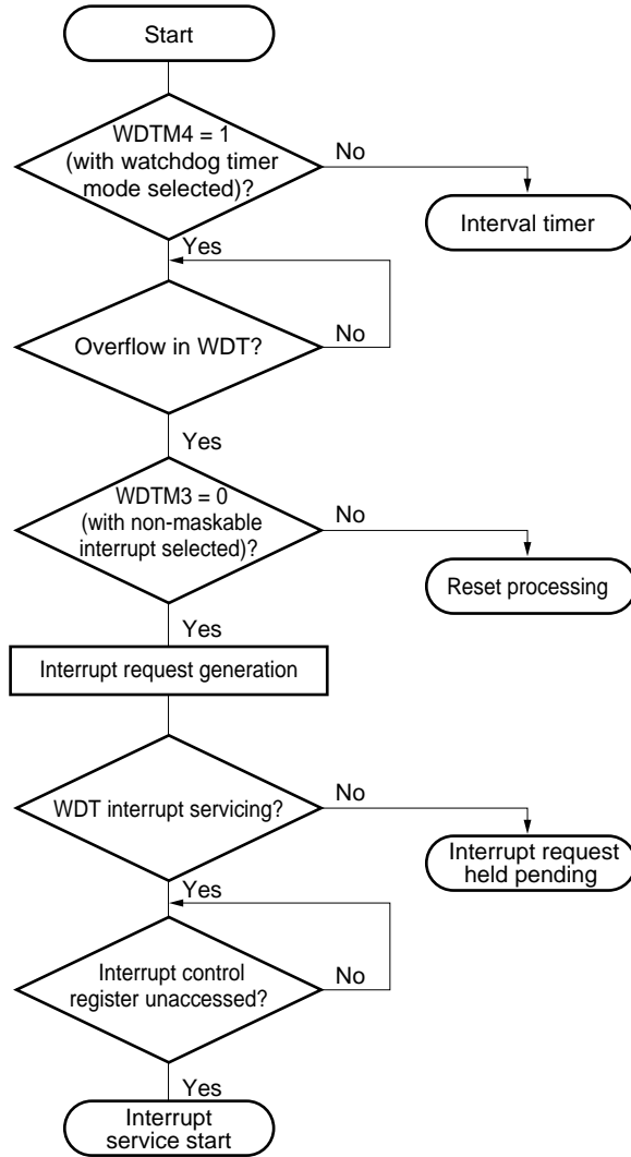
Figure 22-10. Flowchart from Non-Maskable Interrupt Generation to Acknowledge
