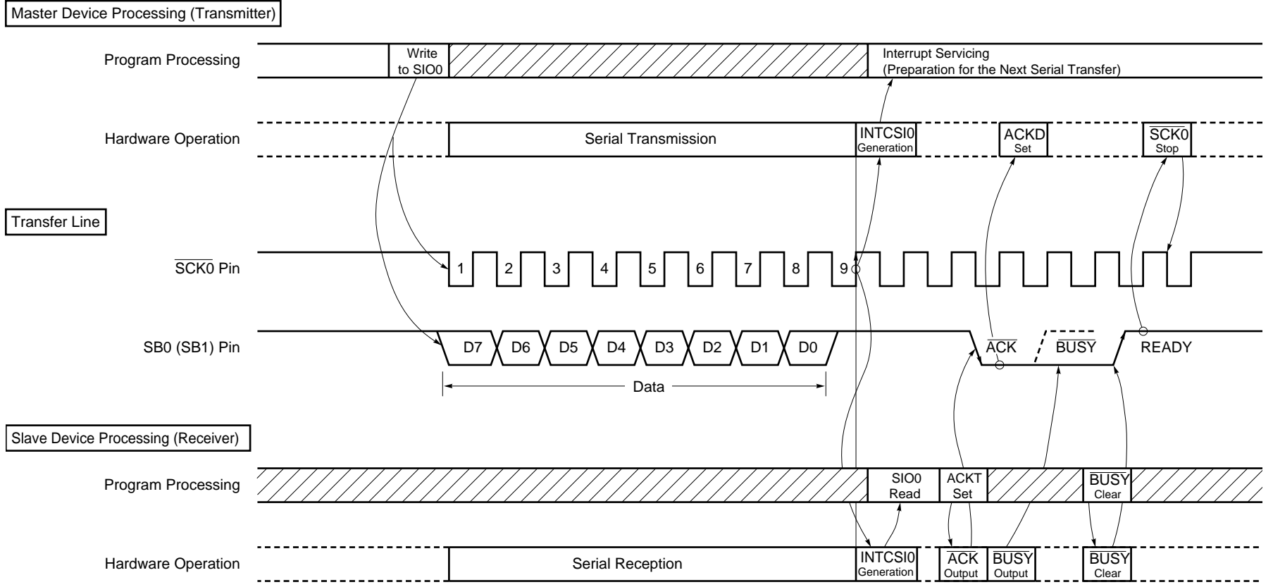
Figure 17-29. Data Transmission from Master Device to Slave Device
