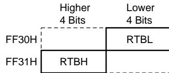
Figure 21-2. Real-time Output Buffer Register Configuration
