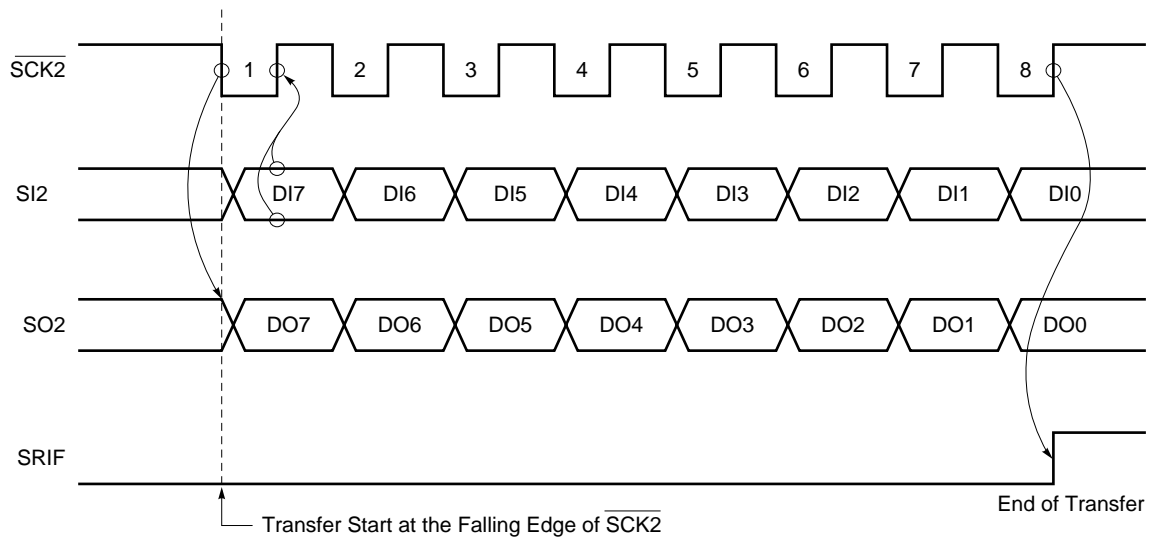
Figure 20-12. 3-Wire Serial I/O Mode Timing
