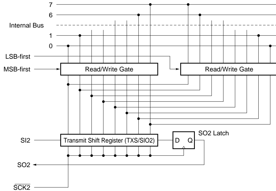
Figure 20-13. Circuit of Switching in Transfer Bit Order
