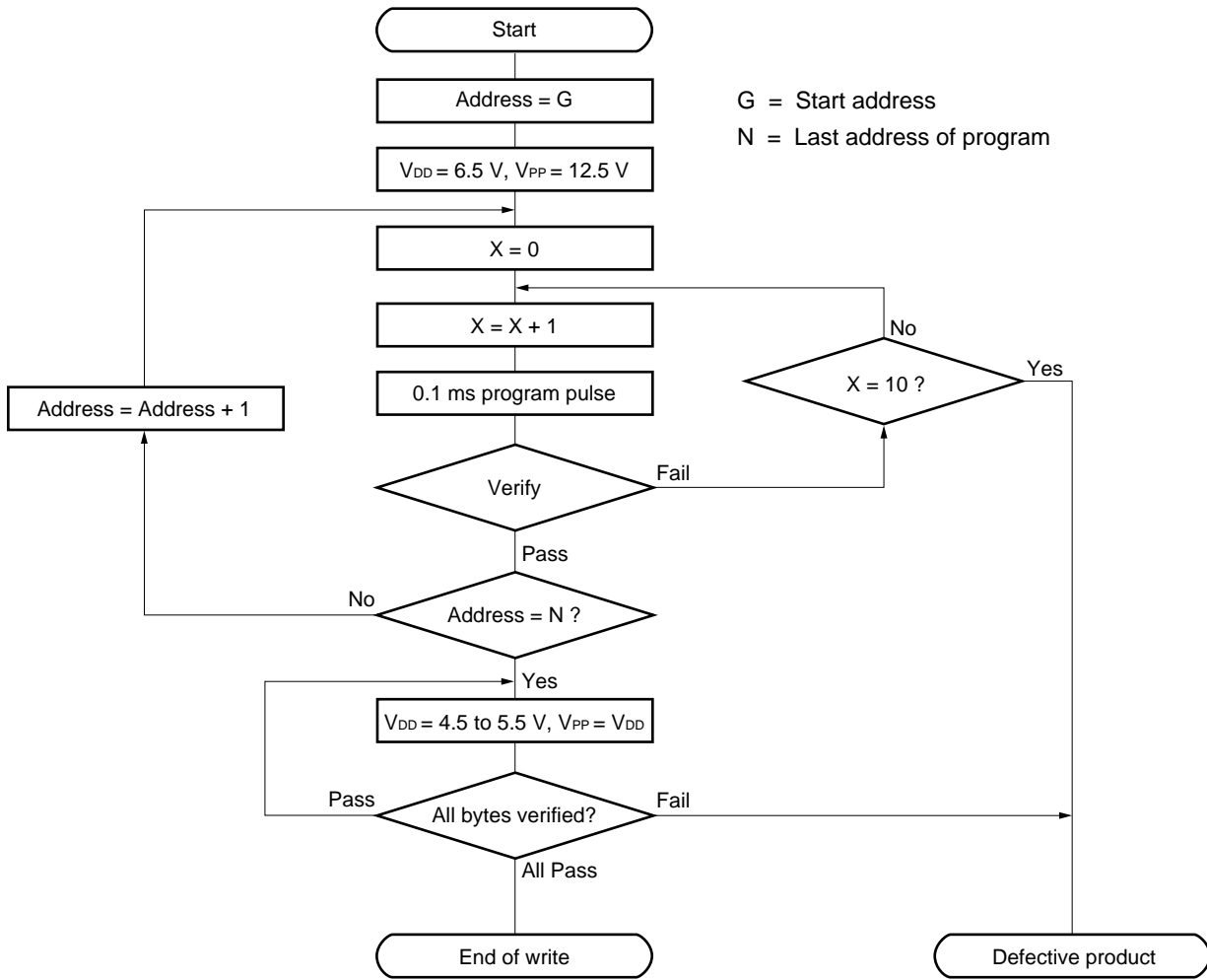
Figure 27-5. Byte Program Mode Flowchart
