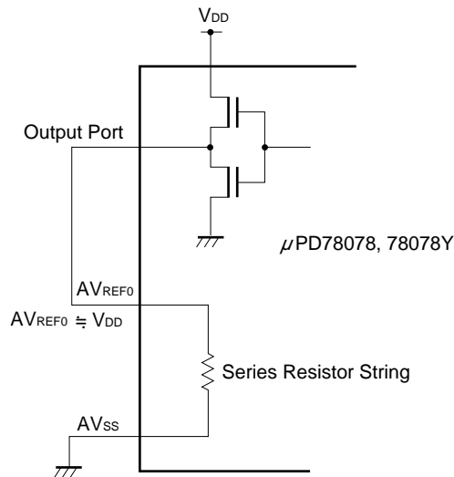
Figure 15-9. Example of Method of Reducing Current Consumption in Standby Mode
