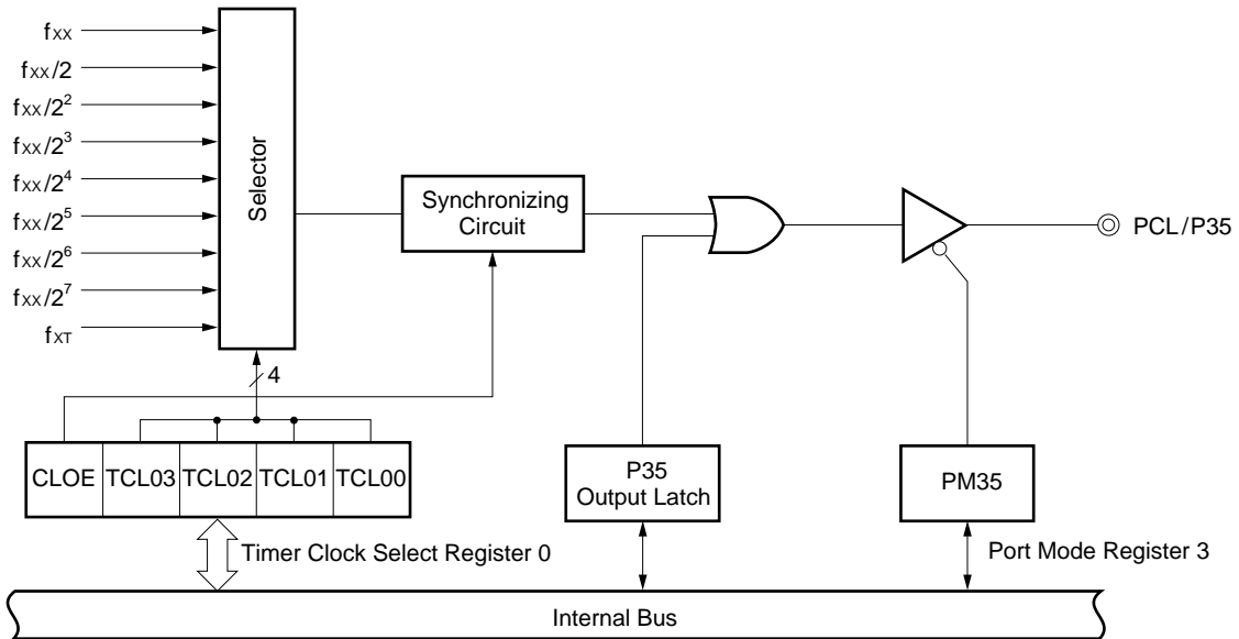
Figure 13-2. Clock Output Control Circuit Block Diagram
