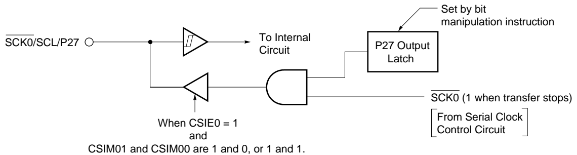
Figure 18-27. \overline{\text{SCK0/SCL/P27}} Pin Configuration
