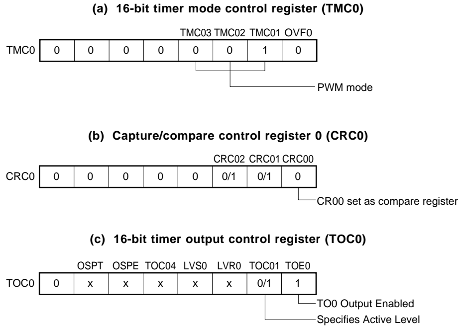
Figure 8-13. Control Register Settings for PWM Output Operation
