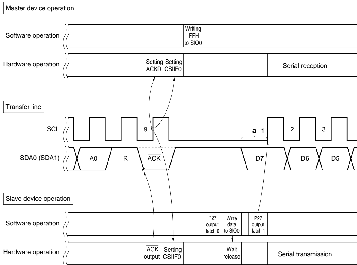
Figure 18-25. Slave Wait Release (Transmission)
