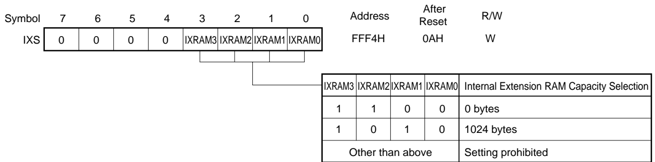
Figure 27-2. Internal Extension RAM Size Switching Register Format
