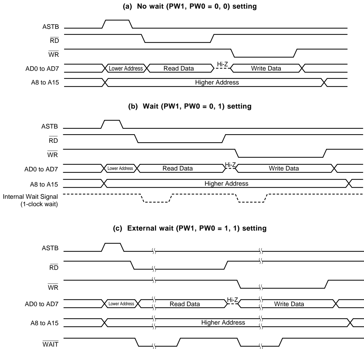
Figure 23-8. External Memory Read Modify Write Timing in Multiplexed Bus Mode
