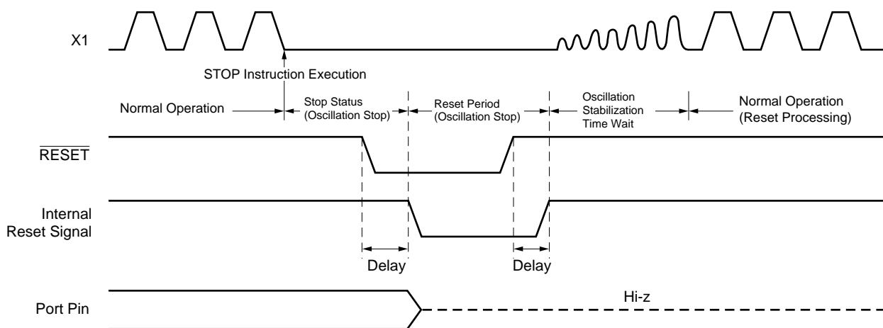
Figure 25-4. Timing of Reset by \overline{\text{RESET}} Input in STOP Mode
