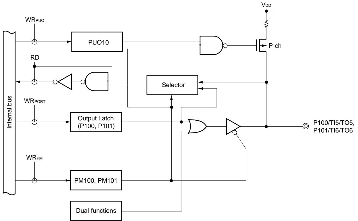
Figure 6-20. Block Diagram of P100 and P101
