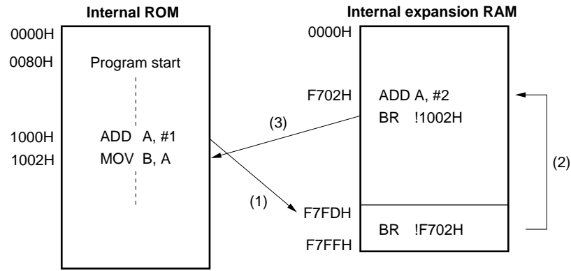
Figure 26-8. ROM Correction Example
