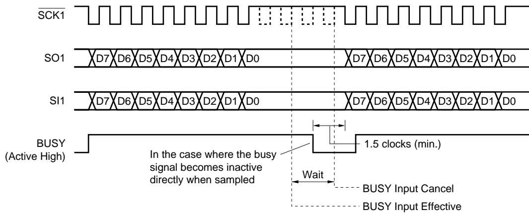
Figure 19-20. Busy Signal and Wait Cancel (BUSY0 = 0)
