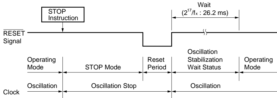
Figure 24-5. STOP Mode Released by \overline{\text{RESET}} Input
