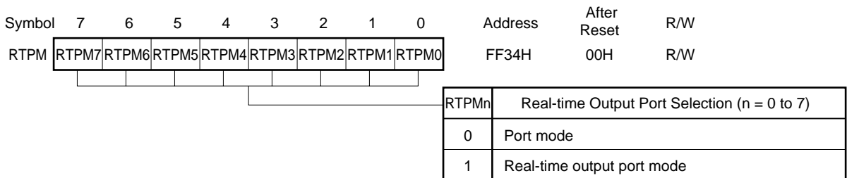
Figure 21-4. Real-time Output Port Mode Register Format
