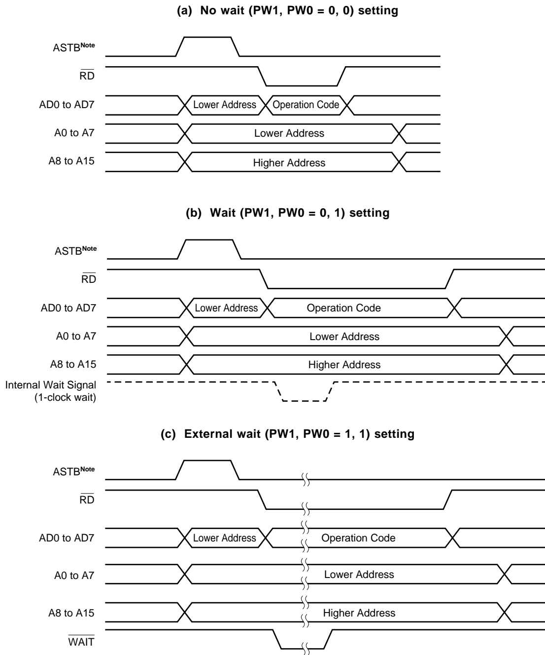
Figure 23-9. Instruction Fetch from External Memory in Separate Bus Mode
