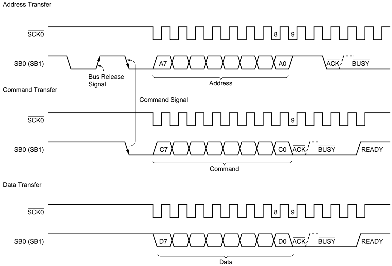
Figure 17-11. SBI Transfer Timings
