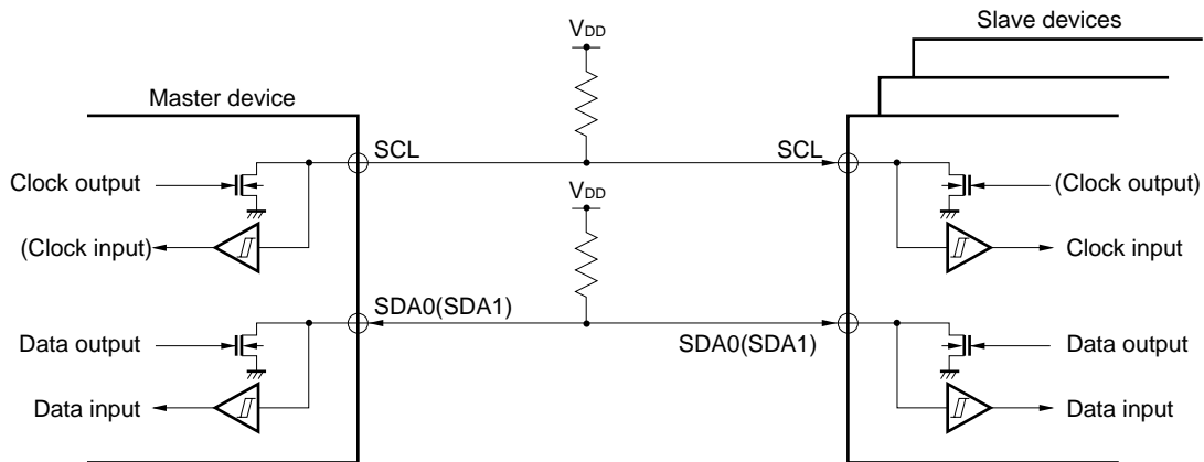
Figure 18-21. Pin Configuration
