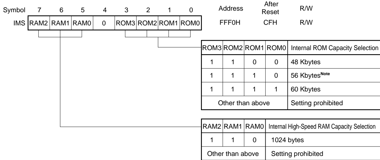
Figure 27-1. Internal Memory Size Switching Register Format
