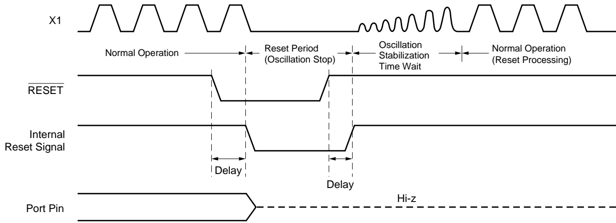
Figure 25-2. Timing of Reset by \overline{\text{RESET}} Input
