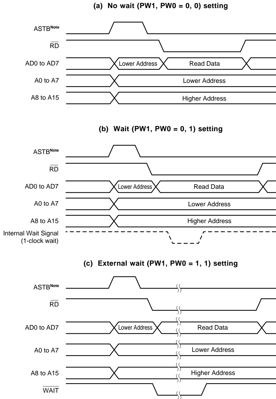
Figure 23-10. External Memory Read Timing in Separate Bus Mode
