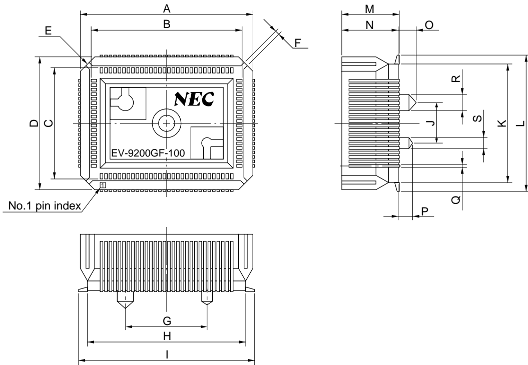
Figure B-3. EV-9200GF-100 Drawing (For Reference Only)
