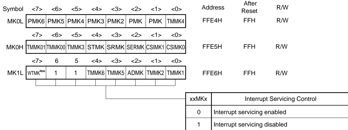
Figure 22-3. Interrupt Mask Flag Register Format
