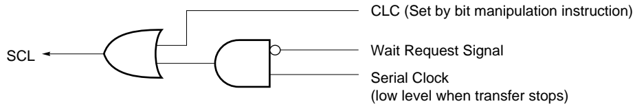
Figure 18-29. Logic Circuit of SCL Signal
