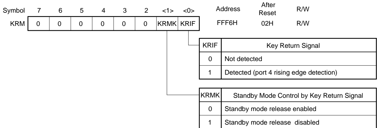
Figure 22-21. Key Return Mode Register Format
