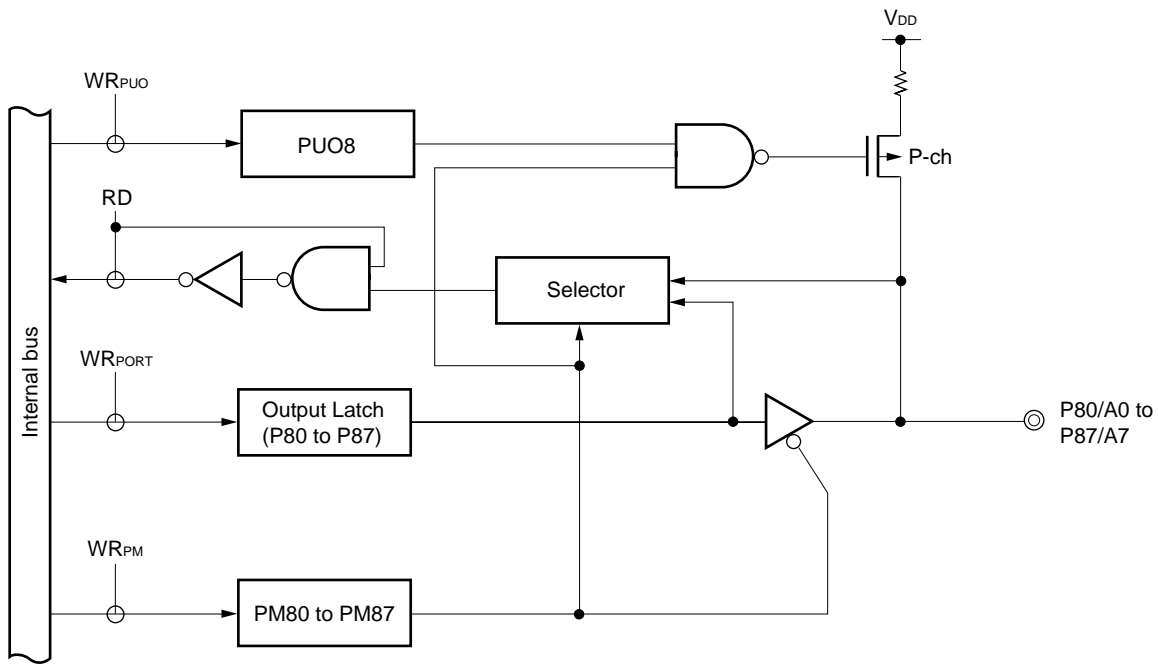
Figure 6-17. Block Diagram of P80 to P87
