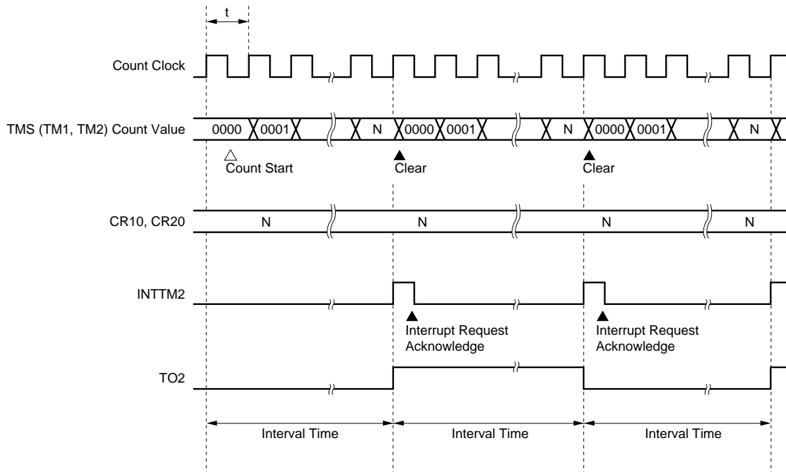
Figure 9-11. Interval Timer Operation Timing
