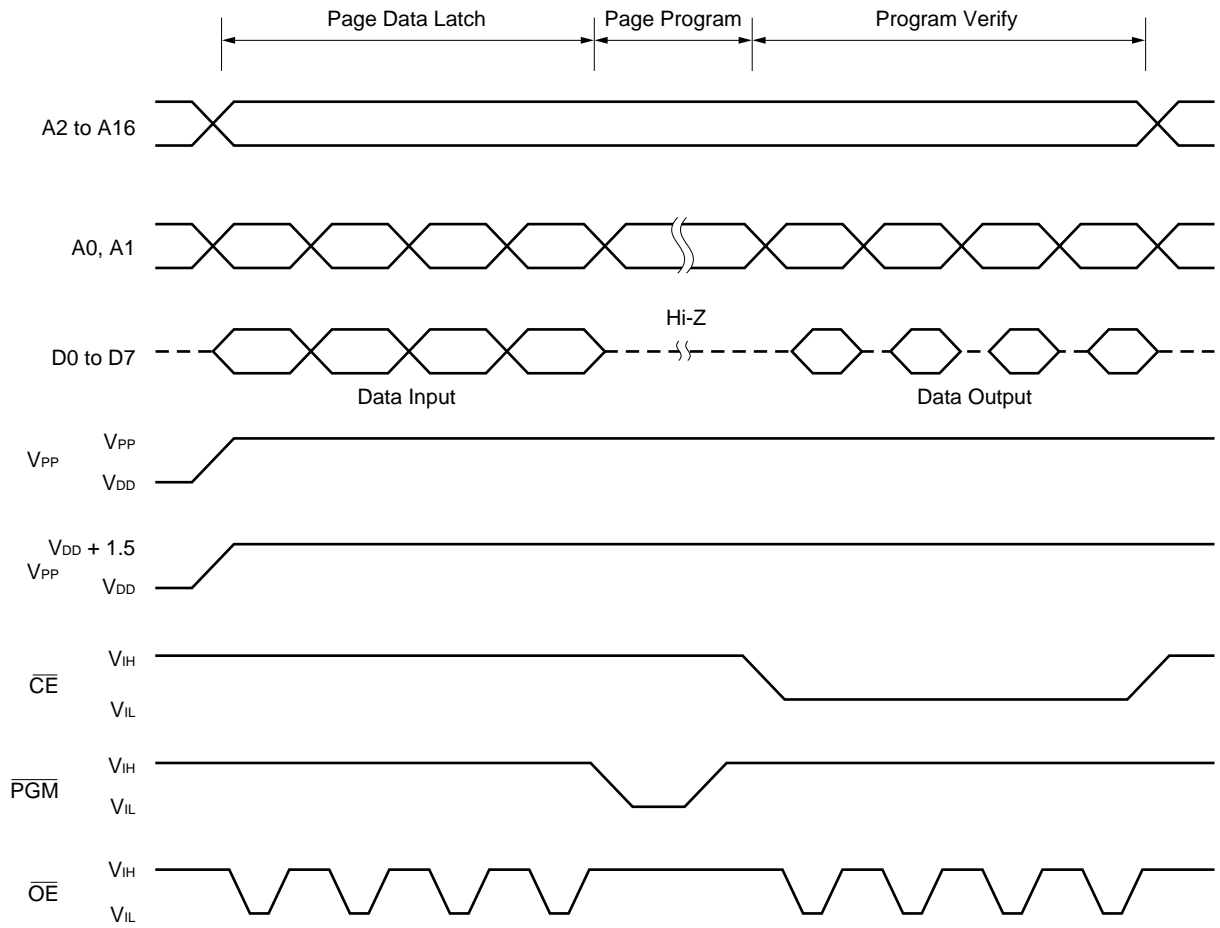
Figure 27-4. Page Program Mode Timing
