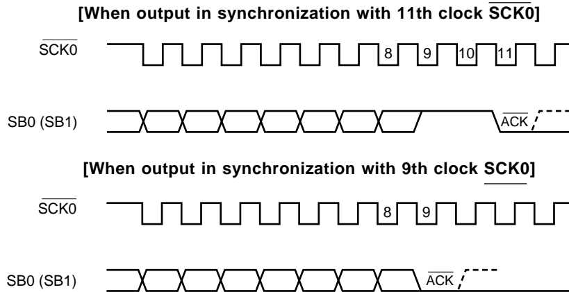
Figure 17-18. Acknowledge Signal
