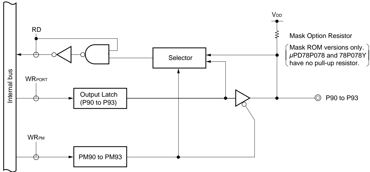
Figure 6-18. Block Diagram of P90 to P93
