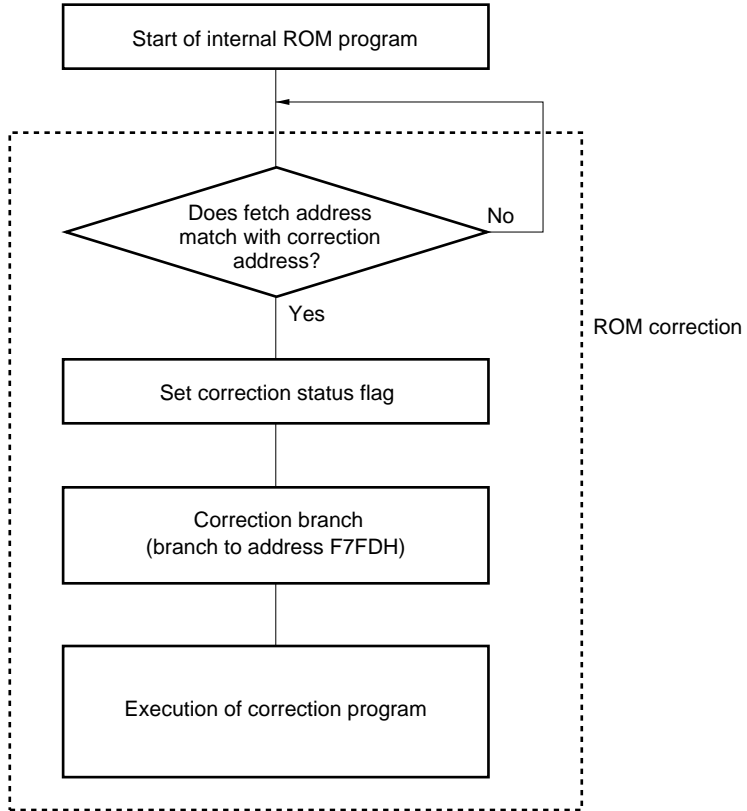
Figure 26-7. ROM Correction Operation
