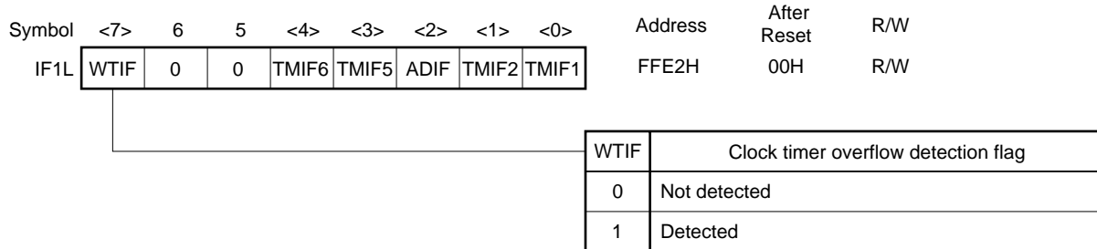
Figure 22-19. Format of Interrupt Request Flag Register 1L
