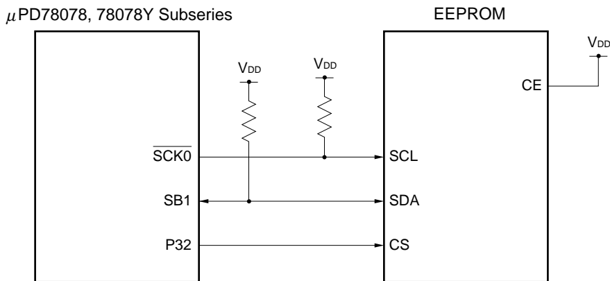
Figure 26-5. Connecting Example with EEPROM (Using 2-Wire Serial I/O Mode)
