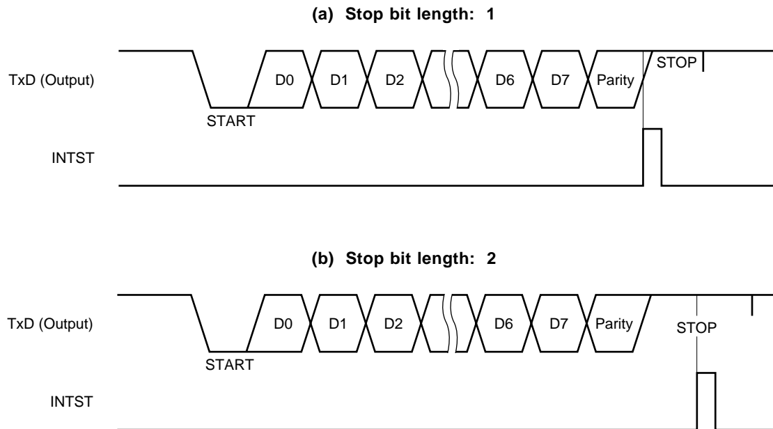
Figure 20-8. Asynchronous Serial Interface Transmission Completion Interrupt Request Generation Timing
