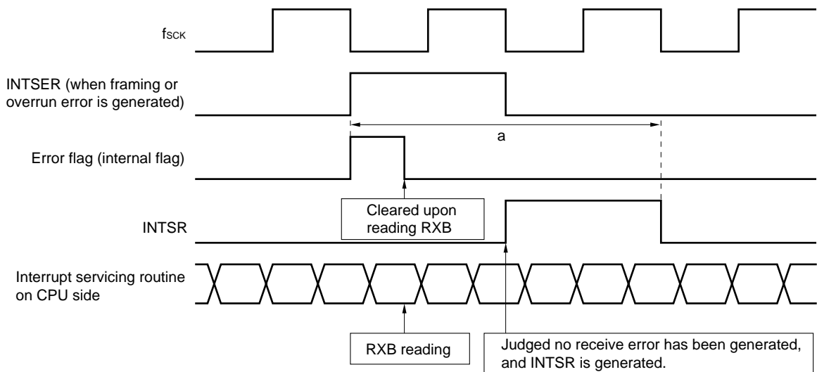
Figure 20-14. Receive Completion Interrupt Request Generation Timing (ISRM = 1)
