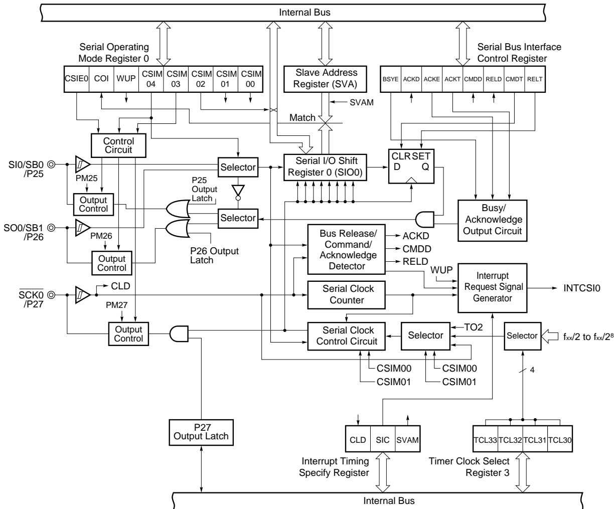
Figure 17-2. Serial Interface Channel 0 Block Diagram
