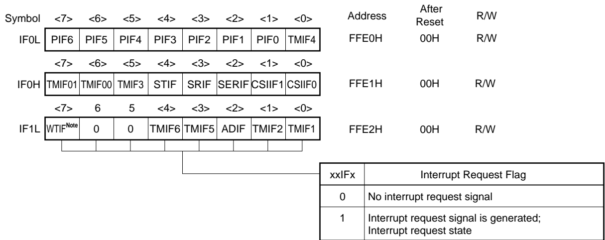
Figure 22-2. Interrupt Request Flag Register Format
