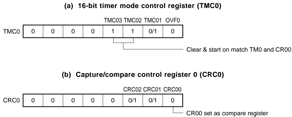
Figure 8-10. Control Register Settings for Interval Timer Operation
