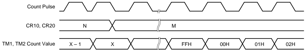
Figure 9-15. Timing after Compare Register Change during Timer Count Operation
