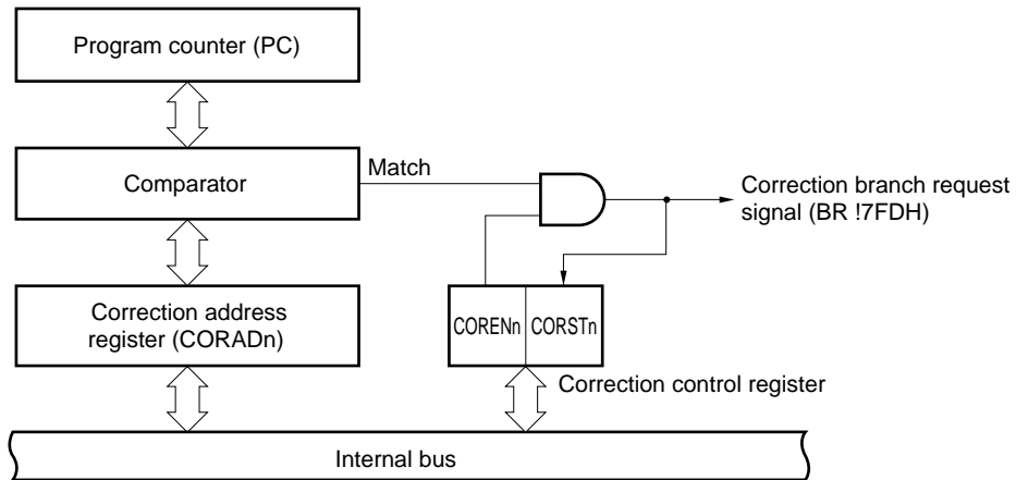
Figure 26-1. Block Diagram of ROM Correction
