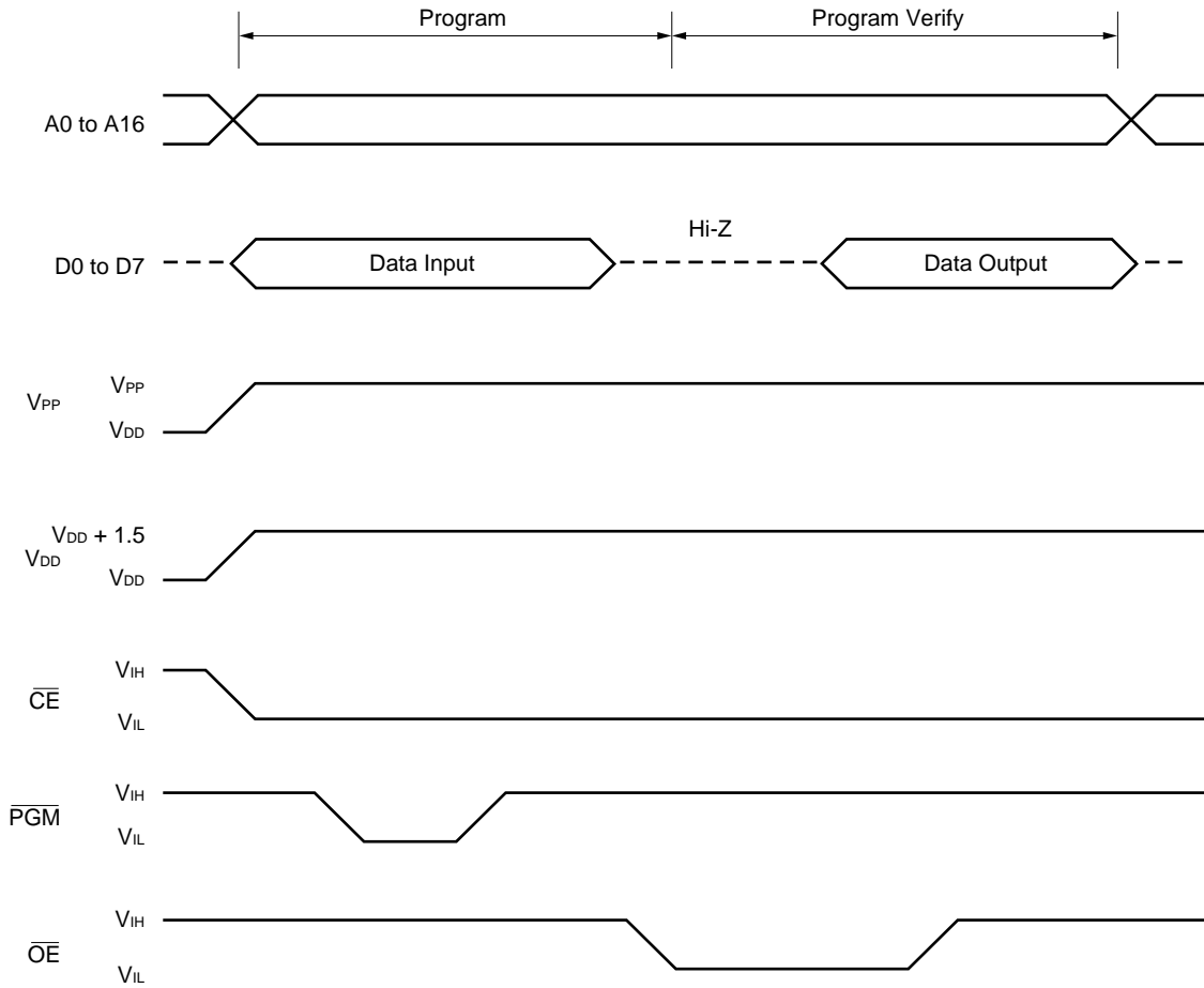
Figure 27-6. Byte Program Mode Timing
