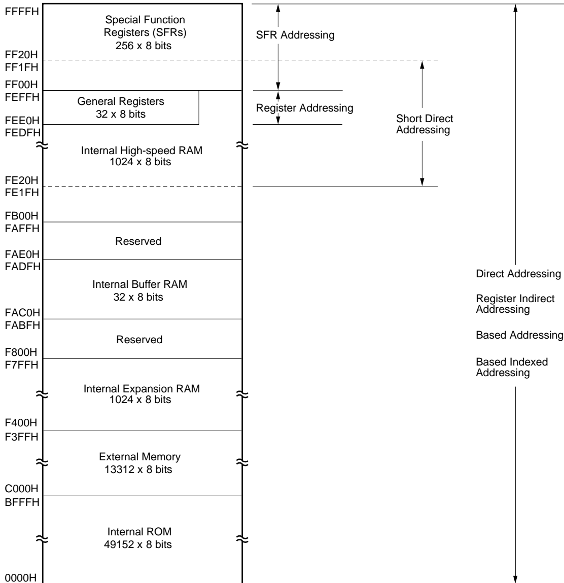
Figure 5-4. Data Memory Addressing ( \mu PD78076, 78076Y)
