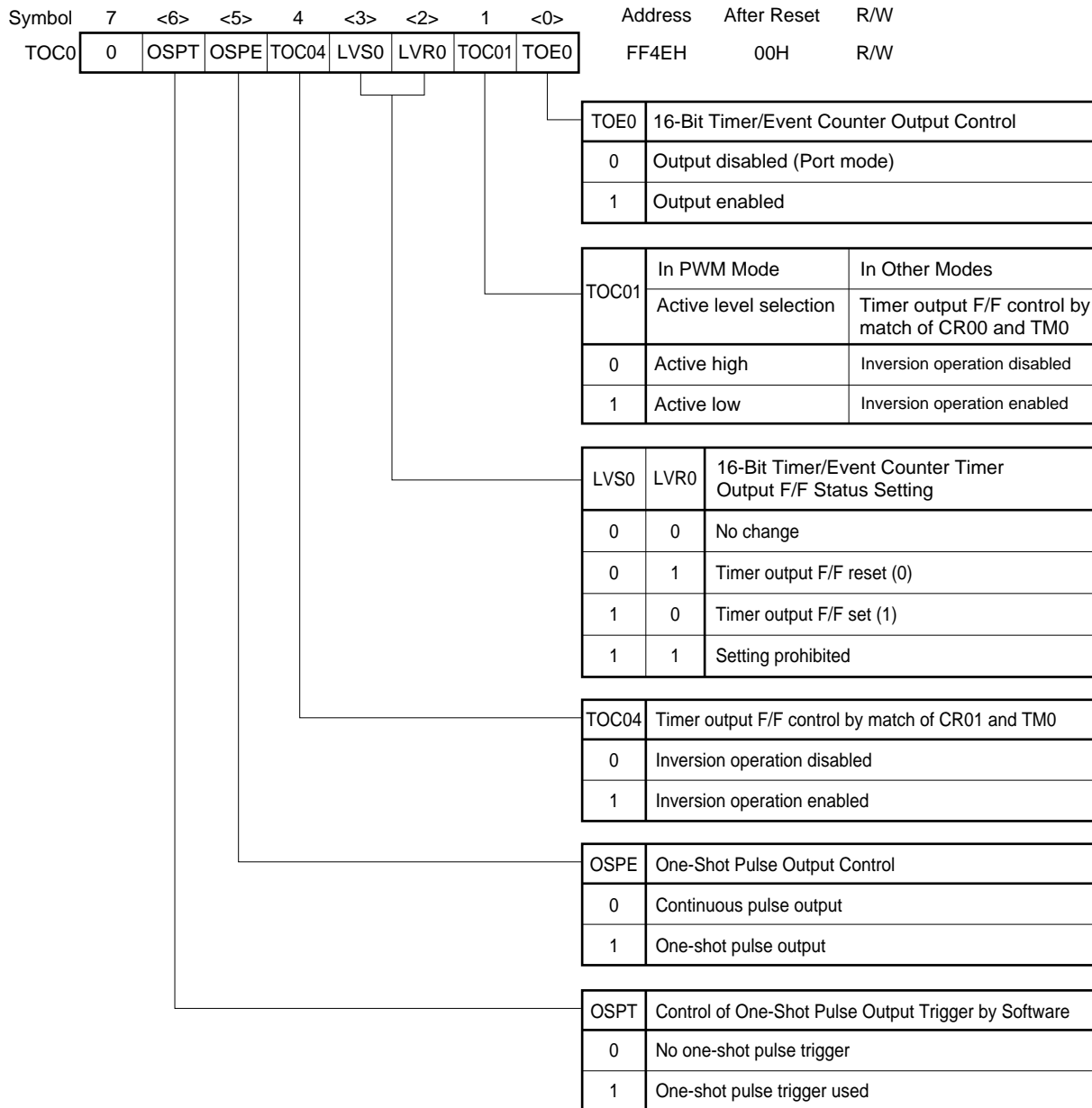
Figure 8-6. 16-Bit Timer Output Control Register Format
