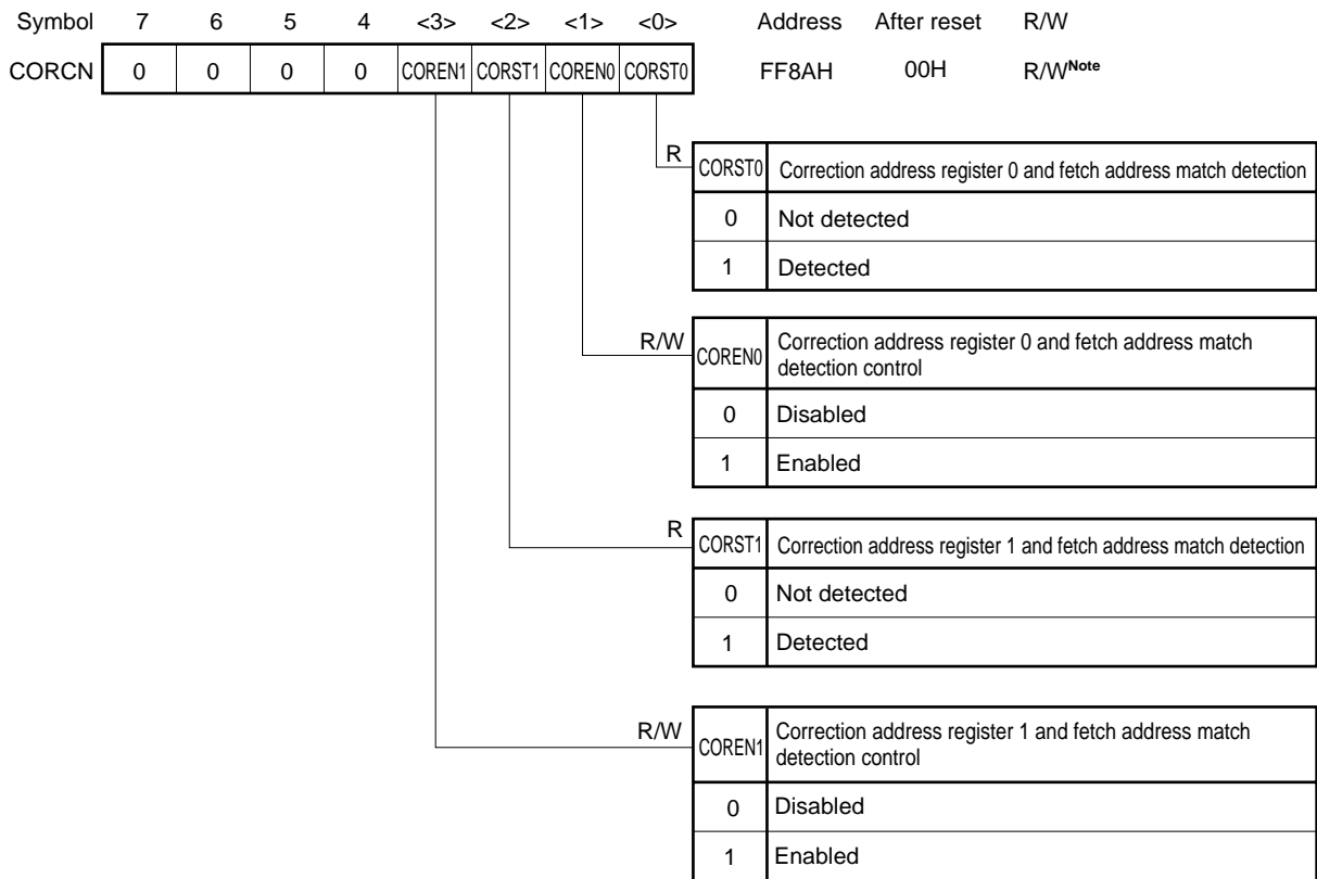
Figure 26-3. Correction Control Register Format
