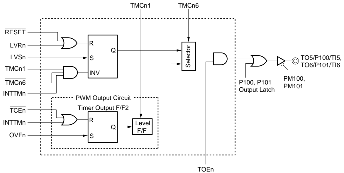
Figure 10-2. Block Diagram of 8-Bit Timer/Event Counters 5 and 6 Output Control Circuit
