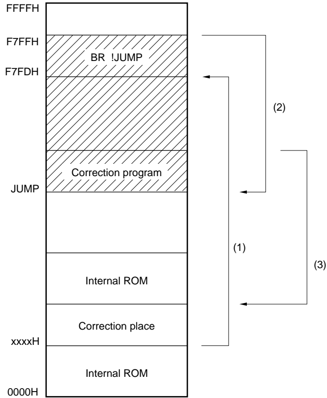
Figure 26-9. Program Transition Diagram (when One Place is Corrected)
