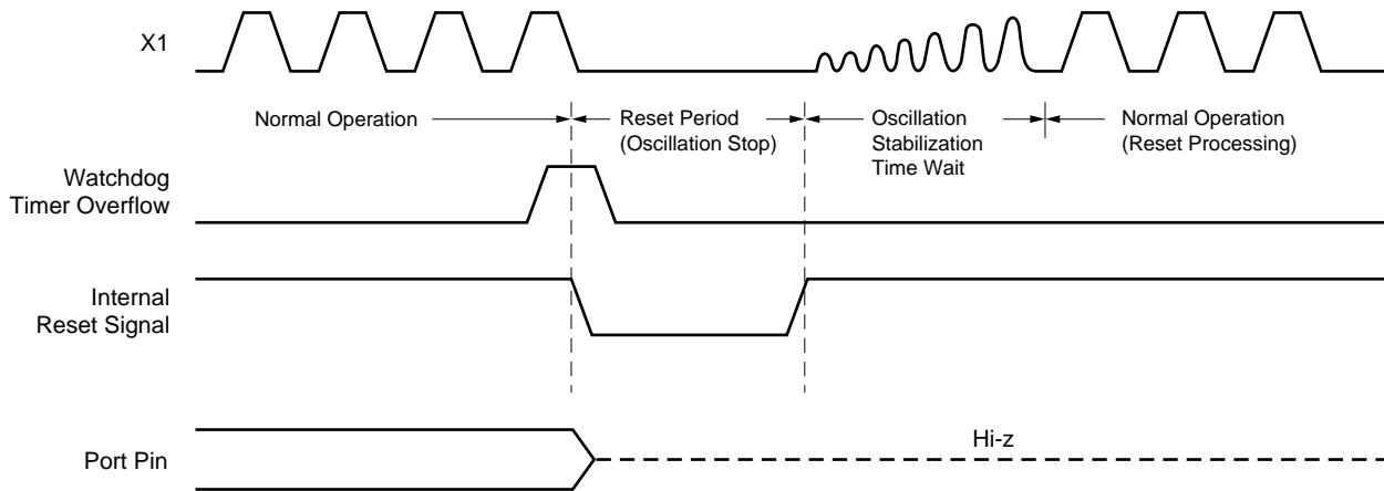
Figure 25-3. Timing of Reset due to Watchdog Timer Overflow
