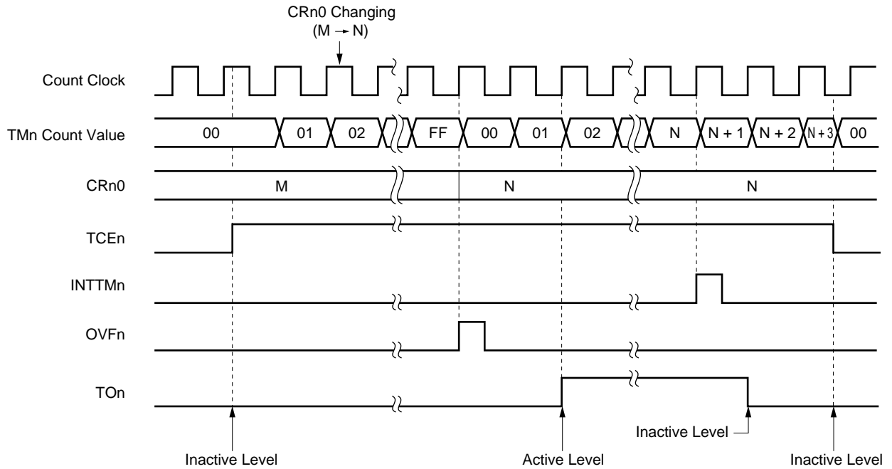
Figure 10-15. PWM Output Operation Timing (Active High Setting)
