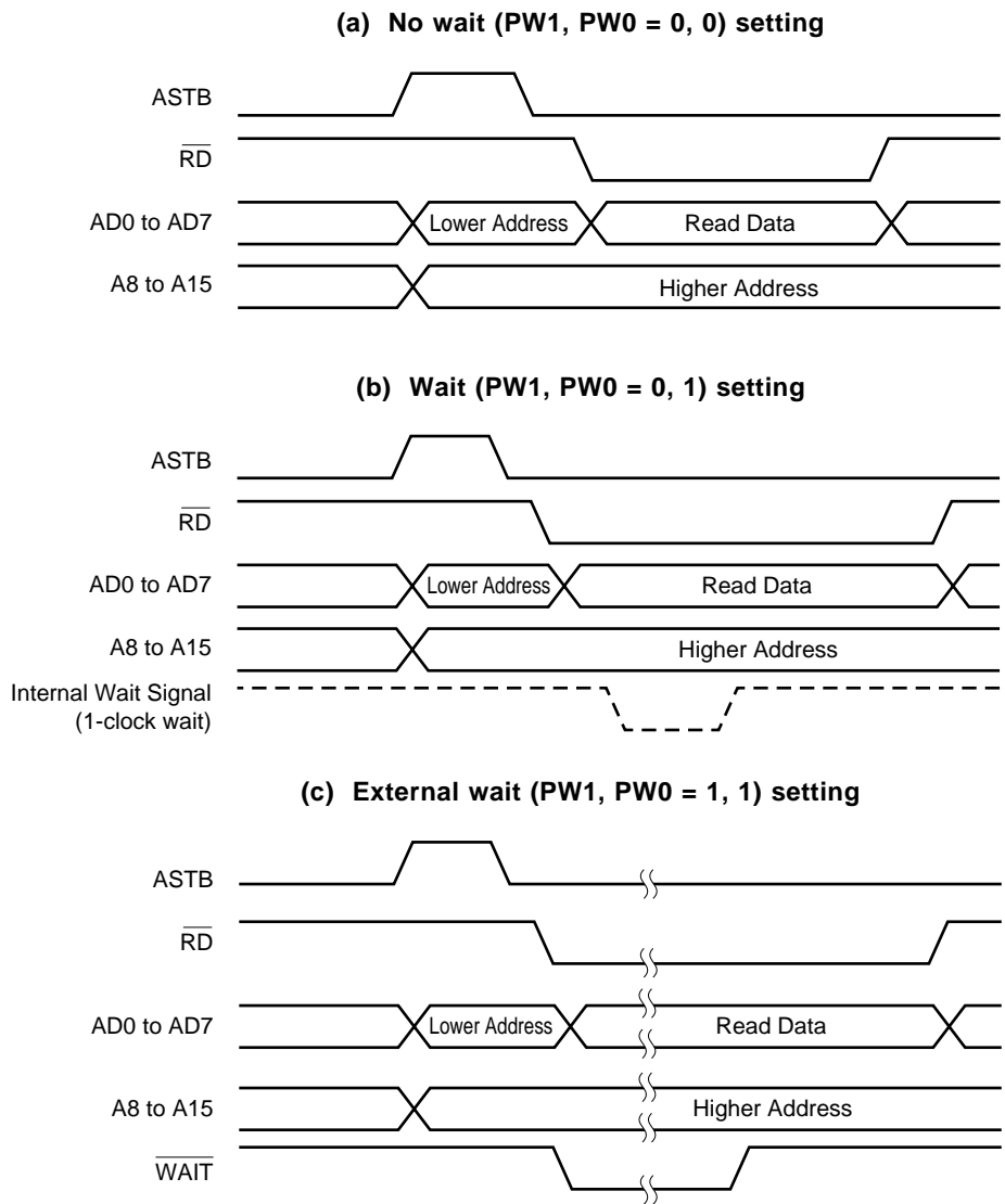
Figure 23-6. External Memory Read Timing in Multiplexed Bus Mode
