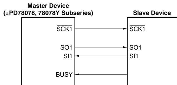
Figure 19-18. System Configuration when the Busy Control Option is Used
