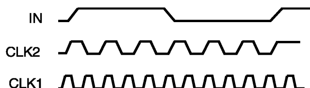
Input and Output Clock Waveforms with CLK2 Connected to FBIN
