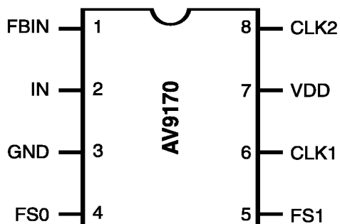
8-Pin DIP or SOIC
