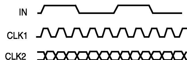
Input and Output Clock Waveforms with CLK1 Connected to FBIN
