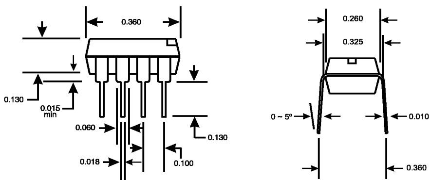
8-Pin DIP PACKAGE
