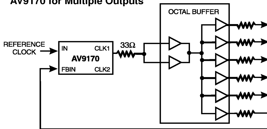
Figure 1: Application of AV9170 for Multiple Outputs
