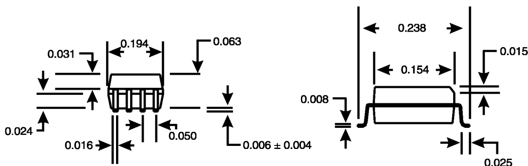
8-Pin SOIC PACKAGE
