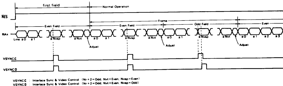
Figure 45 RES Release Sequence in The Interlace Mode (2)
