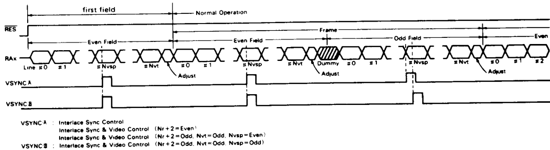
Figure 44 RES Release Sequence in The Interlace Mode (1)
