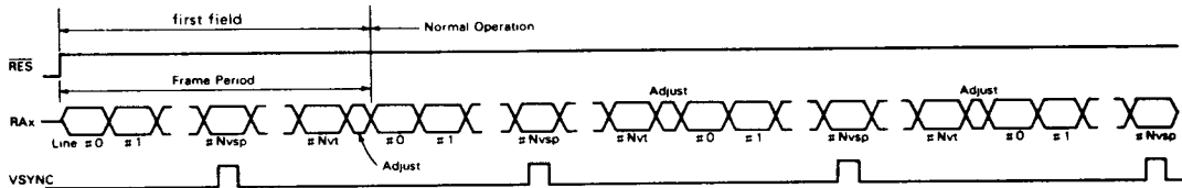
Figure 43 RES Release Sequence in The Non-interlace Mode
