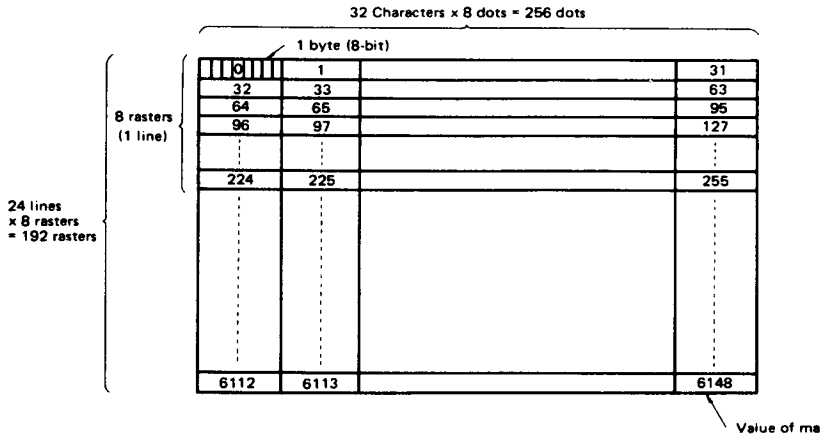
Figure 37 Memory Address and Dot Display Position on the Screen for Full Graphic Display
