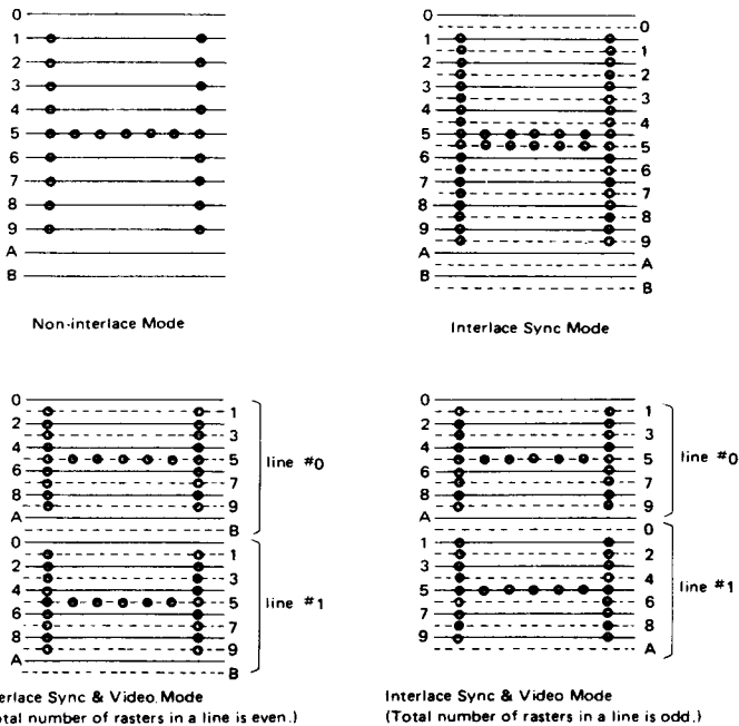
Figure 8 Example of Raster Scan Display
