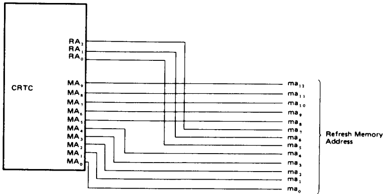
Figure 36 Refresh Memory Address Method for Full Graphic Display
