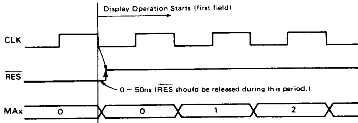
Figure 42 RES Release Sequence
