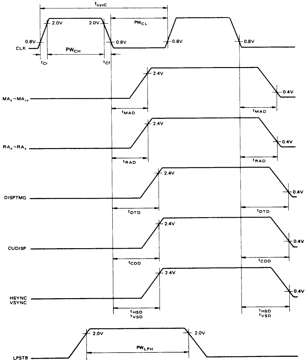
This Figure shows the relation in time between CLK signal and each output signals. Output sequence is shown in Figs. 10~15.
