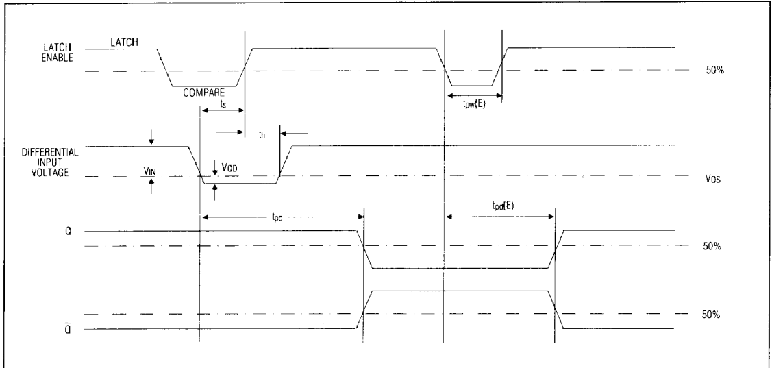
MAX9686 and MAX9698 Timing Diagram
