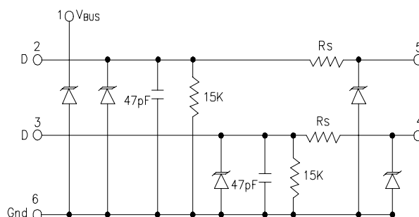
Figure 1 - STF201 Circuit Diagram
