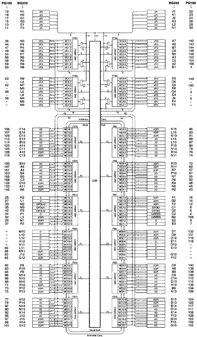
Figure 2: XC73144 Architecture
