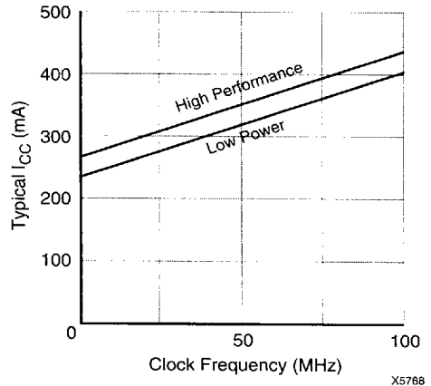
Figure 1: Typical I CC vs. Frequency for XC73144
