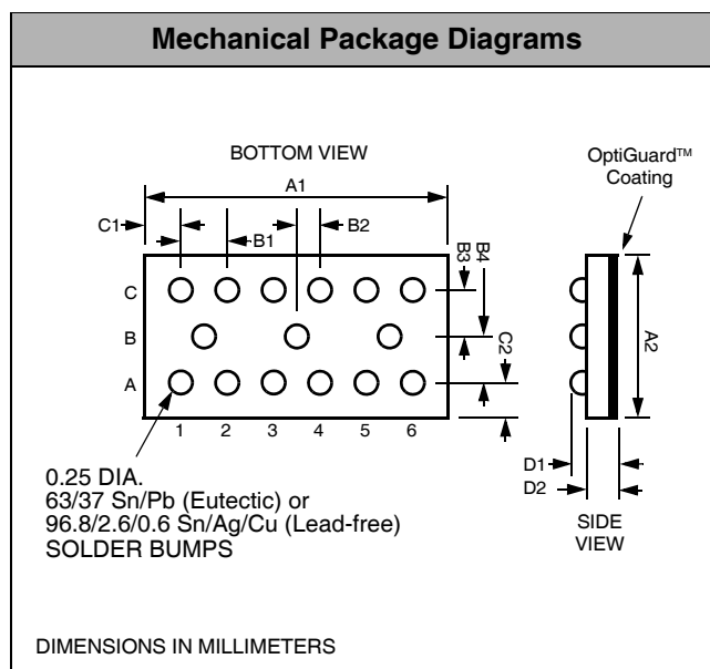
Package Dimensions for CM1440 Chip Scale Package
