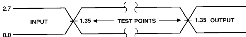
Fig. 7 Transient Input/Output Reference Waveform for V_{CC} = 2.7 to 3.6\text{ V}
