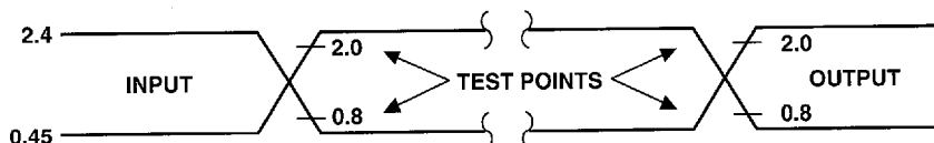
Fig. 8 Transient Input/Output Reference Waveform for V_{CC} = 3.3 \pm 0.3\text{ V} and V_{CC} = 5.0 \pm 0.25\text{ V} (High Speed Testing Configuration)
