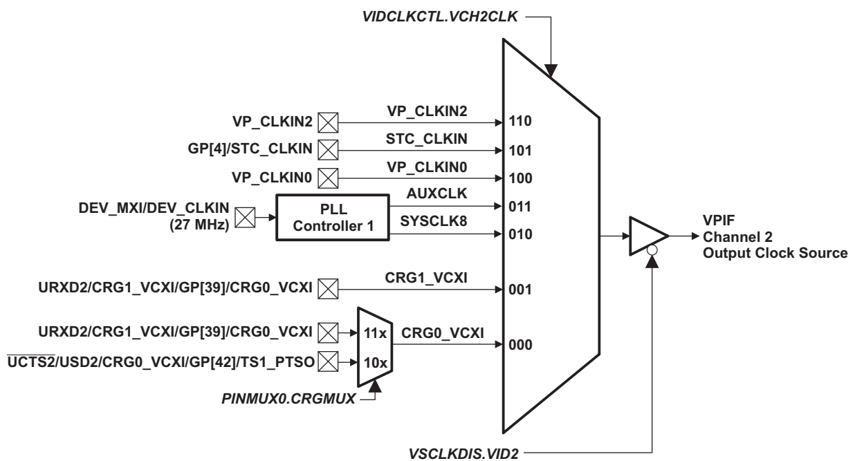
Figure 6-28. VPIF Display Channel 2 Source Clock Selection
