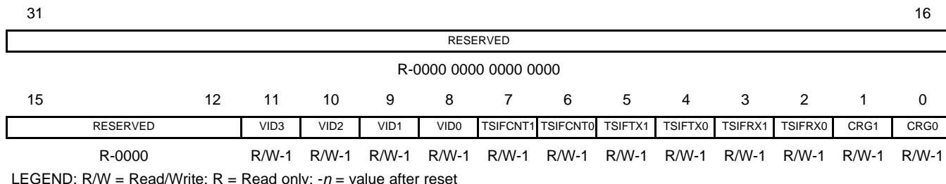
Figure 3-4. VSCLKDIS Register [0x01C4 006C]
