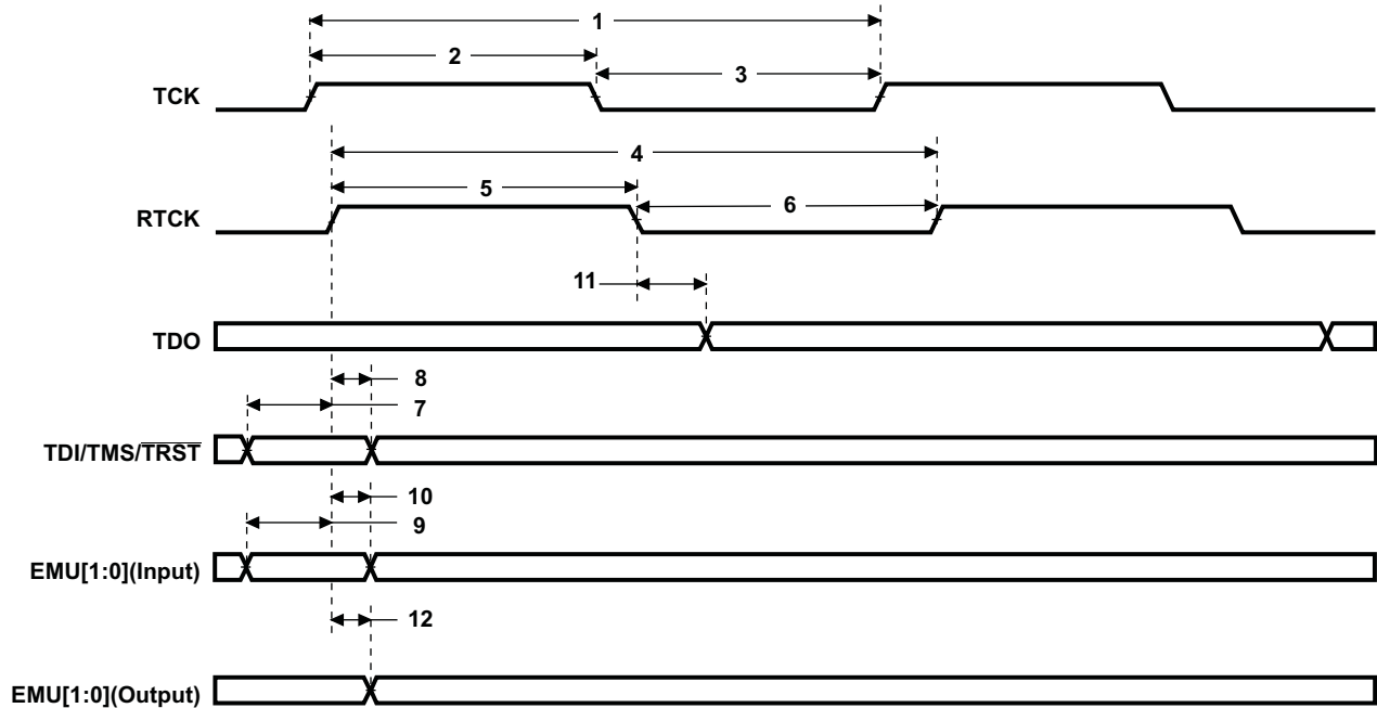
Figure 6-88. JTAG Test-Port Timing
