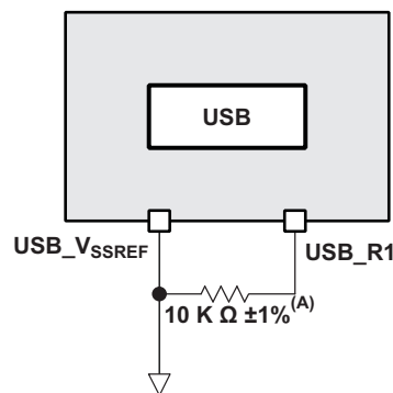
Figure 6-55. USB Reference Resistor Routing
