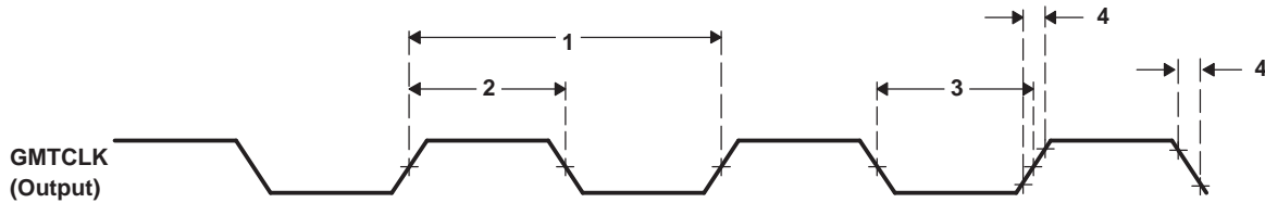
Figure 6-44. GMTCLK Timing (EMAC – Transmit) [GMII Operation]
