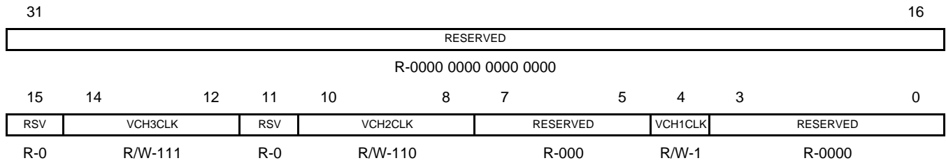
Figure 3-2. VIDCLKCTL Register [0x01C4 0038]
