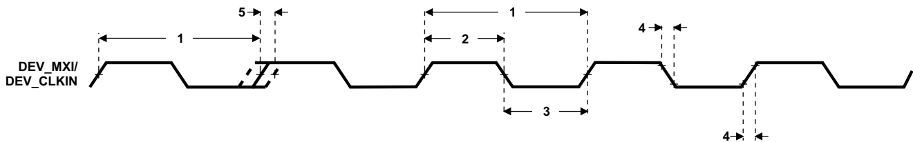
Figure 6-15. DEV_MXI/DEV_CLKIN Timing
