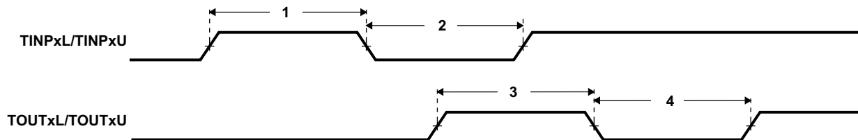
Figure 6-85. Timer Timing
