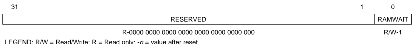
Figure 3-10. ARMWAIT Register
