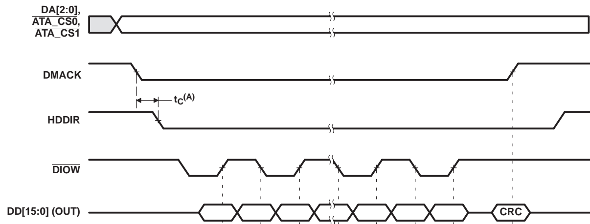
Figure 6-70. ATA HDDIR Multiword DMA Write Transfer Timing
