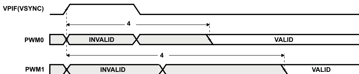
Figure 6-84. PWM Output Delay Timing
