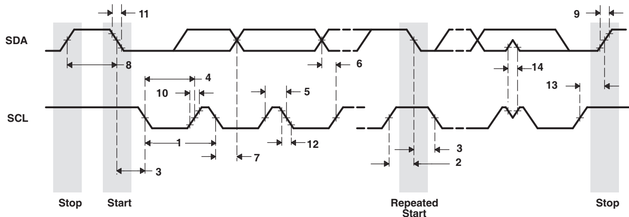
Figure 6-81. I2C Receive Timings
