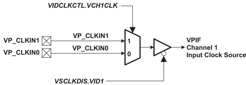
Figure 6-27. VPIF Capture Channel 1 Source Clock Selection
