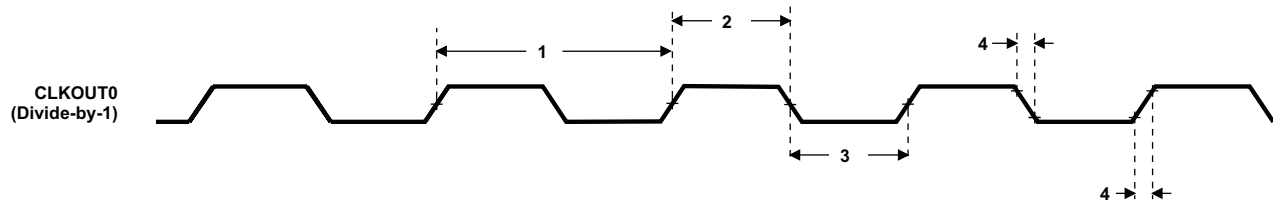
Figure 6-17. CLKOUT0 Timing
