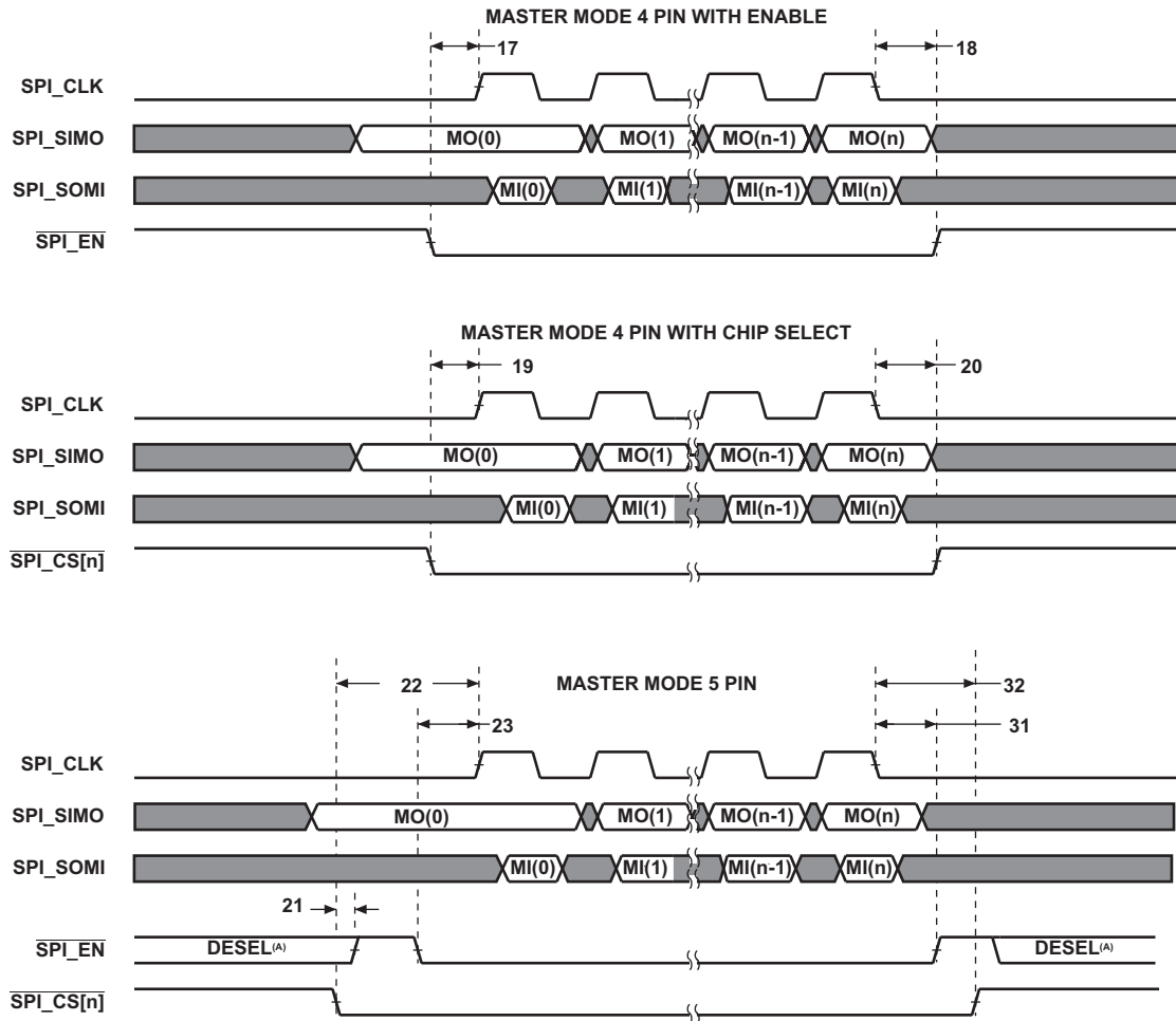
Figure 6-78. SPI Timings—Master Mode (4-Pin and 5-Pin)
