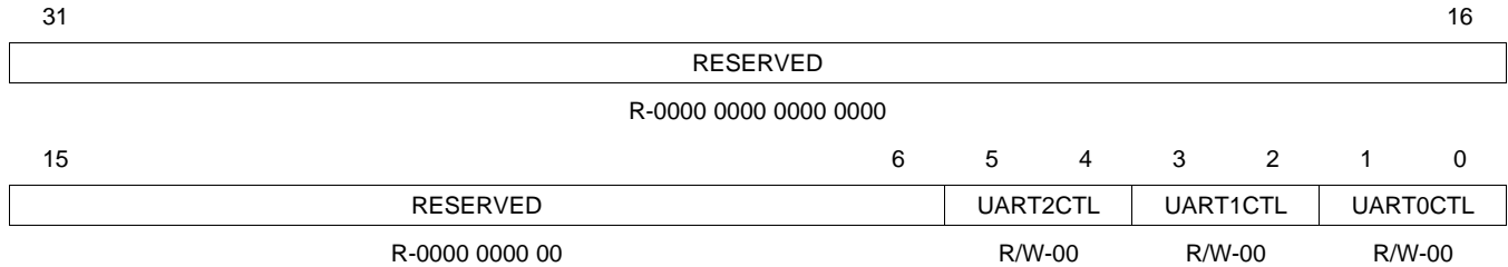
Figure 3-19. PINMUX1 Register
