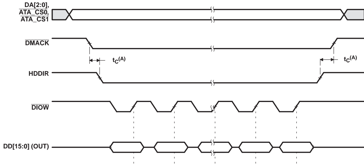
Figure 6-70. ATA HDDIR Multiword DMA Write Transfer Timing
