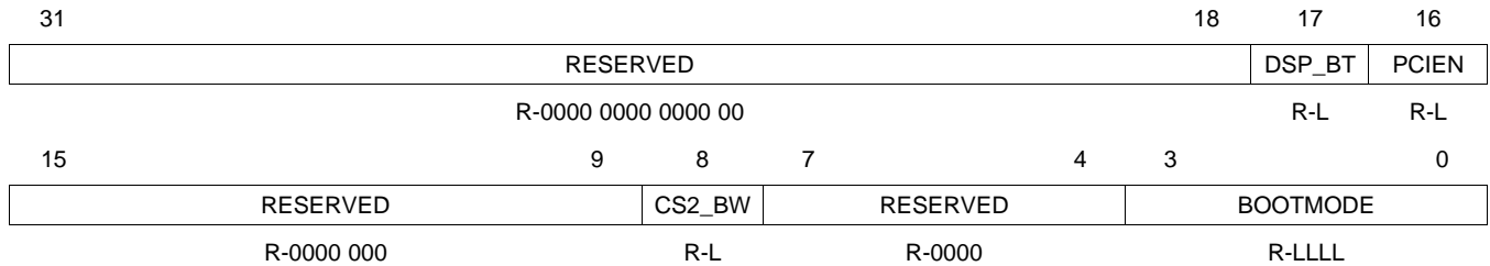
Figure 3-8. BOOTCFG Register
