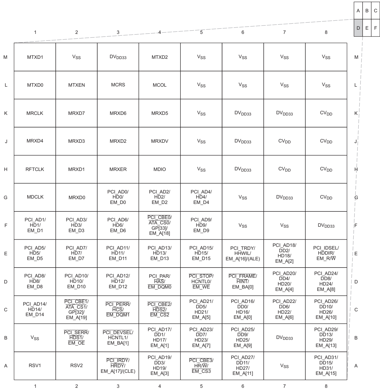
Figure 2-5. Pin Map [Section D]
