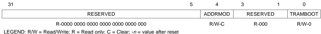
Figure 3-9. ARMBOOT Register
