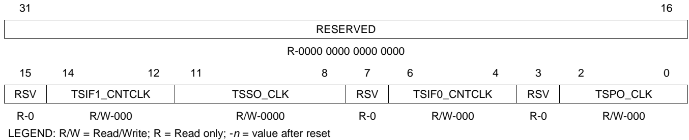
Figure 3-3. TSIFCTL Register [0x01C4 0050]
