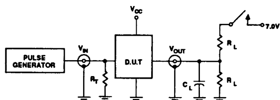
Test Circuit For Open Collector Outputs
