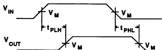
Waveform 1. Propagation Delay for Non-Inverting paths
