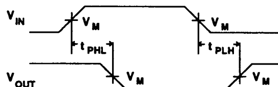
Waveform 2. Propagation Delay for Inverting paths
