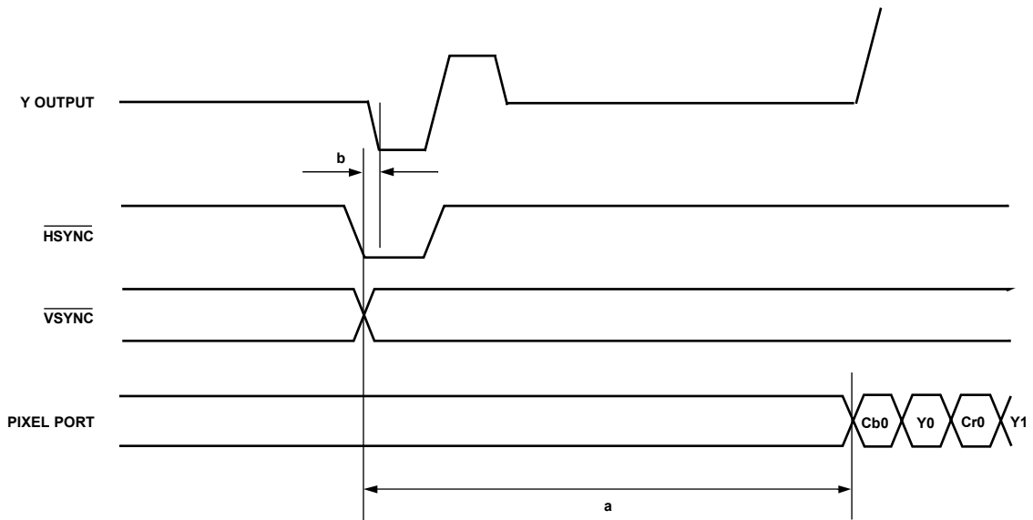
Figure 12. HD-SDR, 16-Bit 4:2:2 YCrCb ( \overline{\text{HSYNC}}/\overline{\text{VSYNC}} ) Input Timing Diagram
