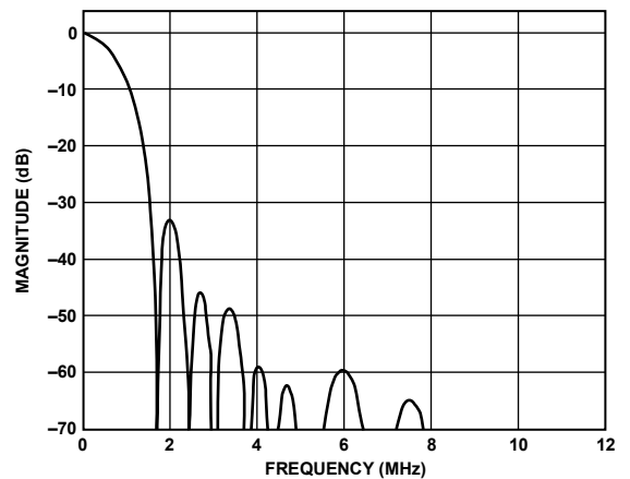
Figure 42. SD Chroma 0.65 MHz Low-Pass Filter Response
