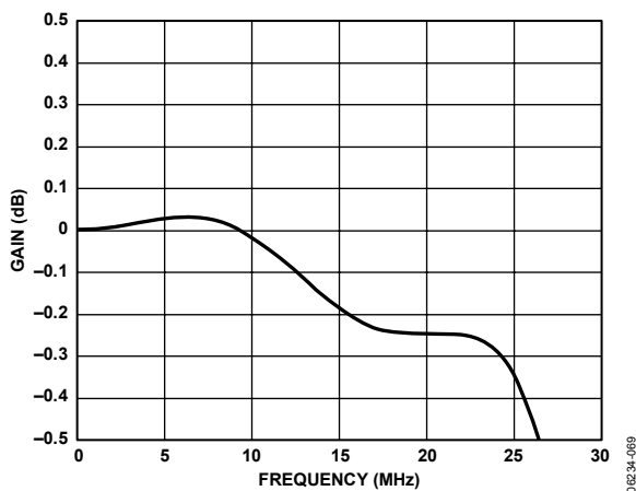
Figure 69. ED/HD Sinc Compensation Filter Disabled
