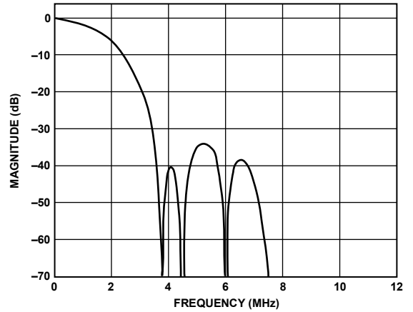
Figure 40. SD Chroma 1.3 MHz Low-Pass Filter Response
