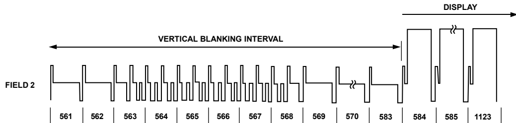
Figure 141. SMPTE 274M (1080i)
