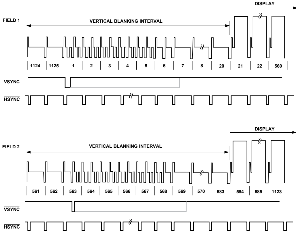
Figure 115. 1080i \overline{HSYNC} and \overline{VSYNC} Input Timing
