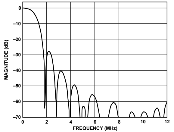
Figure 41. SD Chroma 1.0 MHz Low-Pass Filter Response
