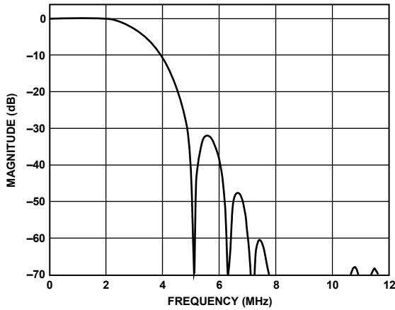
Figure 38. SD Chroma 3.0 MHz Low-Pass Filter Response
