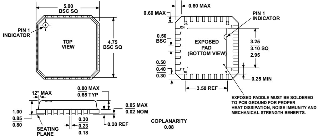
COMPLIANT TO JEDEC STANDARDS MO-220-VHHD-2 Figure 142. 32-Lead Lead Frame Chip Scale Package [LFCSP_VQ] 5 mm × 5 mm Body, Very Thin Quad (CP-32-2) Dimensions shown in millimeters
