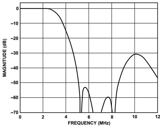
Figure 39. SD Chroma 2.0 MHz Low-Pass Filter Response
