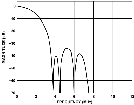
Figure 37. SD Luma QCIF Low-Pass Filter Response
