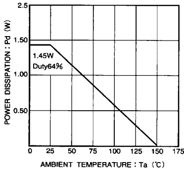
Fig. 3 Thermal reduction curve
