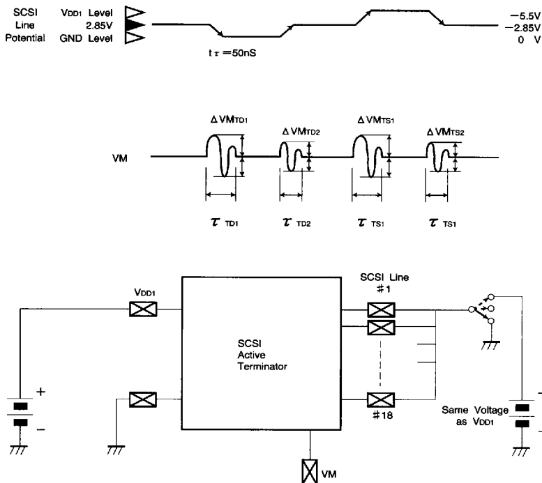
Fig. 1 Measurement of transient characteristics
