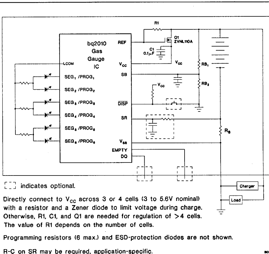
Figure 1. Battery Pack Application Diagram—LED Display
