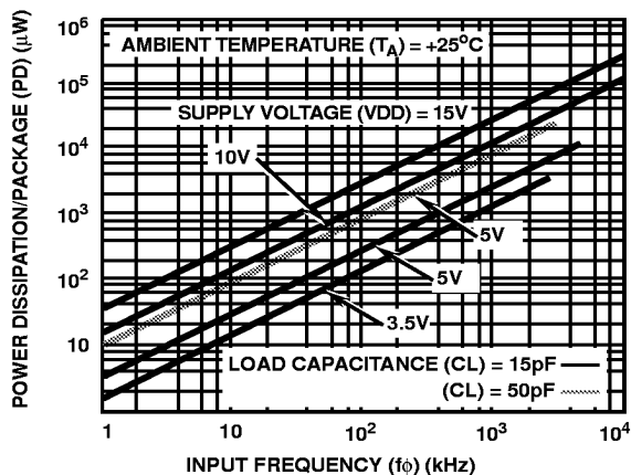
FIGURE 10. TYPICAL DISSIPATION CHARACTERISTICS
