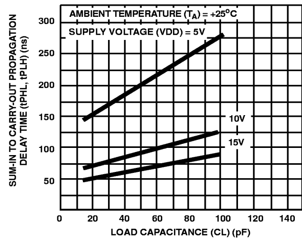
FIGURE 5. TYPICAL SUM-IN TO CARRY-OUT PROPAGATION DELAY TIME vs LOAD CAPACITANCE
