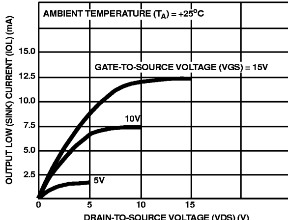
FIGURE 9. MINIMUM OUTPUT LOW (SINK) CURRENT CHARACTERISTICS
