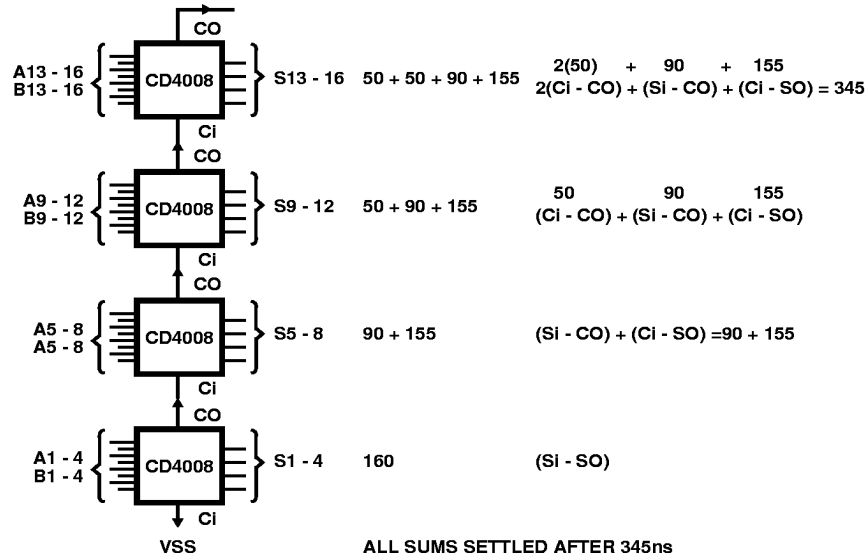
FIGURE 1. PROPAGATION DELAY FOR A 16 BIT ADDER (10V OPERATION)
