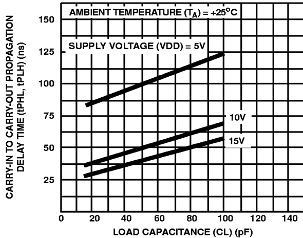
FIGURE 3. TYPICAL CARRY-IN TO CARRY-OUT PROPAGATION DELAY TIME vs LOAD CAPACITANCE
