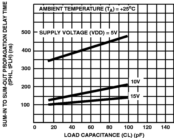
FIGURE 2. TYPICAL SUM-IN TO SUM-OUT PROPAGATION DELAY TIME vs LOAD CAPACITANCE
