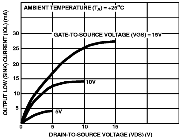
FIGURE 8. TYPICAL OUTPUT LOW (SINK) CURRENT CHARACTERISTICS
