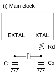
Fig. 10. Recommended oscillation circuit
