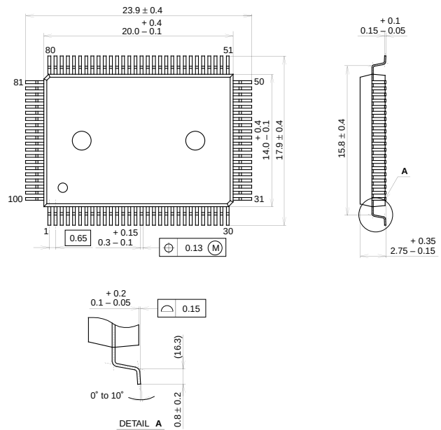
PACKAGE STRUCTURE
