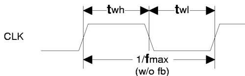
Clock Width
