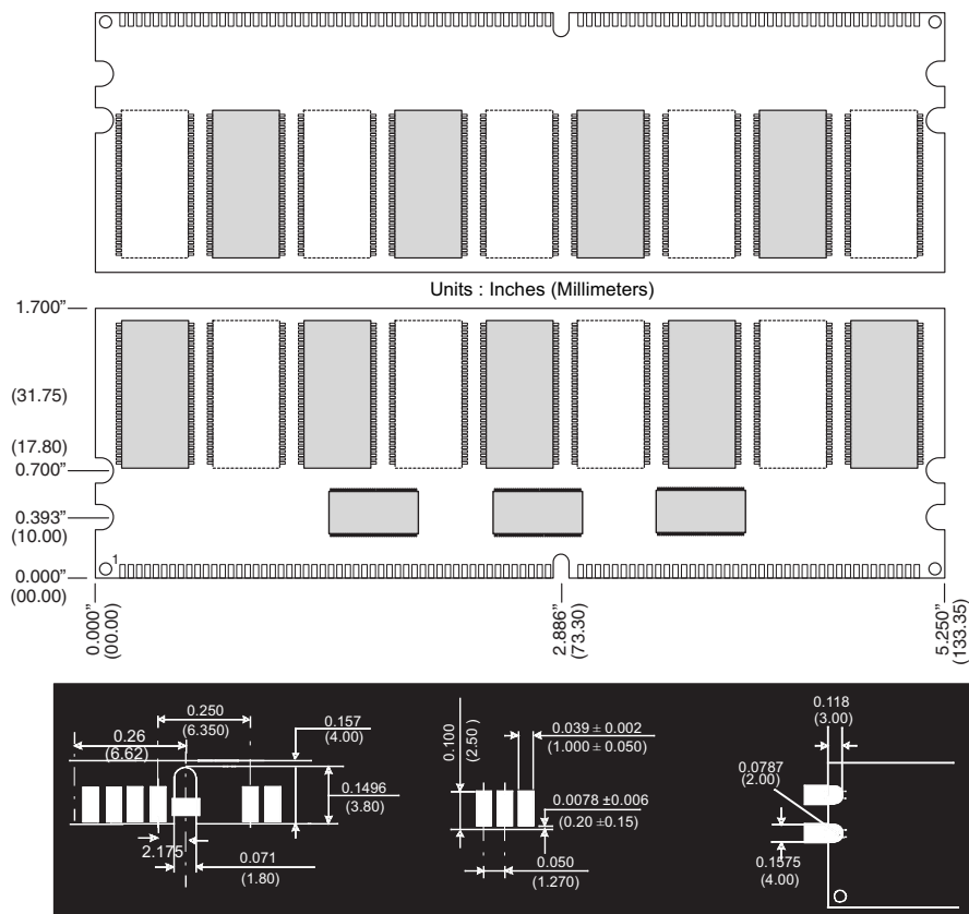
Figure 1: KVR266X72C25/128 184-Pin DDR SDRAM Module
