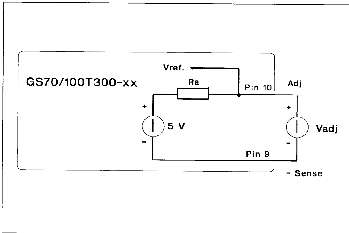
Figure 2. Output voltage adjustment
