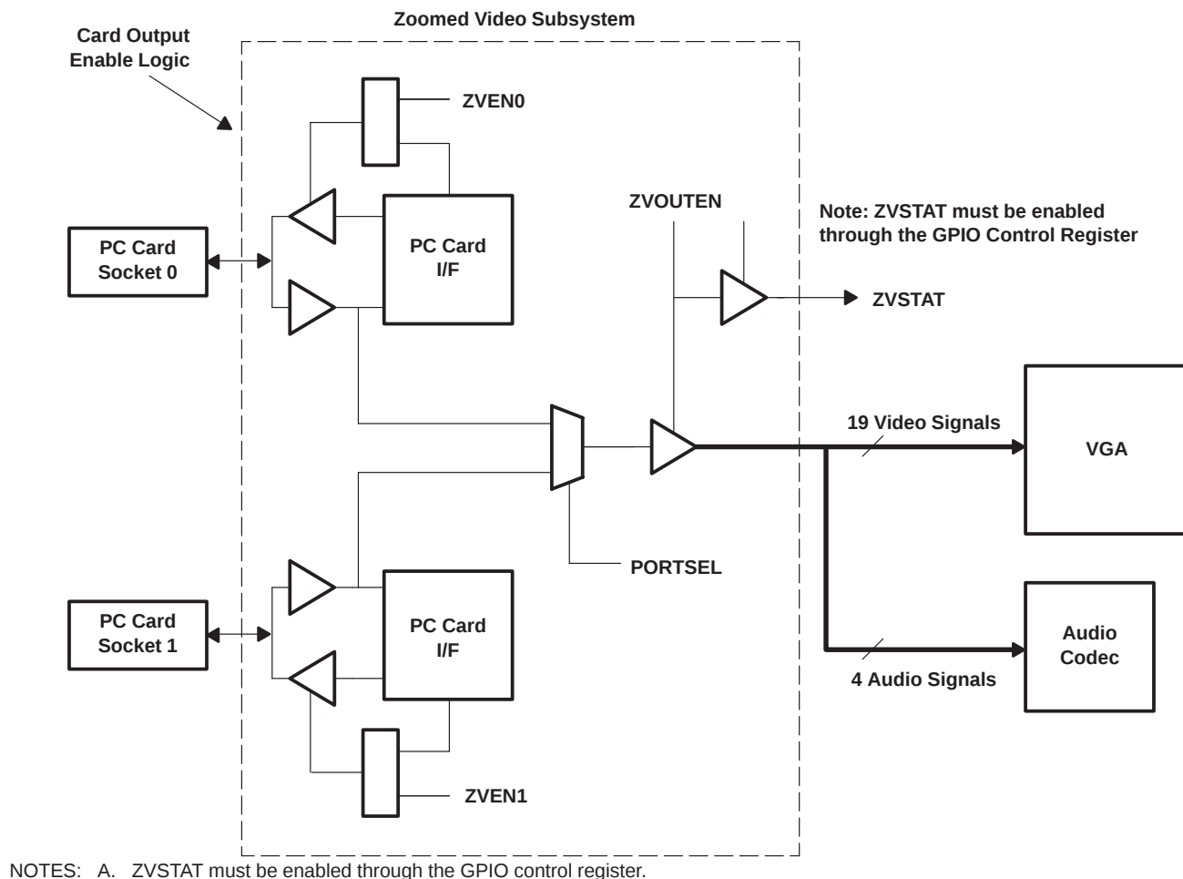
Figure 10. Zoomed Video Subsystem
