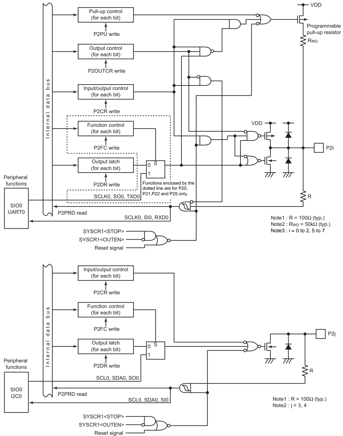
Figure 8-5 Port P2
