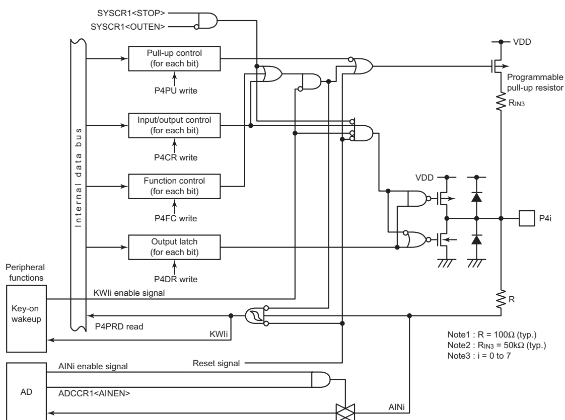
Figure 8-6 Port P4
