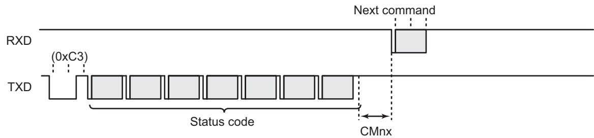
Figure 22-13 Flash Memory Status Output Command
