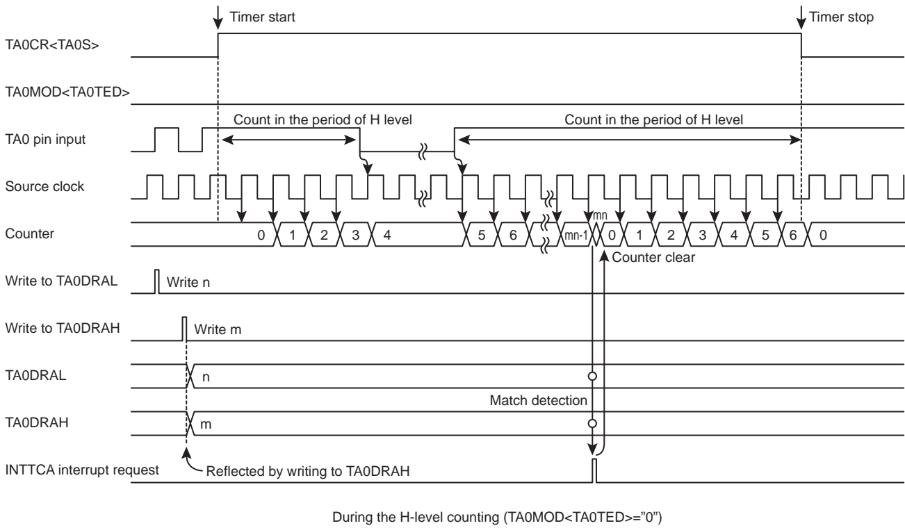
Figure 13-6 Window Mode Timing Chart
