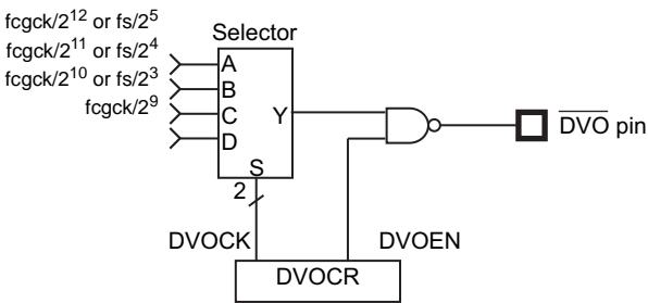
Figure 11-1 Divider Output
