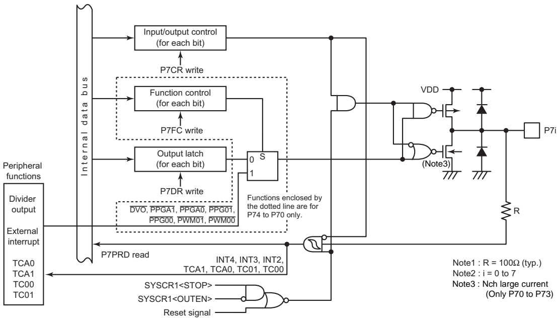
Figure 8-7 Port P7
