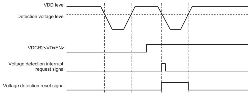
Figure 7-2 Voltage Detection Interrupt Request Signal and Voltage Detection Reset Signal
