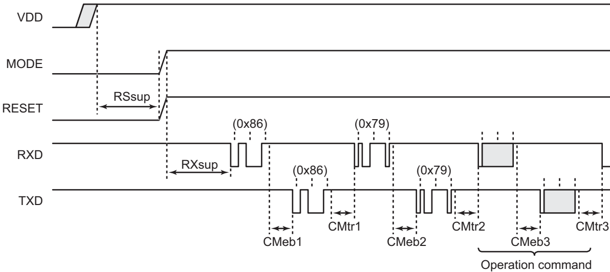
Figure 22-6 Reset Timing
