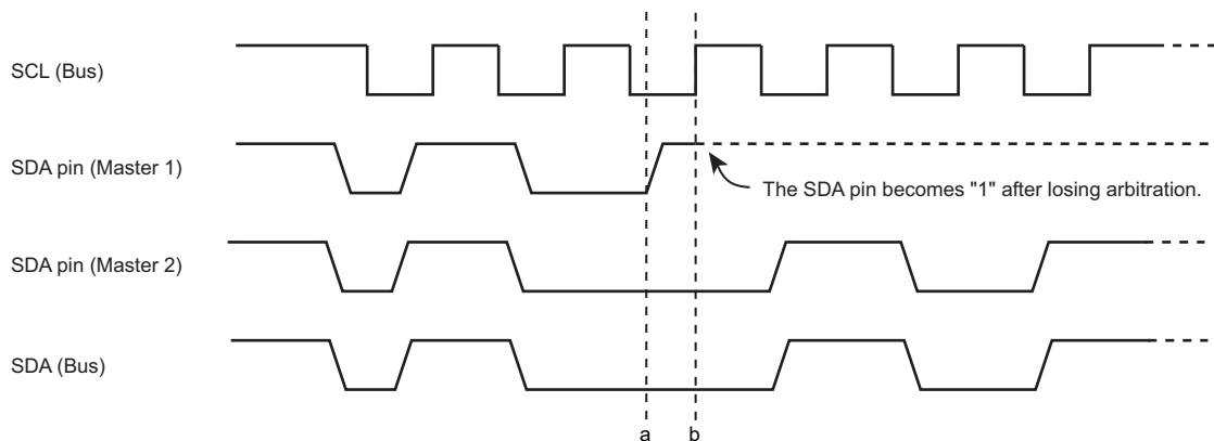
Figure 18-12 Arbitration Lost
