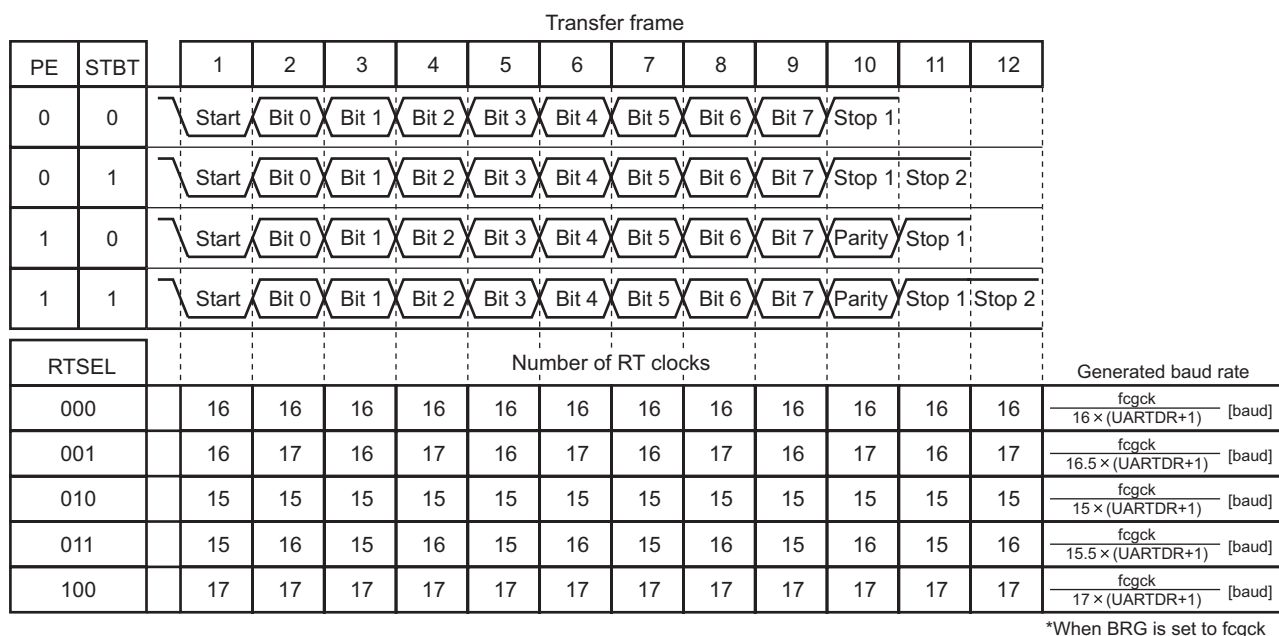
Figure 16-4 Fine Adjustment of Baud Rate Clock Using UART0CR2&lt;RTSEL&gt;
