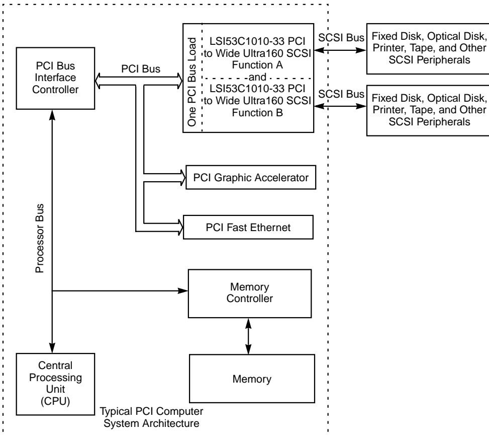
Figure 1.2 Typical LSI53C1010-33 System Application
