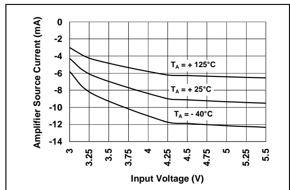
FIGURE 2-6: Error Amplifier Source Current vs. Input Voltage.
