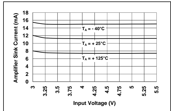
FIGURE 2-5: Error Amplifier Sink Current vs. Input Voltage.
