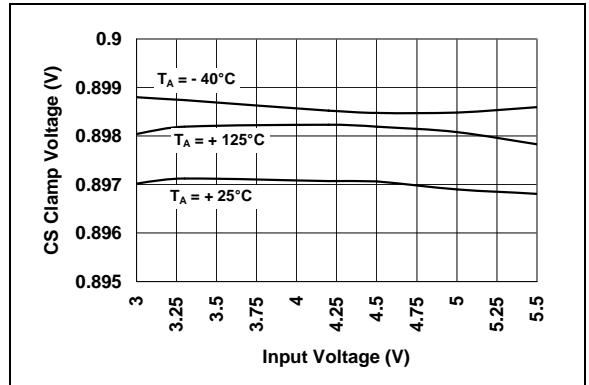
FIGURE 2-10: Current Sense Clamp Voltage vs. Input Voltage (MCP1630).
