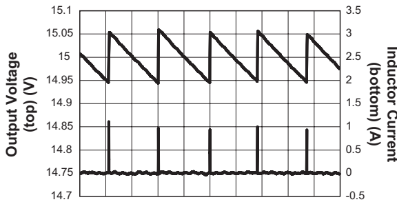
Output Ripple
