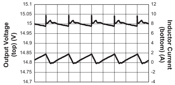
Output Ripple
