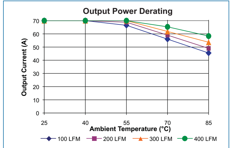
Figure 20 — Maximum output power derating vs ambient air temperature. Longitudinal airflow, Board and junction temperatures <125° C. Tested with IBC evaluation board IB050Q096T70N1-CB
