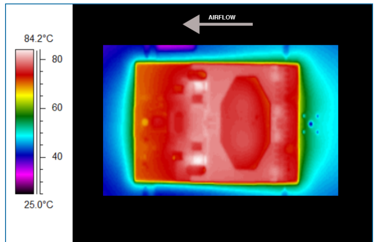
Figure 29 — Thermal plot, 600 LFM, 25°C, 48 Vin, 670 W output power
