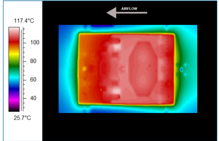
Figure 25 — Thermal plot, 200 LFM, 25°C, 48 Vin, 670 W output power
