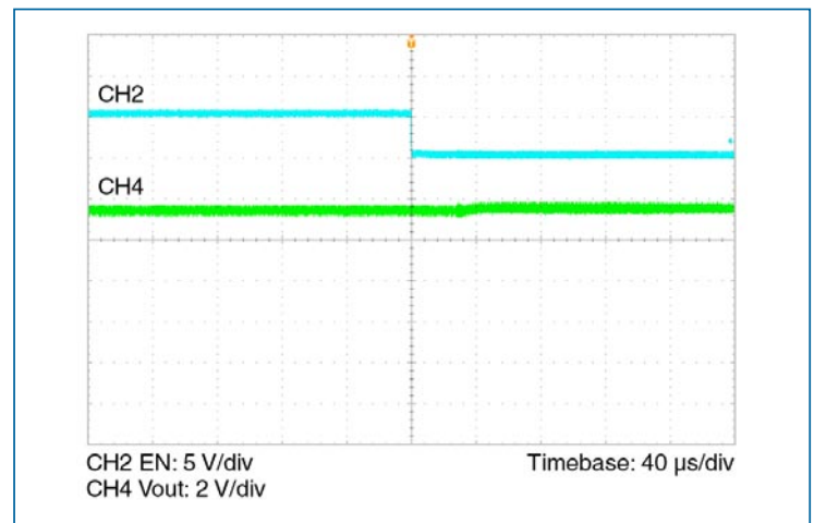
Figure 18 — Three module parallel array test. Vout change with two modules operating and a third module enabled. Nominal
