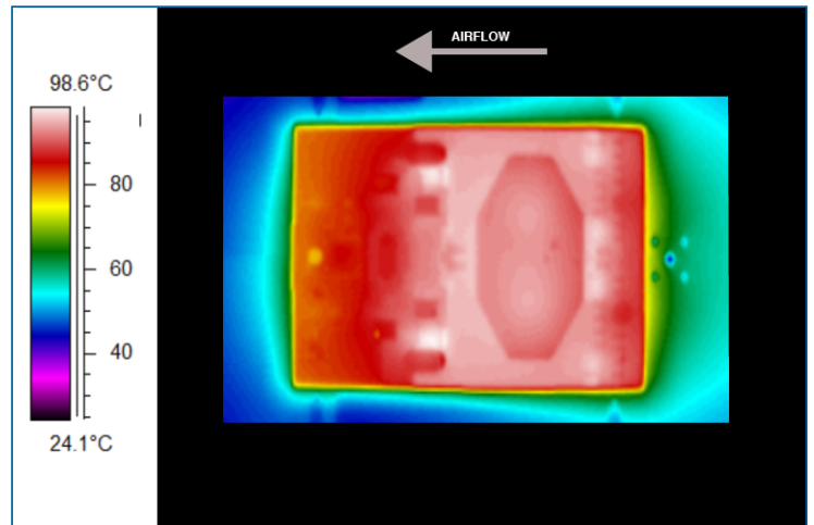
Figure 27 — Thermal plot, 400 LFM, 25°C, 48 Vin, 670 W output power
