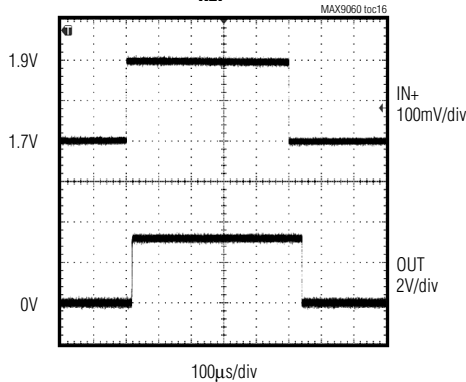
MAX9060 PROPAGATION DELAY AT V_{REF} = 1.8V
