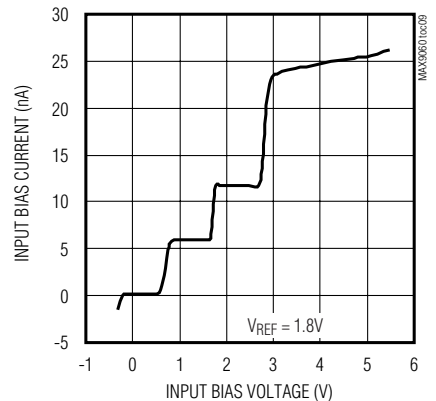
MAX9060 INPUT BIAS CURRENT vs. INPUT BIAS VOLTAGE
