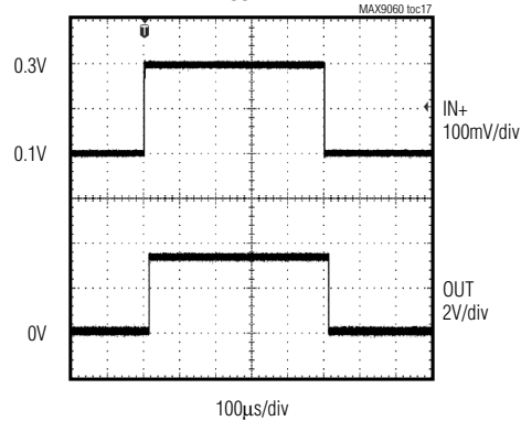
MAX9064 PROPAGATION DELAY AT V_{CC} = 3.3V
